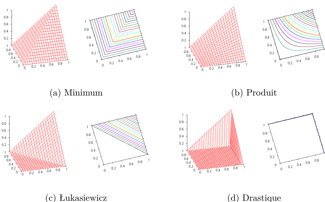
FIGURE 1.17 – T-normes usuelles
