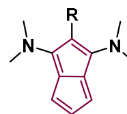
1,3-bis(dimethyl)aminopentalène
