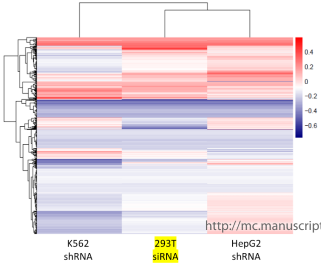
HNRNPA2B1
