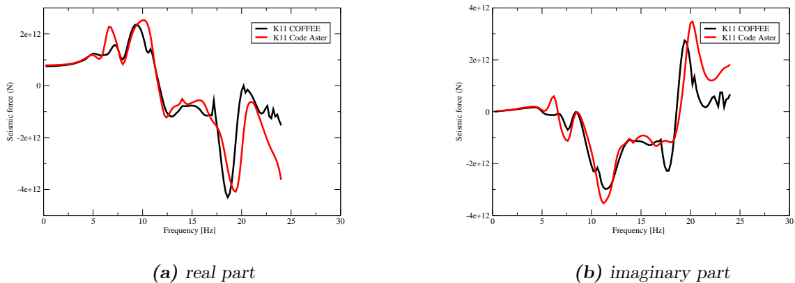
Figure 4.45.: Embedded cylindrical footing. Validation of the computation of the seismic force for the coupling of SV-wave with the horizontal mode f_{11} : comparison between the FM-BEM (denoted COFFEE) and the FEM-BEM coupling (Code_Aster) solutions.
