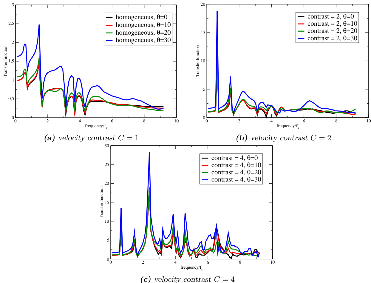
Figure 5.11.: Total displacement at the base of the structure. An incident unit plane SV-wave is imposed as a loading for various angle of incidence.
