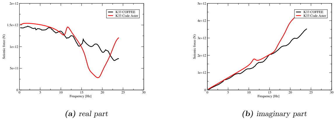
Figure 4.44.: Validation of the computation of the seismic force for the coupling of P-wave with the horizontal mode f_{33} : comparison between the FM-BEM solution (denoted COFFEE), the solution given by Code_Aster.
