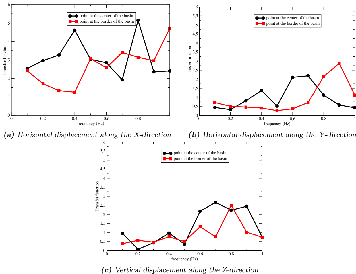
Figure 6.3.: Displacement at the free surface of the basin. A vertical incident unit plane SV-wave is imposed as a loading.
