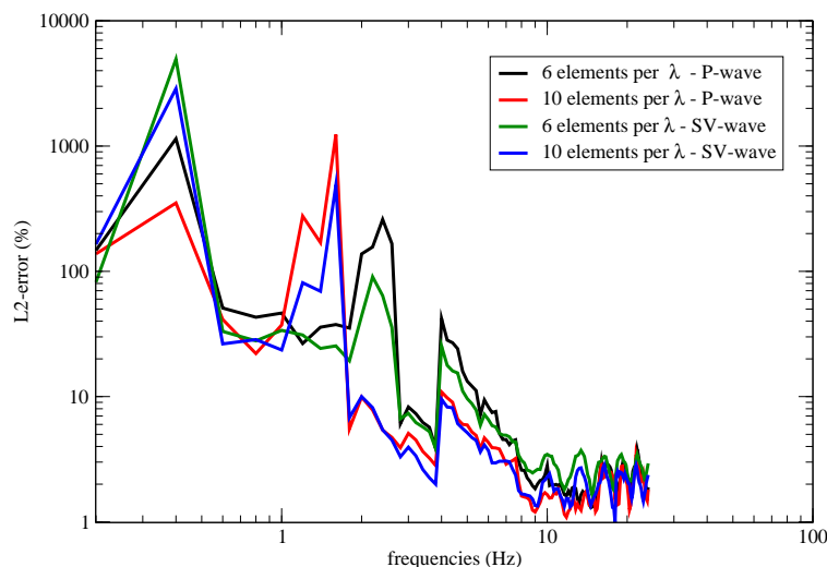
Figure 2.4.: Relative errors for different meshing criterion.
