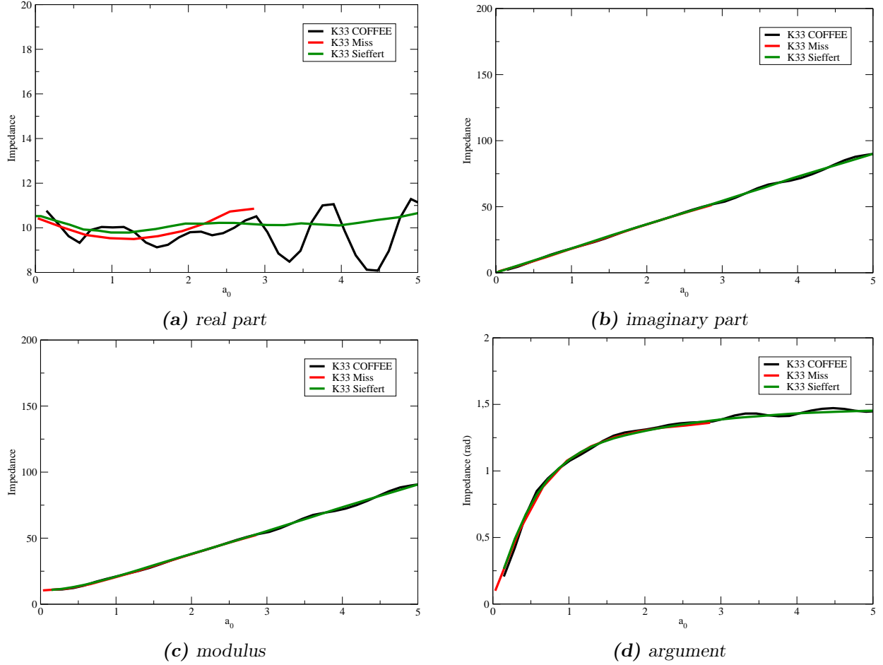
Figure 4.13.: Embedded cylindrical footing: Validation of the computation of the impedance of the vertical mode K_{33} (Equation 3.7): comparison between the FM-BEM solution (denoted COFFEE ), the solution given by standard BEM using Miss3D code (denoted Miss ) and the solution extracted from [60] (denoted Sieffert ).
