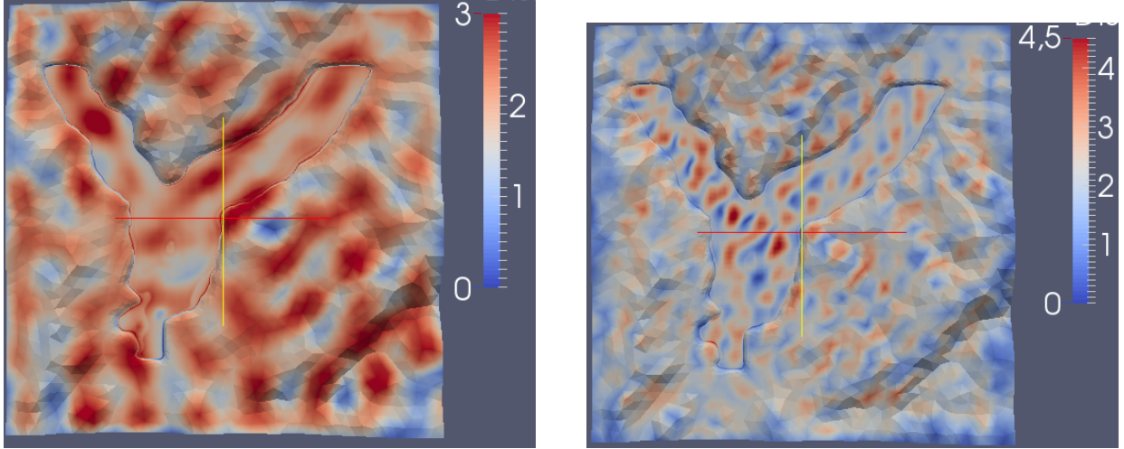
(a) Grenoble basin harmonic response to a unit incident wave at frequency f = 0,2\text{Hz} .
