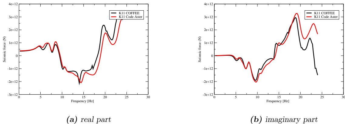
Figure 4.41.: Validation of the computation of the seismic force for the coupling of SV-wave with the horizontal mode f_{11} : comparison between the FM-BEM solution (denoted COFFEE) and the solution given by the FEM-BEM coupling ( Code_Aster ).
