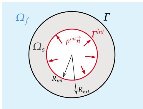
Figure 3.4: Radially-symmetric pressurised elastic annulus in an acoustic fluid.
