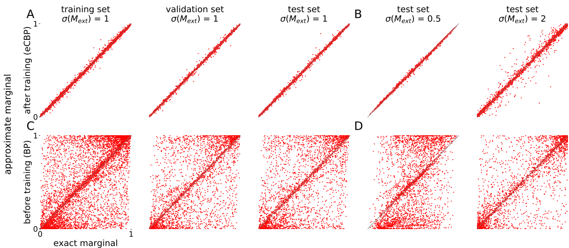
FIGURE 3.8: Extended Circular BP generalizes to new data after training . The topology considered here is the Erdos-Renyi model with p = 0.6 and 9 nodes, with 30 random weighted graphs generated, each with 100 test examples. (A) The model learns and generalizes well to the test set (within-set generalization). (B) Generalization to examples with different statistics (out-of-set generalization). While \sigma(\mathbf{M}_{\text{ext}}) = 1 on the training set, the model still performs well for lower and higher standard deviations of the input. The performance goes down for increased \sigma(\mathbf{M}_{\text{ext}}) as expected (the system becomes highly non-linear, and the correction brought by eCBP is linear) but only slightly. Inferences remain relatively good on such examples for instance compared to BP. (C, D) Same as above but for BP, which shows frustration in (at least) some of the randomly weighted graphs, that is, absence of convergence of the algorithm, in which case the beliefs have very little to do with the correct marginals.
