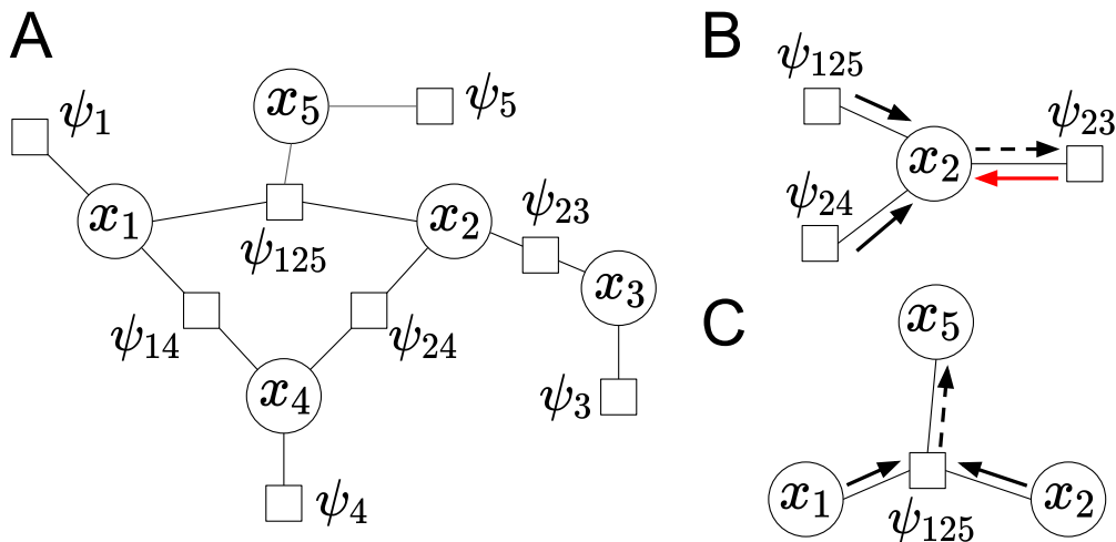
FIGURE 5.1: Belief Propagation and Circular Belief Propagation on a general factor graph. (A) Example of a factor graph with higher-order interactions (i.e., not only unitary and pairwise factors), here representing the probability distribution p(\mathbf{x}) = \psi_{125}(x_1, x_2, x_5)\psi_{23}(x_2, x_3)\psi_{14}(x_1, x_4)\psi_{24}(x_2, x_4)\psi_1(x_1)\psi_3(x_3)\psi_4(x_4)\psi_5(x_5) . (B) Belief Propagation updates a given variable-to-factor message (from x to \psi , dotted black line) according to the messages received by node x from other factor nodes than \psi (full black lines). For Circular BP, the opposite message (coming from \psi to x , full red line) is also taken into account. (C) Both BP and Circular BP update factor-to-variable messages (from \psi to x , dotted black line) according to the messages collected by \psi from other variable nodes than x (full black lines), and the interaction function \psi .
