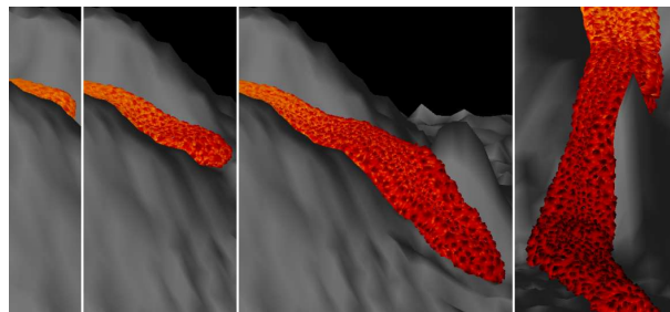
Figure 2.20: A’a lava flow in (SAC+99).
