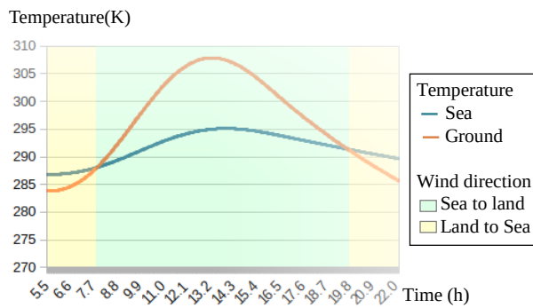
Figure 4.8: Diurnal cycles leading to a shift in wind direction at the interface between land and sea from onshore during the day to offshore at night.
