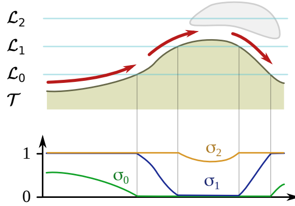
Figure 4.4: We use terrain topography \mathcal{T} to compute the orographic velocity damping coefficients \sigma_i per layer \mathcal{L}_i . Damping velocity creates high and low pressure areas that transform into updraft and downdraft velocity components, which accounts for orographic effects, such as the lenticular cloud depicted here.
