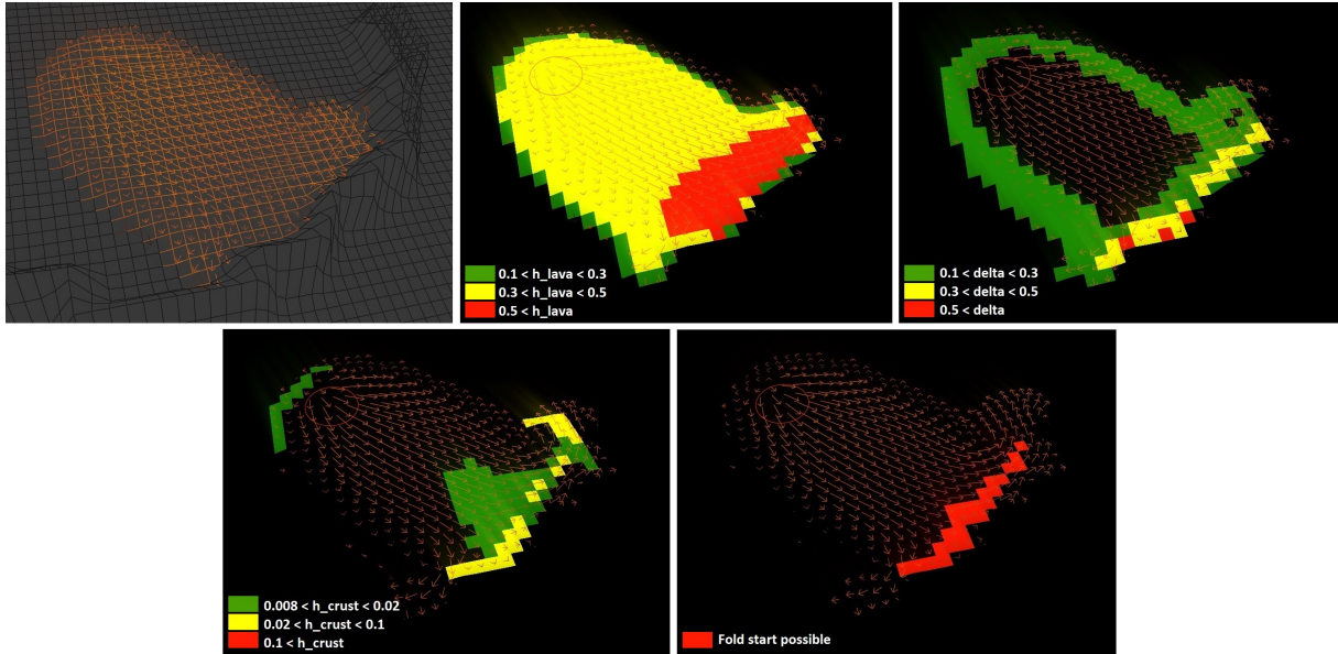
Figure 5.14: Real time visualization of several values on a lava flow for test case 1. The lava source is at the top left of the image, and the lava flows down the slope before hitting a long obstacle. Upper left: velocity field. Upper middle: lava thickness h_{lava} . Upper right: height difference between the lava and the lowest lava height around. Lower left: crust thickness h_{crust} . Lower right: fold start possibility.
