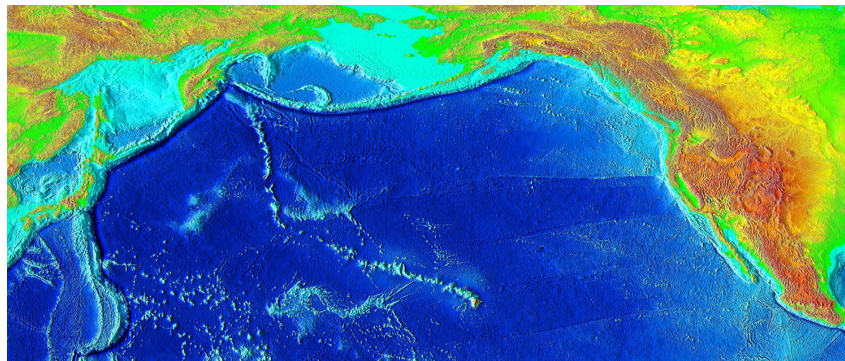
Figure 1.4: The trail formed by former and present volcanoes formed by the Hawaii hotspot while the Pacific tectonic plate was moving for millions of years. Only the most recent ones are high enough to form islands, the other ones are underwater. The most recent ones are also the only active volcanoes nowadays since the hotspot is underneath them.
