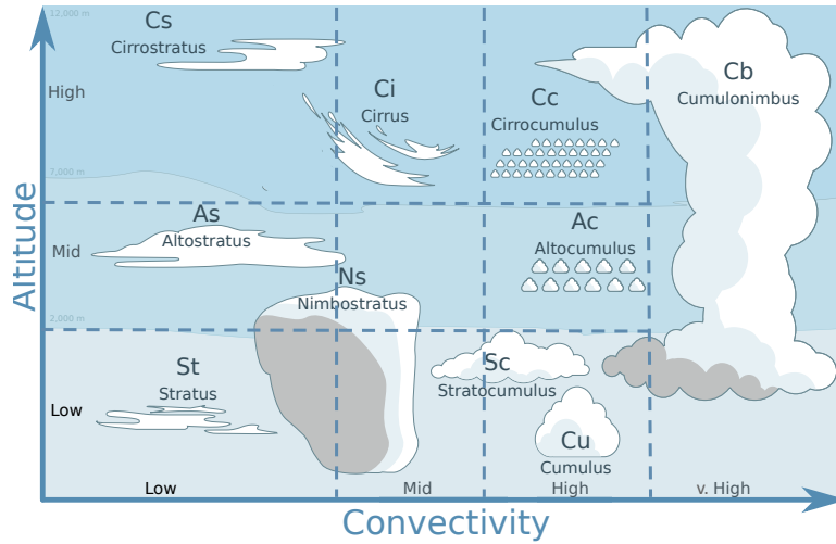
Figure 4.5: Our cloud classification scheme. The dashed lines indicate classification boundaries between cloudforms derived from Table 4.3.
