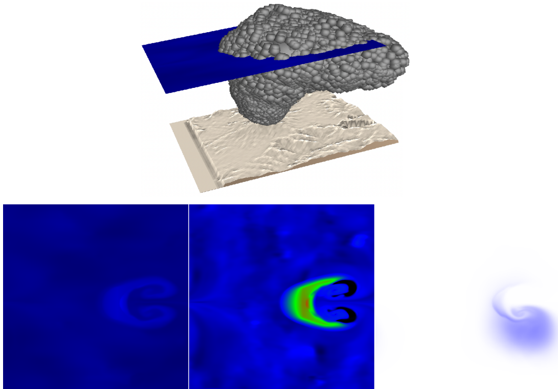
Figure 4.16: Top: A volcanic plume encountering an air layer at 16500m of altitude. Bottom: Corresponding maps of 30km by 30km showing condensed water (left), temperature (middle) and ash content (right) at 16500m after 250s of simulation.
