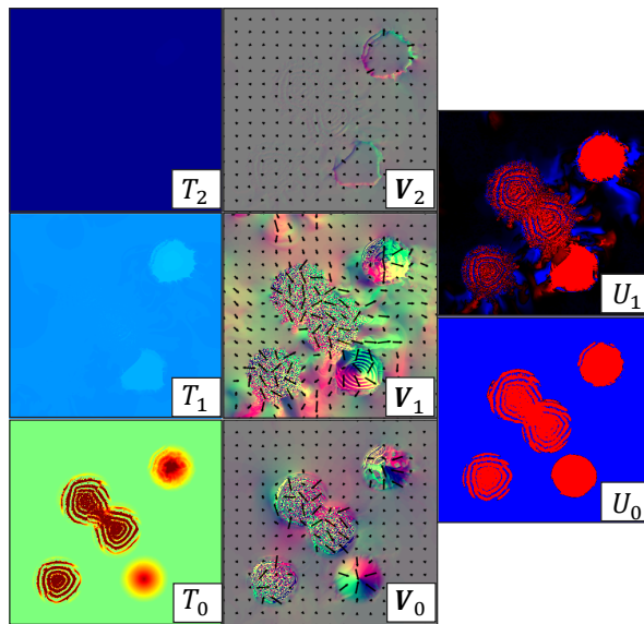
Figure 4.6: Convection cells form in a 3-layer simulation after the user paints hot-spots in the lowest temperature field. From left to right: temperature, 2D velocity visualized using both arrows and RGB colouring, and convection with a red (uplift) to blue (downdraft) heatmap. Successive layers appear from top to bottom with the convection field straddling layers.
