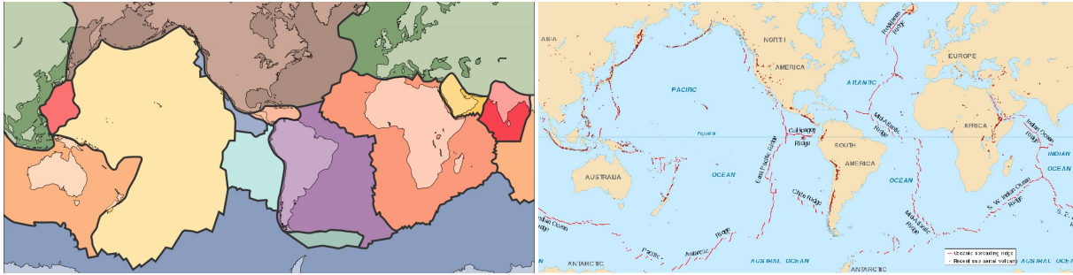
Figure 1.3: Left: Tectonic plates at the surface of the Earth. Right: Repartition of the volcanoes on Earth and spreading ridges. We can observe whole ranges of volcanoes where subduction occurs, as well as lonely volcanoes like Hawaii in the middle of the Pacific Ocean.
