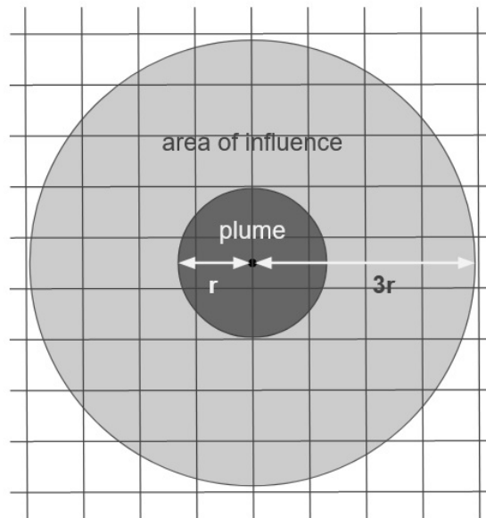
Figure 4.13: Region covered by the plume and its area of influence in the grid. We transfer data from the atmosphere to the plume system by computing the mean value in all cells in light grey. We transfer data from the plume to the weather system by enforcing values in the cells in dark grey.
