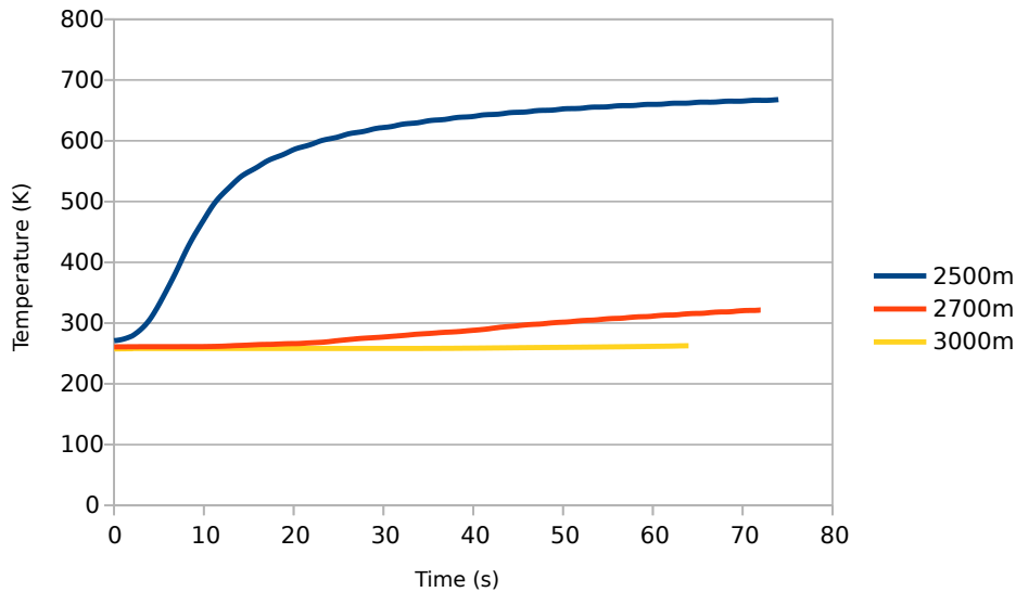
Figure 4.15: Smoothed curves showing the evolution of the temperature around the plume over time at altitudes of 2500m (where the vent is), 2700m, and 3000m.
