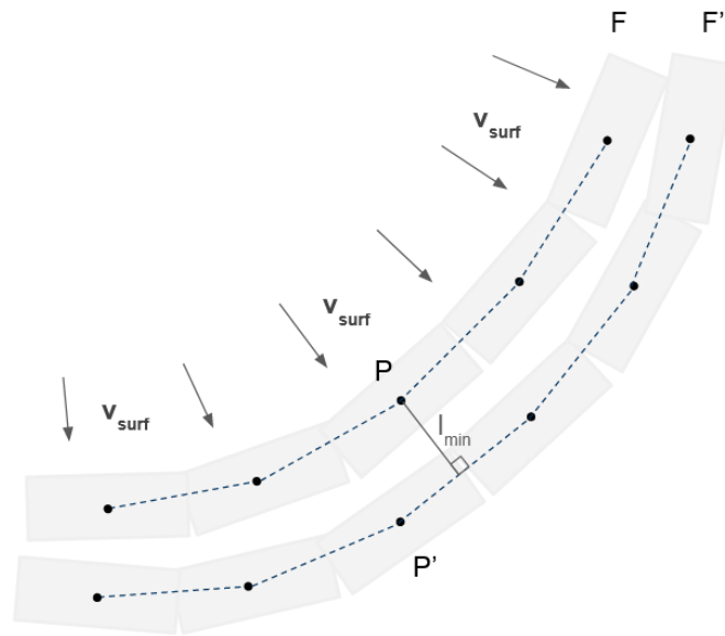
Figure 5.8: Collision detection between two neighbouring folds. Here, F is moving towards F' .
