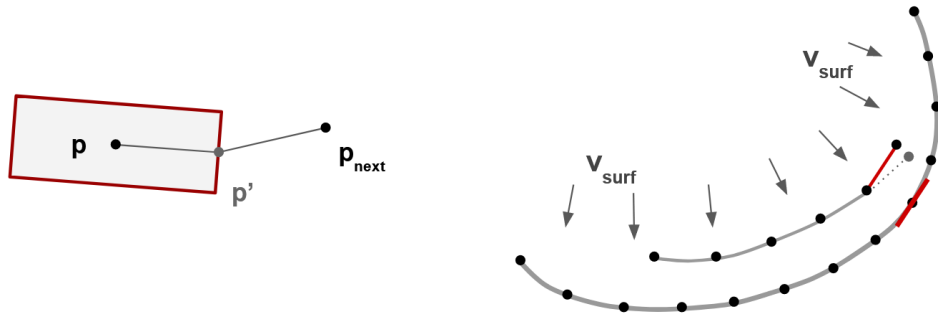
Figure 5.7: Iterative formation of a fold, particle after particle. Left: creation of the next particle in a fold in two steps (top view). Right: if this new particle is too close to a neighbouring fold, the fold tangent of the closest particle is used instead (top view).
