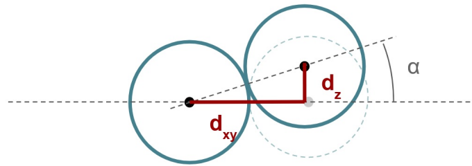
Figure 5.9: Ascending collision between two folds. The fold on the right is moving towards the one on the left. As the horizontal distance between the two particles becomes lower than the sum of their two radii, we compute the new height of the fold on the right to maintain the required distance. This gives us the angle defining its rotation.
