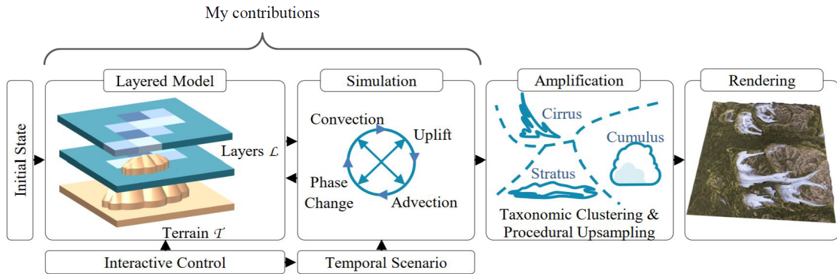
Figure 4.3: Overview: A large-scale layered atmospheric model is updated at interactive rates by a meteorological simulation. The later can be used to feed a fine-scale procedural volumetric amplification process, used for the offline rendering of animated skyscapes. I highlighted my contributions on this model: I worked on the terrain interaction and on the meteorological framework with Ulysse Vimont.
