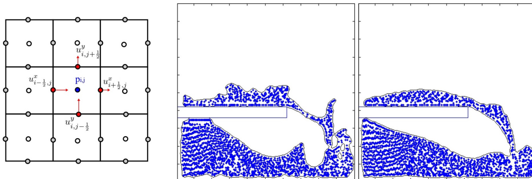
Figure 2.16: Left: The MAC grid. Middle: PIC simulation. Right: FLIP simulation.
