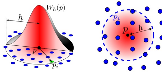
Figure 2.9: The kernel used in the SPH simulation. The further a particle is, the less it influences the density.
