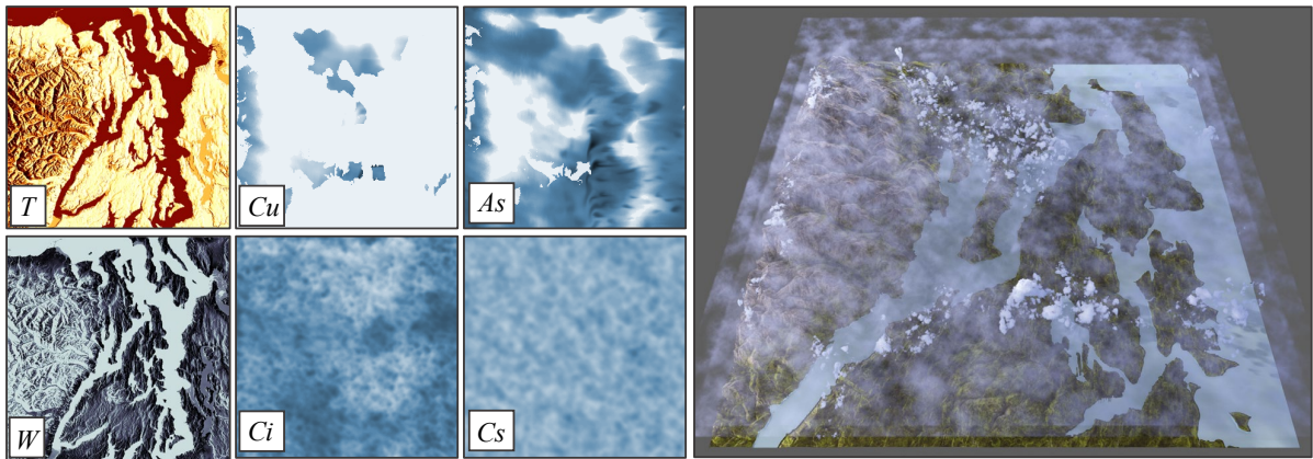
Figure 4.2: (Left) Our meso-scale simulation engine generates temperature ( T ) and water ( W ) terrain data, as well as cumulus ( Cu ), altostratus ( As ), cirrus ( Ci ) and cirrostratus ( Cs ) cloud layers. (Right) These sparse outputs are procedurally amplified to enable the rendering of a detailed volumetric skyscape.
