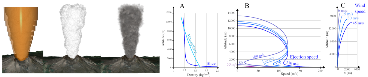
Figure 3.5: Left: Real-time previsualization of the column dynamics showing respectively the slices; the first and second scale spheres; rotating billboard. Right: Validation of the evolution of the simulation parameters. A: Evolution of the density of the column with respect to the altitude, compared to the density of the standard atmosphere (for a given ejection speed and no wind). B: Evolution of the altitude and vertical speed of a slice for different ejection speeds. C: Trajectory of a slice displayed in a 2D graph when a constant horizontal wind is applied. Stronger wind velocity leads to a lower maximal altitude.
