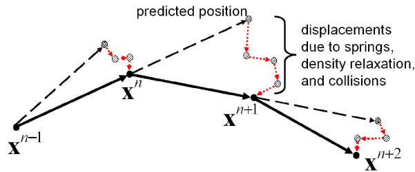
Figure 2.10: Computation of the next position for a particles in (CBP05).
