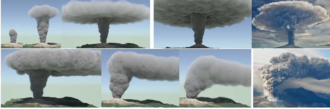
Figure 3.4: Top: Evolution of a rising plume through time and its spreading umbrella shape in the atmosphere (off-line rendering) compared to a real photograph at the right. Bottom: Effect of an increasing wind of 15, 45, and 105 m/s on the column profile (off-line rendering) compared to a real photograph.
