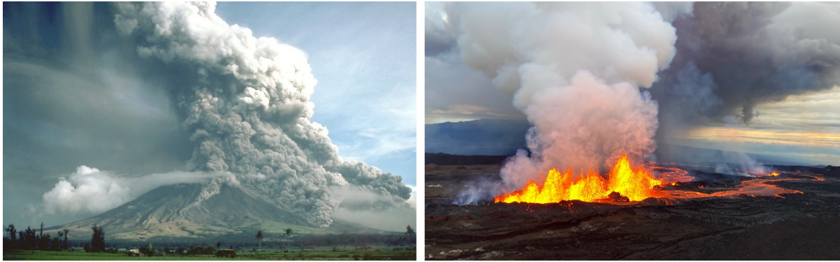
Figure 1.5: The two main types of volcanoes. On the left, a “grey” volcano, the Mayon in the Philippines, emitting a plume and pyroclastic flows. On the right, a “red” volcano, the Mauna Loa in Hawaii, emitting lava.
