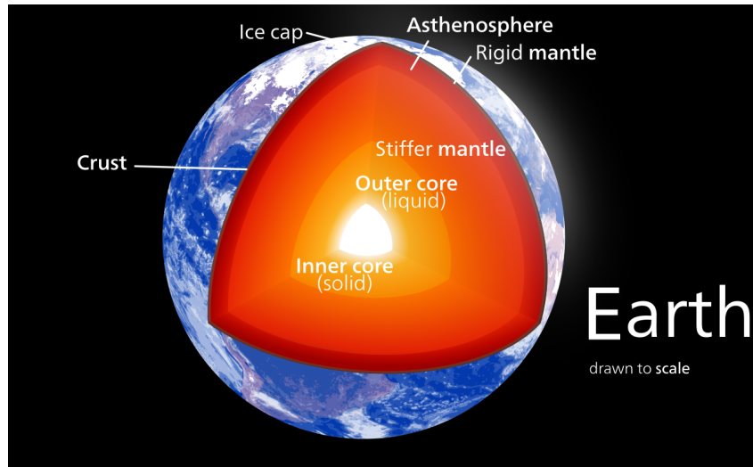
Figure 1.2: The different layers inside the Earth.
