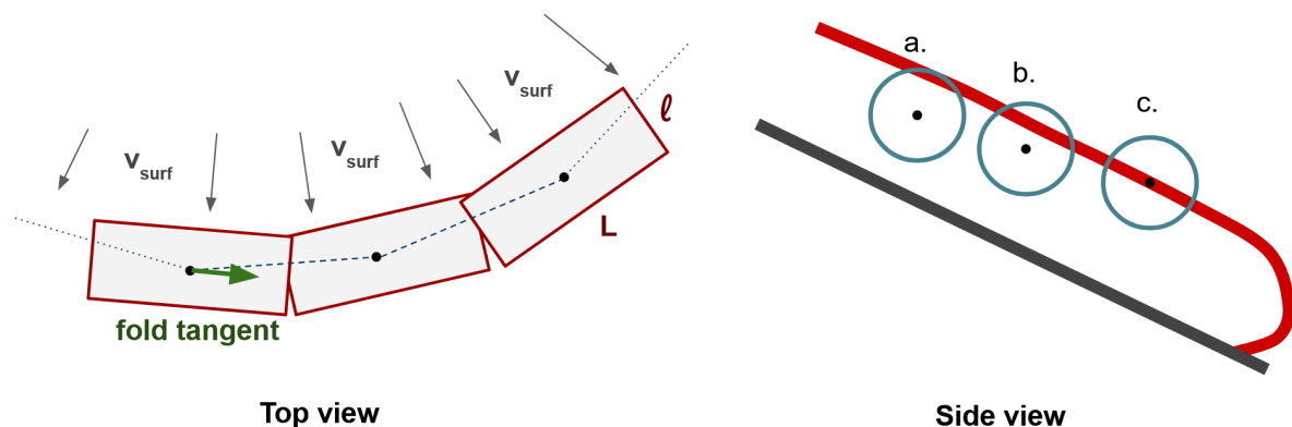
Figure 5.6: Left: Basic fold structure (top view). A fold is made of a chain of oriented particles physically represented by cylinders. L is the length of the cylinder and the distance between particles, and \ell its diameter. Right: Offset of a fold (side view). a. When the fold is created, it is first invisible under the surface, and the offset is set at -\frac{\ell}{2} . b. The offset increases over time. c. The offset eventually reaches zero, placing the fold at the surface of the flow.
