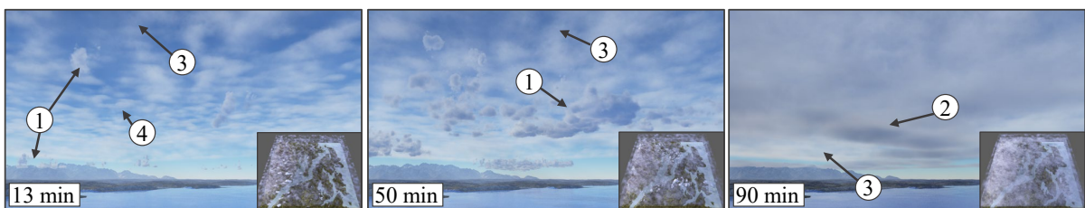
Figure 4.10: Multiple cloudforms within a single scene, including cumulus (1), altostratus (2), cirrus (3), and cirrostratus (4) clouds.
