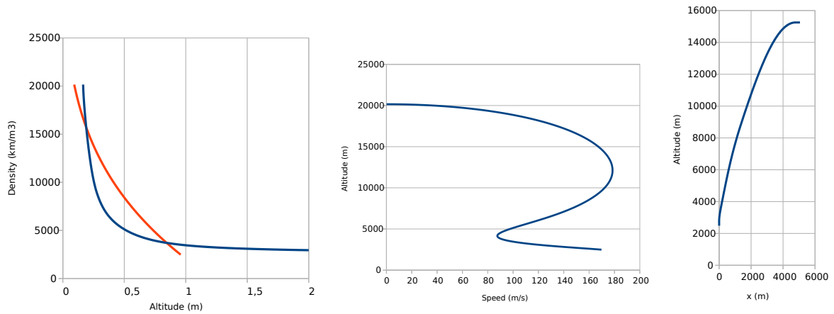
Figure 4.14: Left: Comparison between the density of a plume slice (blue curve) and the atmosphere (red curve) with altitude. Middle: Evolution of the vertical speed of the plume with altitude, with an initial speed of 170 m/s. Right: Trajectory of a plume under a wind originally set linear with a maximum of 50m/s at high altitude, and changing with time in the weather simulation.
