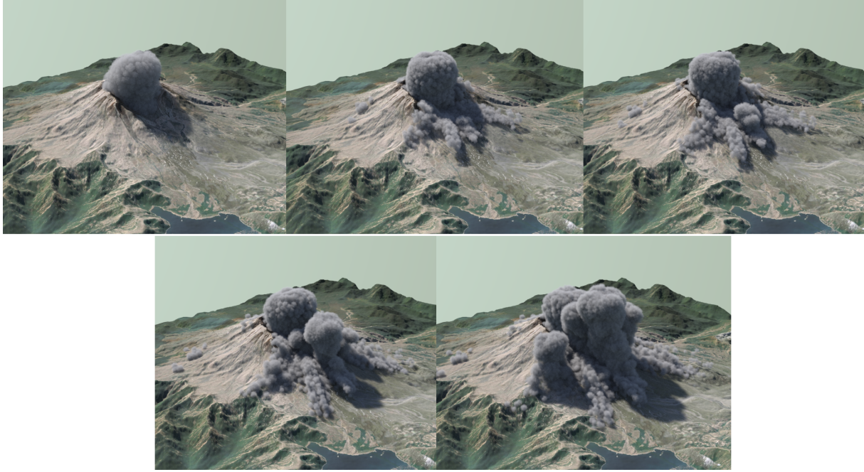
Figure 3.6: Pyroclastic flows animation: from left to right, first the top row and then the bottom row, the column begins to fall down; the pyroclastic flows go down the slopes of the volcano; secondary columns appear above the flows; secondary columns rise (off-line rendering).
