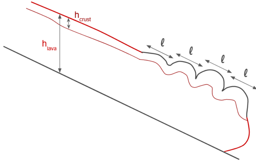
Figure 5.5: Side cut of a lava flow with a crust and folds.
