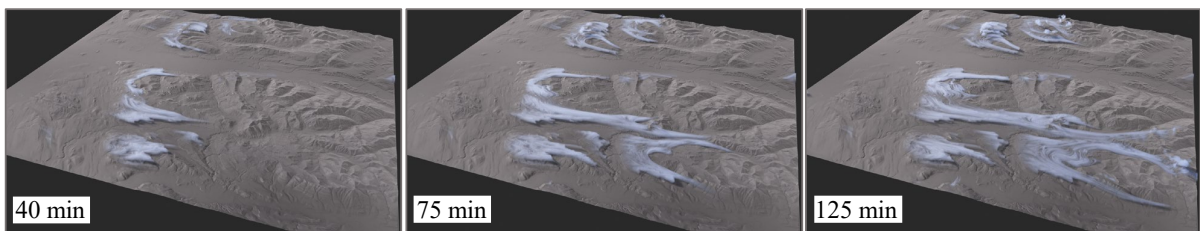
Figure 4.9: Orographic lift causes upslope cloud formation, showing one of the effects of terrain in our simulation framework.
