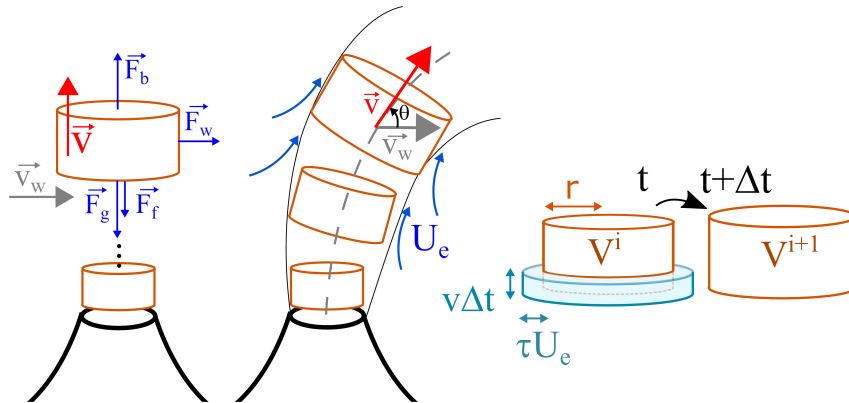
Figure 3.3: Left : Forces applied to a plume slice. Middle : Effect of wind on the path and orientation of slices. Right : Increase of slice volume at each time step, considering the entrained air represented by the blue ring.
