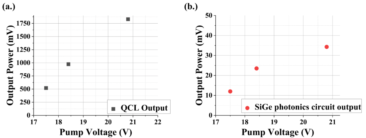
Fig.3.11. The output power in the function of the applied voltage for different configurations: (a.) from QCL output and (b.) from SiGe photonics circuit output.
