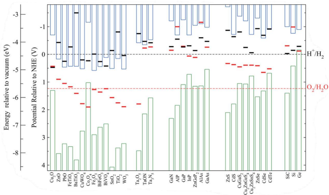
Figure 1. 13 Calculated anodic ( E_{p,d} red bars), cathodic ( E_{n,d} black bars) self-decomposition potentials for various semiconductor materials at pH=0, with corresponding CB and VB band alignments. Adapted from ref [51]
