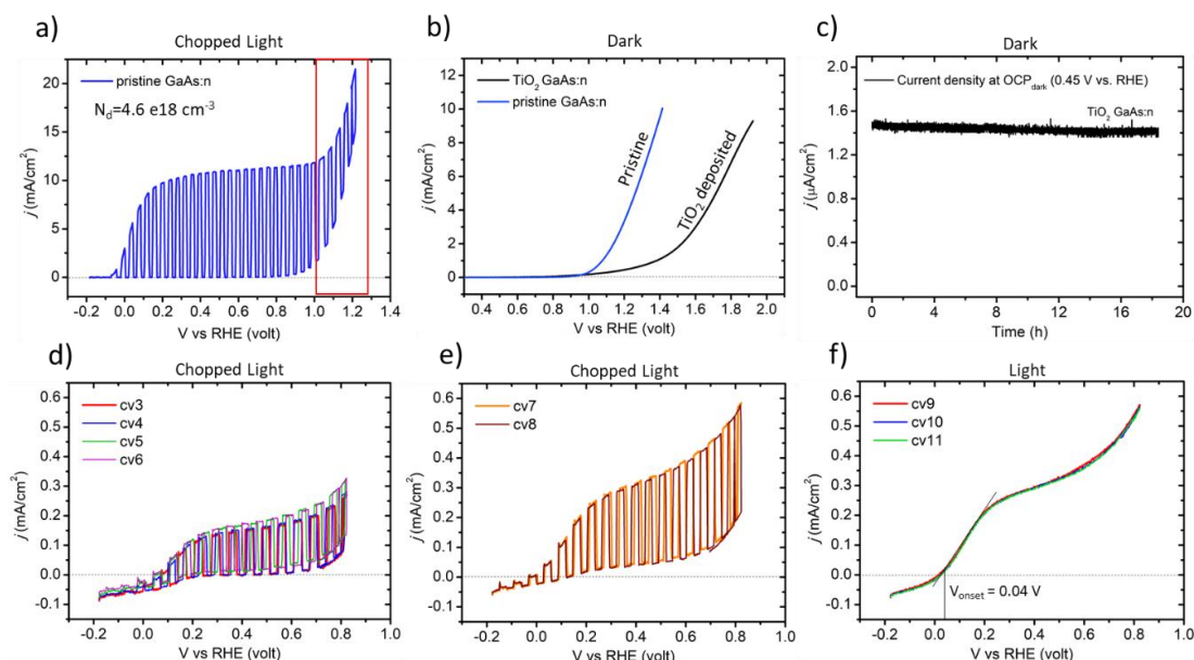
Figure 5. 21 Photoelectrochemical (PEC) characterization of the photoanodes: j - V curve of (a) pristine GaAs:n under chopped light; (b) j - V curve of \text{TiO}_2 GaAs:n and pristine GaAs:n PA in the dark ; (c) chronoamperometric stability test of \text{TiO}_2 GaAs:n PA at OCP in the dark; (d-e) j - V curves of \text{TiO}_2 GaAs:n PA under chopped light and (f) under light of 1-sun illumination
