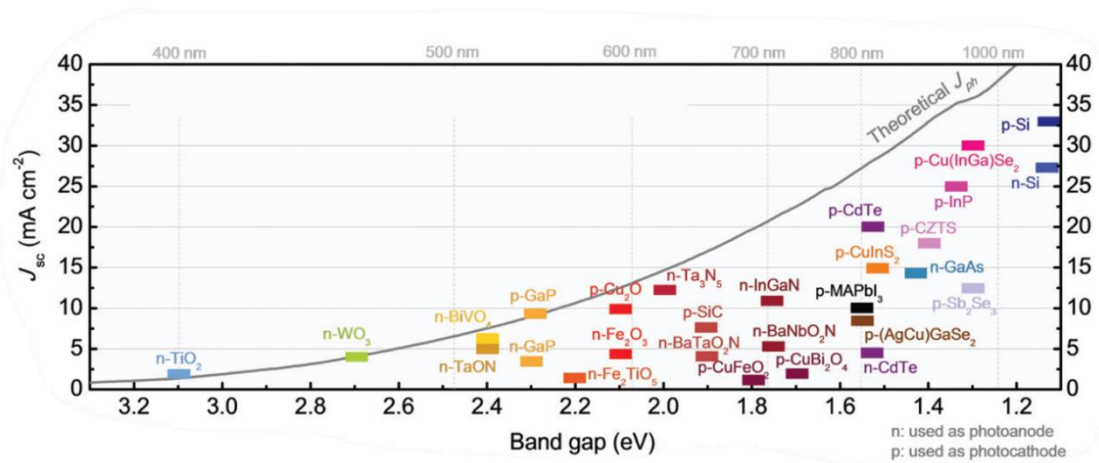
Figure 1. 10 Photocurrent density under short circuit conditions (photoanode @ 1.23 V vs. RHE, photocathode @ 0.0 V vs. RHE) under 1-sun illumination. Solid grey line is the j_{\text{theoretical}} and colored bars are experimental demonstrations with various different materials. Adapted from [30]
