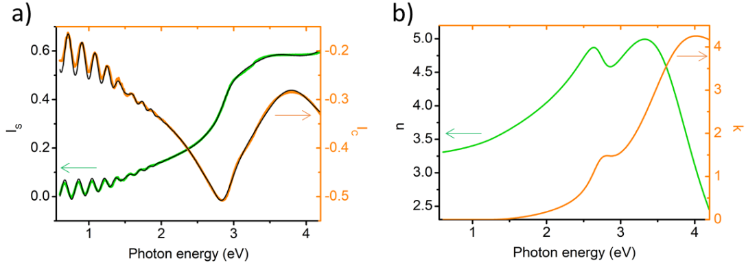
Figure 3. 3 (a) I_s (green) and I_c (orange) ellipsometry parameters and fitting curves with Tauc-Lorentz 2 model (black); (b) optical constants n (real part) and k (imaginary part) extracted from the fitting data for the GaAs/Si sample.
