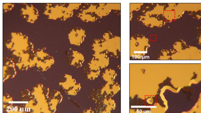
Figure 5. 15 Optical microscopy images of the CMP Ni/TiO 2 /GaAs-Si PA after 2 min of PEC characterization
