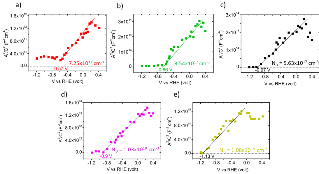
Figure 4. 8 Mott-Schottky analysis performed in the dark for \text{GaP}_{1-x}\text{As}_x alloys with different x(\text{As}) : (a) 1, (b) 0.83, (c) 0.52, (d) 0.22 and (e) 0, respectively. The x-intercept of the y-axis ( A^2/C_S C^2 ) of the linear portion indicate the flat-band potential ( V_{fb} )
