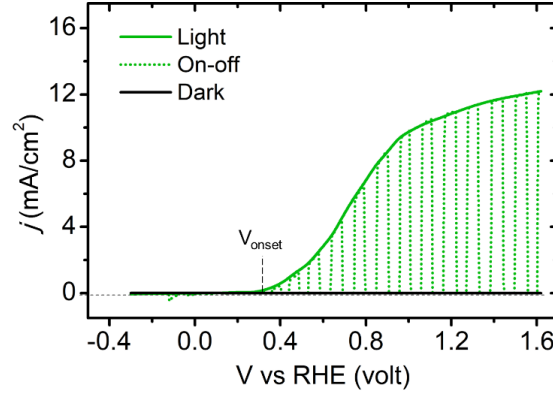
Figure 2. 11 Typical j - V curve for a photoanode of \text{GaP}_{1-x}\text{As}_x alloy with x(\text{As})=0.8 , measured in 0.2 \text{ M H}_2\text{SO}_4 ( \text{pH} = 0.35 ) under 1-sun illumination
