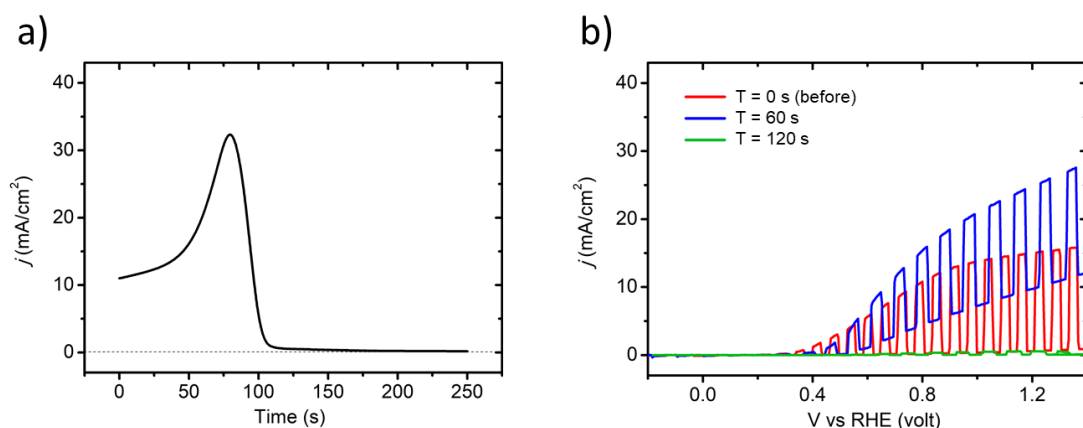
Figure 5. 4 (a) Photocurrent density vs. Time at 0.8 V vs. RHE under 1-sun illumination for 1- \mu m thick GaAs/Si:n photoanode; (b) j – V curves obtained before chronoamperometry (0 s), at 60 s and 120 s, respectively.
