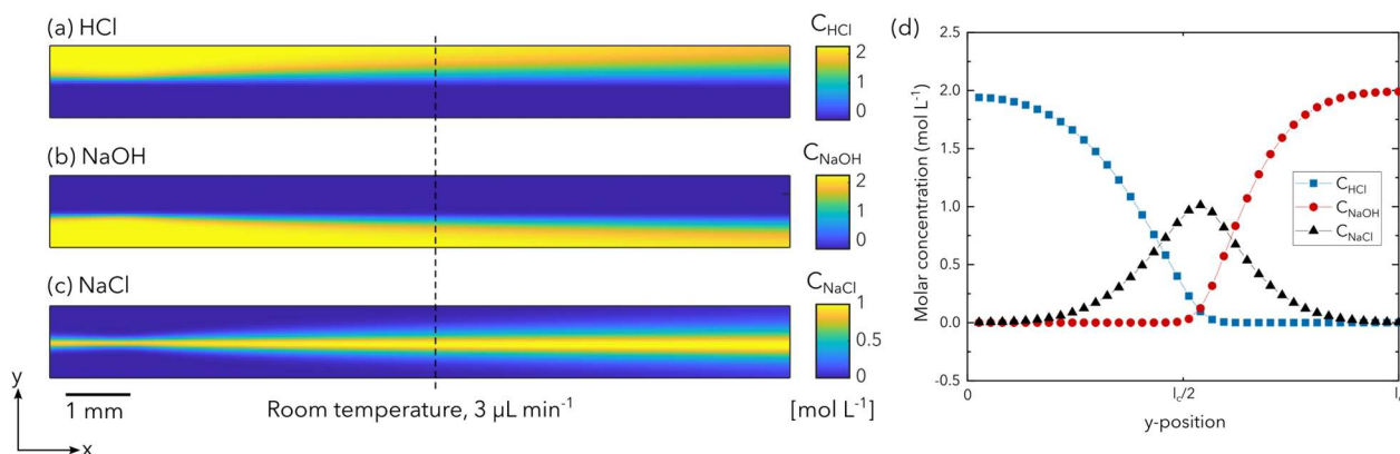
Fig. 3-7: The numerical concentration fields of (a) HCl, (b) NaOH, and (c) NaCl cropped to the entrance of the mixing channel at a flow rate of 3 \mu\text{L min}^{-1} and (d) the corresponding molar concentration profiles of each species averaged over 10 columns centered around the dashed line shown in (a) to (c).
