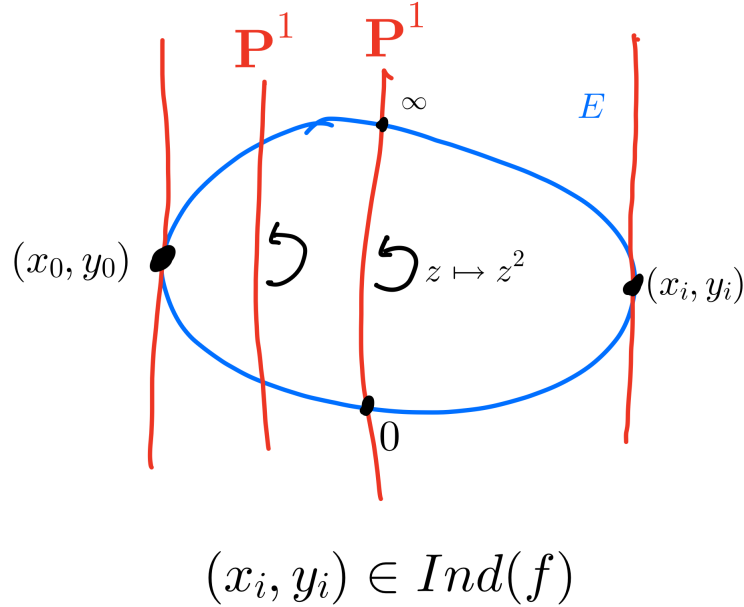
Figure 4.1: The endomorphism f on X_0
