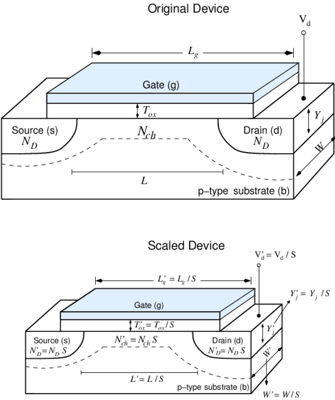
Figure 1.2 Architecture of an n-channel MOSFET and MOSFET constant electric field scaling by a factor of S [4].
