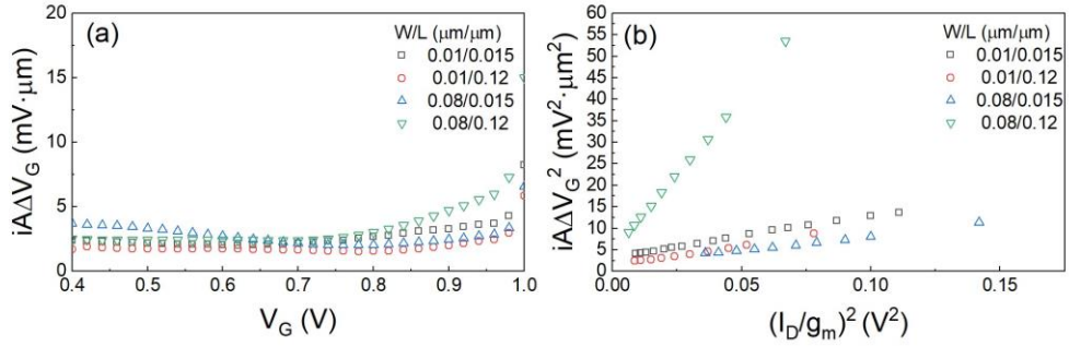
Figure 3.14 (a) the individual matching parameter, i\Delta V_G as a function of gate voltage, (b) Individual matching parameter vs. extracted by experimental data, (I_D/g_m)^2 with various device geometries.
