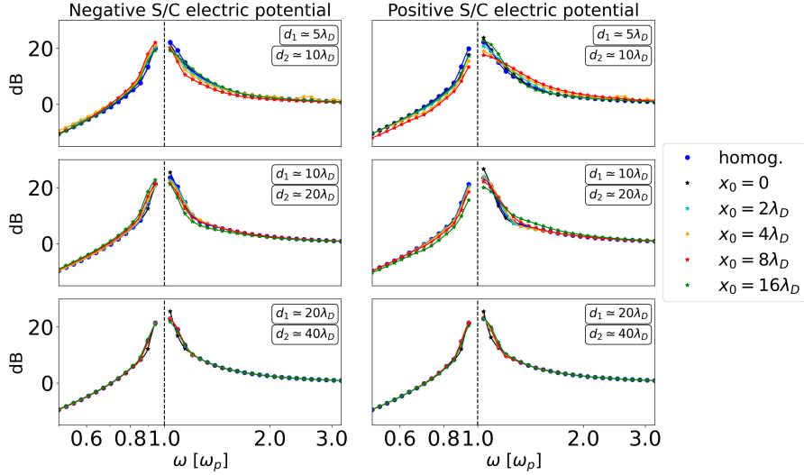
Figure 2. Examples of mutual impedance spectra obtained in the presence of the sensor/satellite plasma sheath. Left (resp. right) panels correspond to the plasma sheath of a satellite with negative (resp. positive) electric potential, placed at distance x_0 from the emitting antenna (Table 1).
