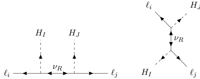
Figure 3.2: Matching contributions to the Weinberg operator in type I seesaw.
