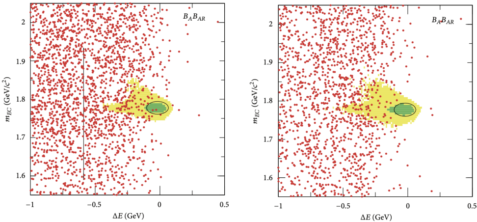
Figure 3.21: The Grand Signal Box and the 2\sigma ellipse for \tau^\pm \rightarrow e^\pm\gamma ( left ) and \tau^\pm \rightarrow \mu^\pm\gamma ( right ) decays in the m_{BC} vs. \Delta E plane. Data are shown as dots, and contours containing 90% (50%) of signal MC events are shown as light-shaded (dark-shaded) regions (Figure and caption from [243]).
