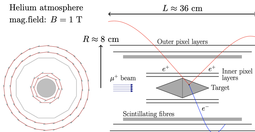
Figure 3.15: Schematic of the Mu3e experiment (Figure from [232]).
