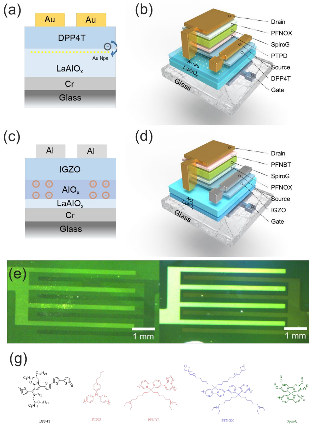
Figure 6-3. Side-view scheme of the low voltage (a) P-type and (c) N-type synaptic transistors. Three-dimensional scheme of the low voltage (b) P-type and (d) N-type LAOLETs. Optical image of low voltage (e) P-type and (f) N-type LAOLETs. (g) Chemical structures of DPP4T, PTPD, PFNBT, PFNOX and SpiroG.
