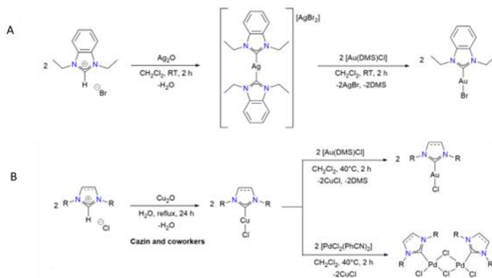
Scheme I-7: [A] Synthesis of [Ag(NHC)_2][AgBr_2] and transmetalation on gold center. 87 [B] Preparation of [Cu(NHC)Cl] complex and transmetalation on gold and palladium centers. 86
