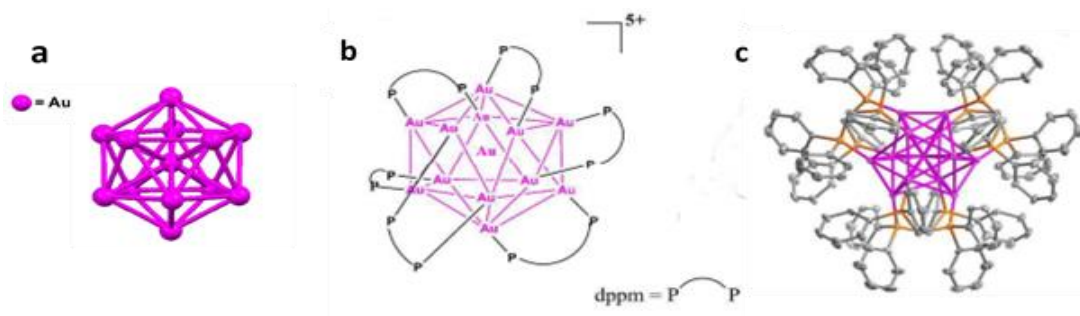
Figure I-4: Icosahedral Au_{13} of PPh_3 ( dppm = Ph_2PCH_2PPh_2 ) capped gold nanoclusters (view without ligands (a), schematic view with ligands (b), X-ray crystal structure (c)) 33,34,35
