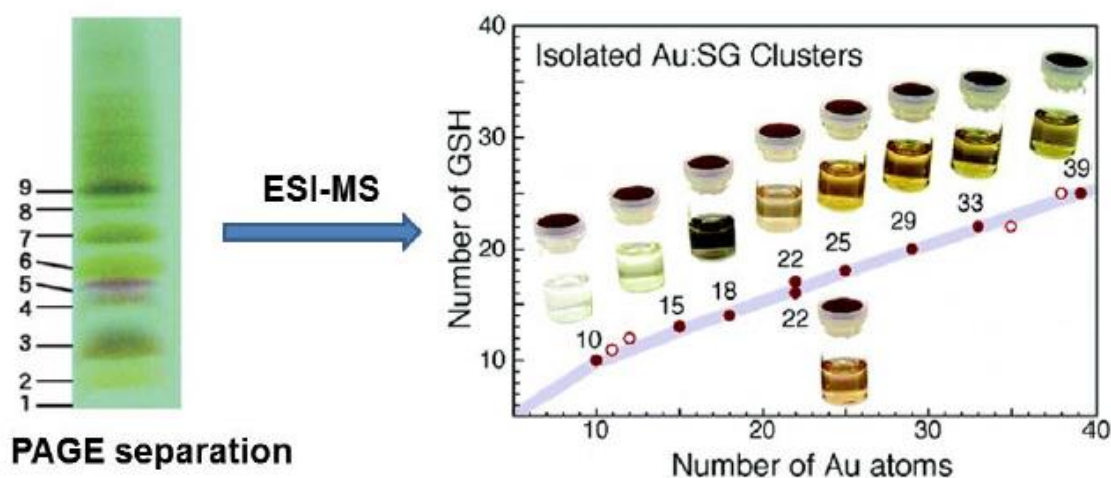
Figure I-9: Isolation and identification of atom-precise glutathionate protected gold nanoclusters through PAGE separation of Au_n(SG)_m nanoclusters mixture followed by ESI-MS analyses 41
