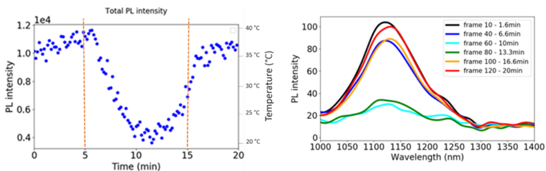
Figure V-20 Evolution of PL intensity as a function of time and temperature for silver sulfide NPs suspension synthesized from \text{AgNO}_3 , imid-PEG 4 , NaH and S in DCM (Ag 2 S-24). Red dotted line corresponds to switching on (5 min) and turning off (15 min) of the heating.
