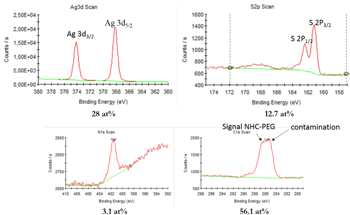
Figure V-26 Ag 3d, S 2p, C 1s, N 1s XPS spectra for the sample Ag_2S-d and elemental composition.
