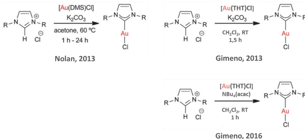
Scheme I-6 Synthesis of [Au(NHC)Cl] complex using the weak base route reported by Nolan in 2013 82 and Gimeno in 2013 83 and 2016 84
