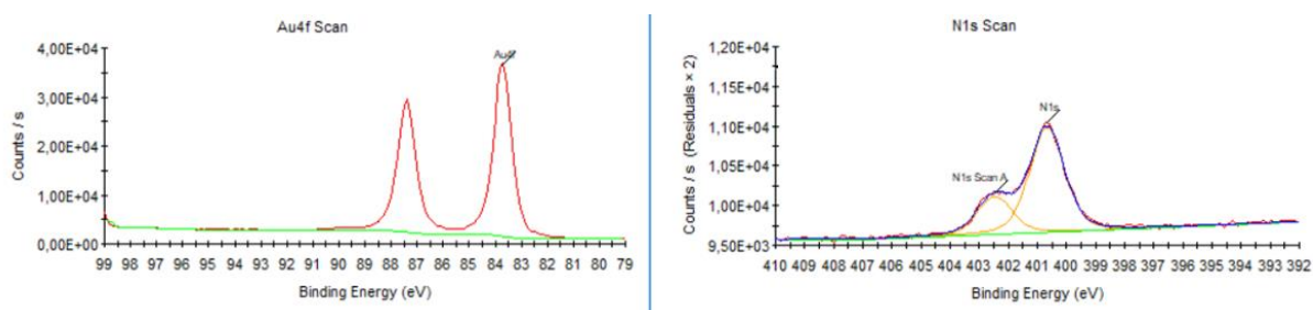
Figure IV-23 XPS N1s and Au4f spectra of nanoparticles synthesized from \text{HAuCl}_4 \cdot 3\text{H}_2\text{O} , 4 equiv. of \text{imidPEG}_4 , NaH and \text{NaBH}_4 in EtOH.
