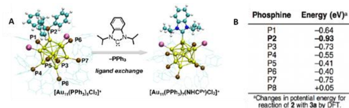
Figure I-15[A] Labelling of phosphines in [Au_{11}(PPh_3)_8Cl_2]Cl and position of NHC ligand exchanged on structure. [B] DFT-predicted changes in potential energy for reaction shown for each phosphine. 97
