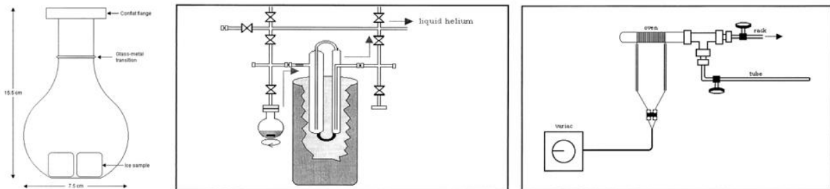
Figure 5.4: The first experimental setup of the getter method for Ar samples (Severinghaus et al., 2003). Left: vacuum extraction flask with ice samples. Middle: water trap at -100°C using water vapour as a carrier gas. Right: oven made by Zr/Al (SAES) getter in a quartz oven to absorb the N 2 , O 2 , and other reactive gases.
