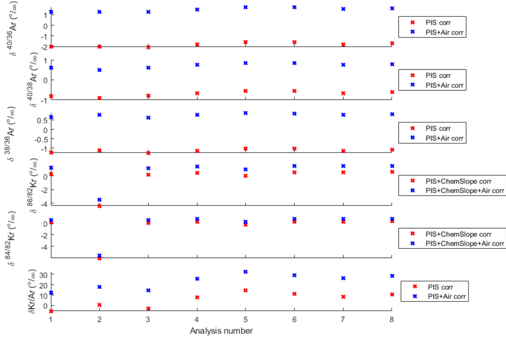
Figure 5.43: Comparison of \delta^{40/36}Ar , \delta^{40/38}Ar , \delta^{38/36}Ar and \delta Kr/Ar corrected for PIS (red crosses) and for PIS and outside air (blue crosses) on TALDICE ice samples. Comparison of \delta^{86/82}Kr and \delta^{84/82}Kr corrected for PIS and chemical slope and corrected for PIS, chemical slope and outside air analysis numbers corresponds to the progressive number of samples analysed over time.
