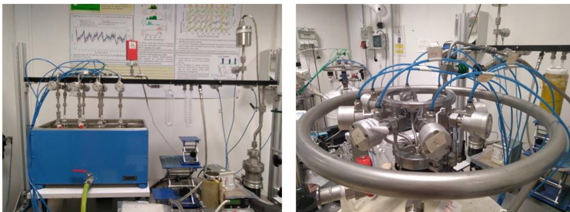
Figure 2.26: Left. Picture of the extraction line at LSCE. Right. Rosette in the helium tank connected to the extraction line.
