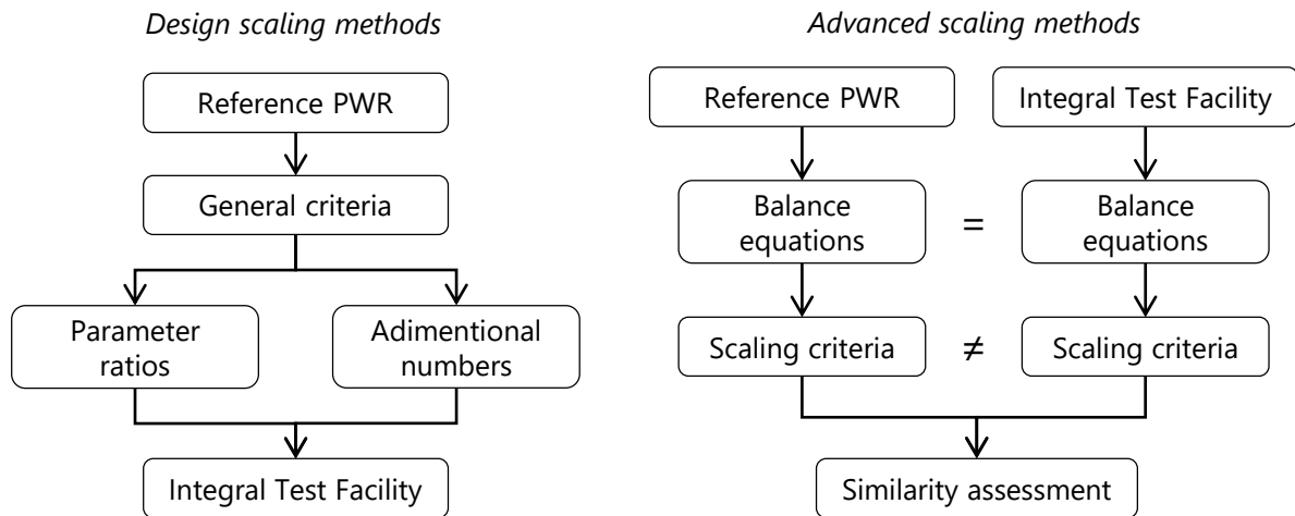
Figure 3.5: Comparison of design and advanced scaling methods
