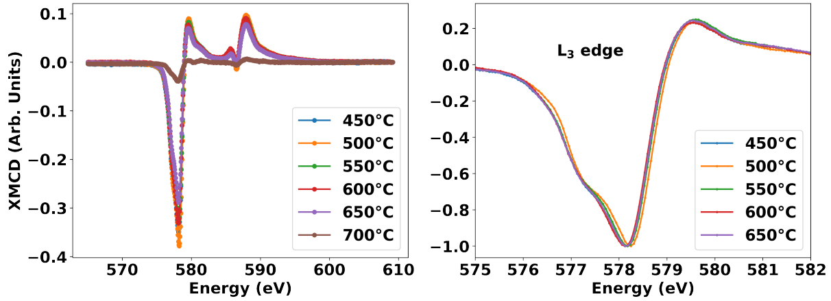
Figure 4.11: On the left, superposition of the XMCD signals of the samples as a function of T_A . Measurements are performed at 5 K with perpendicularly applied magnetic field of \pm 3 T. On the right, zoom on the L_3 edge after intensity normalization to -1 for spectroscopic comparison.
