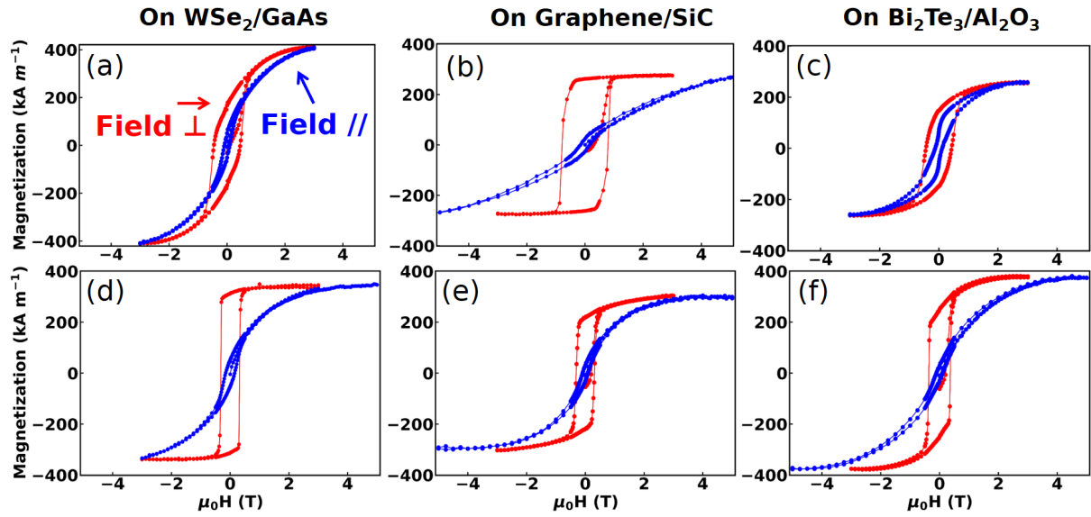
Figure 3.21: SQUID hysteresis loops with out-of-plane ( \perp ) and in-plane ( // ) applied magnetic field measured at 5 K are plotted after the removal of the substrate diamagnetic contribution. (a) (b) (c) Measurements on samples grown at 300°C on WSe 2 /GaAs, graphene/SiC, and Bi 2 Te 3 /Al 2 O 3 . (d) (e) (f) Same measurements on samples annealed at 400°C after growth.
