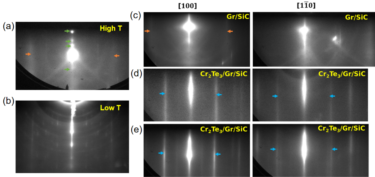
Figure 3.5: RHEED patterns of various \text{Cr}_2\text{Te}_3 films grown on Gr/SiC substrates. (a) Growth of nominally 10 layers at 600°C. Orange arrows indicate the diffraction rods of the underlying graphene, which is still not covered. Layers roughness is revealed with the dots on the specular highlighted by the green arrows. (b) Rings and spotty RHEED pattern after 30s of deposition at 150°C indicating the presence of Te 3D chains. (c) Gr/SiC substrates after desoxidation in-situ along two main crystal axes. (d) After the growth of 5 layers of \text{Cr}_2\text{Te}_3 at 300°C. Blue arrows reveal an isotropic crystal grain orientation. (e) After 10 min annealing at 400°C. The width of the peaks is reduced indicating lower defects density and larger grains.
