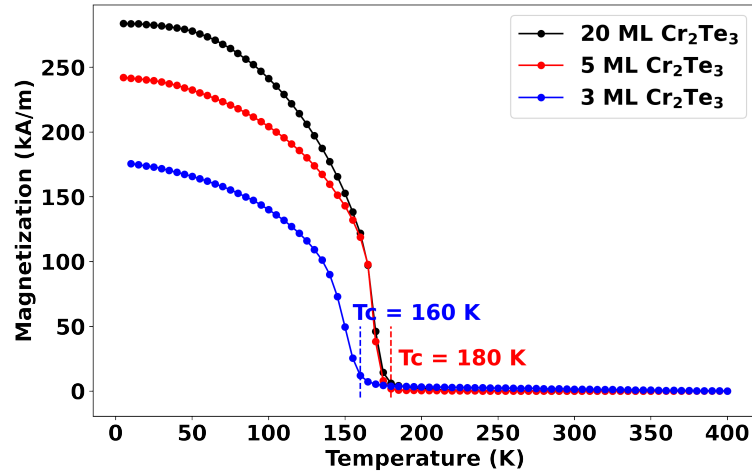
Figure 3.26: Remanent magnetization (after out-of-plane saturation) of Cr 2 Te 3 samples grown on graphene/SiC with different thicknesses. The measured T_C is indicated for each curve. The value is chosen at the inflexion point of the remanent curve.
