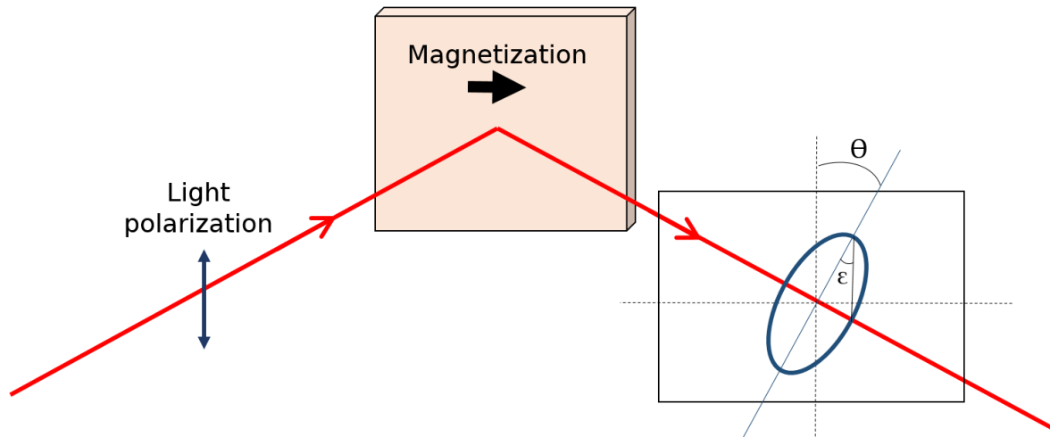
Figure 2.11: Schematic drawing of the polarization change of a linearly polarized light when reflected on a magnetic material. \theta and \epsilon respectively stand for the Kerr rotation and ellipticity.
