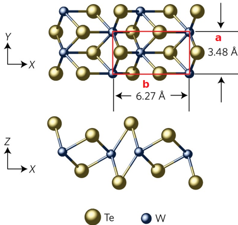
Figure 6.2: Crystal structure of 1\text{T}'\text{-WTe}_2 , adapted from [124]. The two in-plane lattice periodicities are indicated on the figure.
