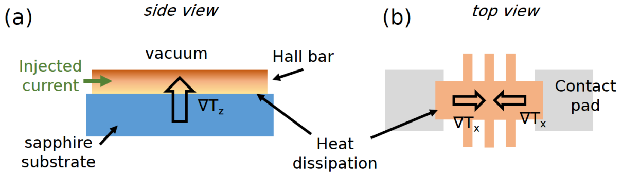
Figure 5.15: Schematic drawings of the patterned Hall bar to illustrate the origin of heat gradients. (a) Side view of the Hall bar and the substrate. The big arrow shows the vertical heat gradient. Heat dissipation is stronger at the interface with the substrate than with vacuum (or He in the sample space of the cryostat). (b) Top view, where the longitudinal heat gradients can be seen due to the heat dissipation in gold contact pads.
