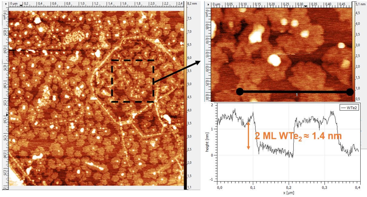
Figure 6.6: AFM images of WTe 2 layers deposited on graphene/SiC. The nominal thickness is 2 ML, as revealed by the line profile along the black line shown on the 500×500 nm scan.
