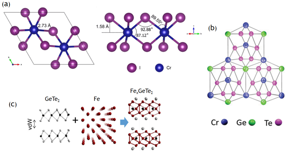
Figure 1.11: (a) Top view and side view of \text{CrI}_3 crystal, taken from [28]. (b) Top view of the structure of \text{CrGeTe}_3 , extracted from [29]. (c) The crystal structure of \text{Fe}_x\text{GeTe}_2 is the sum of the TMD \text{GeTe}_2 and a bcc Fe lattice (image adapted from [30]).
