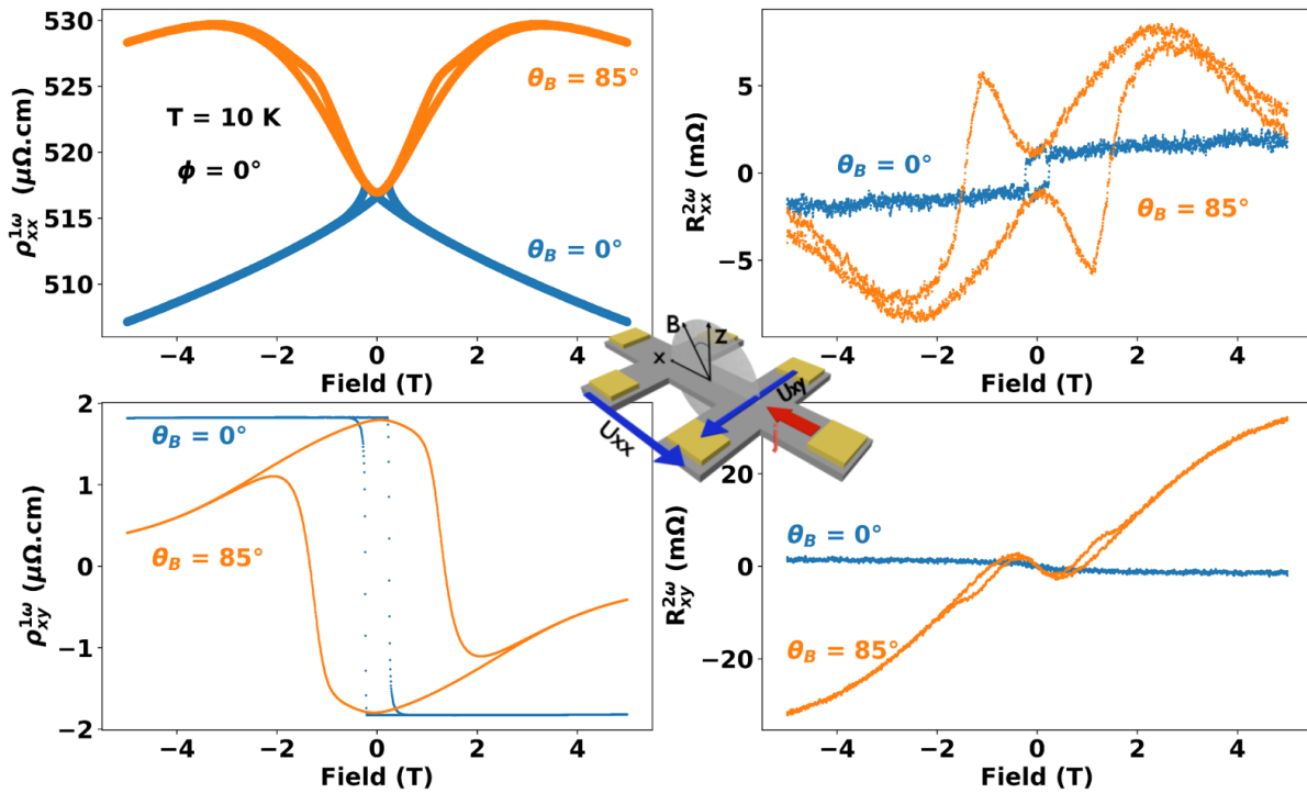
Figure 5.18: First and second harmonic measurements of 5 ML Cr 2 Te 3 deposited on Bi 2 Te 3 /Al 2 O 3 . Those curves were obtained at 10 K for two different directions of the magnetic field in the ZX plane (see the inset in the middle of the figure). OHE was subtracted from \rho_{xy}^{1\omega} . Second harmonic results are displayed without normalization by the surface and length of the Hall bar, in m \Omega .
