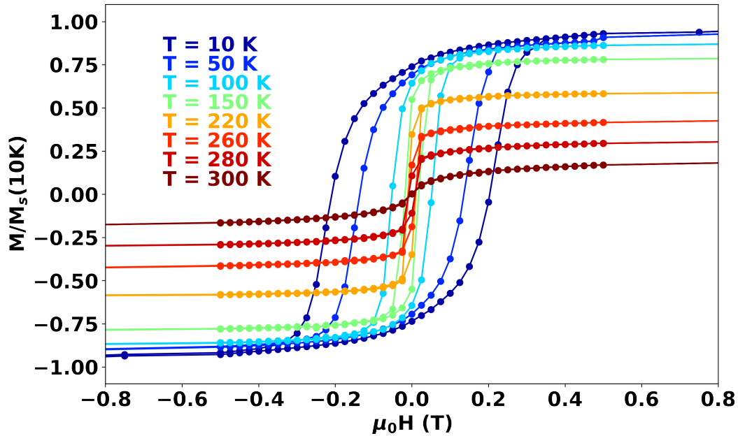
Figure 6.11: Hysteresis loops of \text{Cr}_2\text{Sn}_{0.4}\text{Te}_3 as a function of temperature. The magnetic field is applied in-plane. M_s(10\text{K}) was measured to be 443 kA/m.
