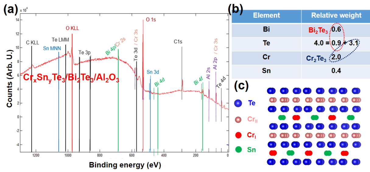
Figure 6.9: (a) XPS broadband spectrum of a heterostructure of \text{Cr}_x\text{Sn}_y\text{Te}_3/\text{Bi}_2\text{Te}_3 deposited on sapphire. C, Sn, Te, O, Bi, Cr and Al are evidenced in this sample. (b) Using the cross section of each element, a relative weight (in %) was attributed to each element. Te is split into two layers: one part in \text{Bi}_2\text{Te}_3 , as evidenced by the red dashed ellipse and one in \text{Cr}_x\text{Sn}_y\text{Te}_3 , as shown with the blue one. (c) Proposed crystal structure for \text{Cr}_2\text{Sn}_{0.4}\text{Te}_3 , based on \text{Cr}_2\text{Te}_3 . Sn atoms lie in the unoccupied sites of the Cr intercalated planes.
