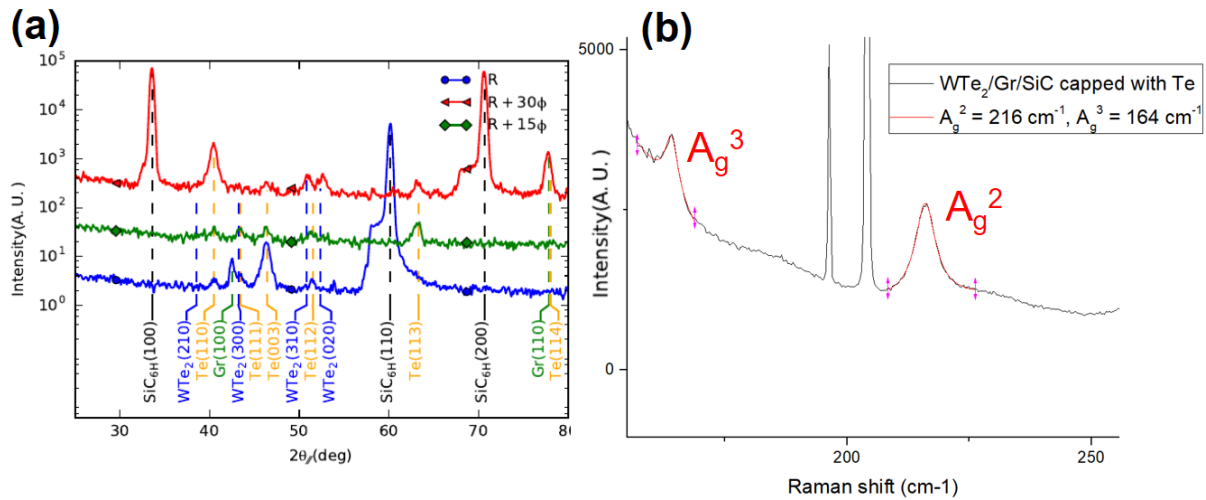
Figure 6.7: (a) XRD radial scan of 1 ML WTe 2 deposited on graphene/SiC. Measurements are performed along three azimuthal directions. Two of them are the graphene main crystal direction (R and R+30°) and one is 15° off for reference. (b) Raman spectroscopy of the same sample, revealing two characteristic vibrational modes of WTe 2 .
