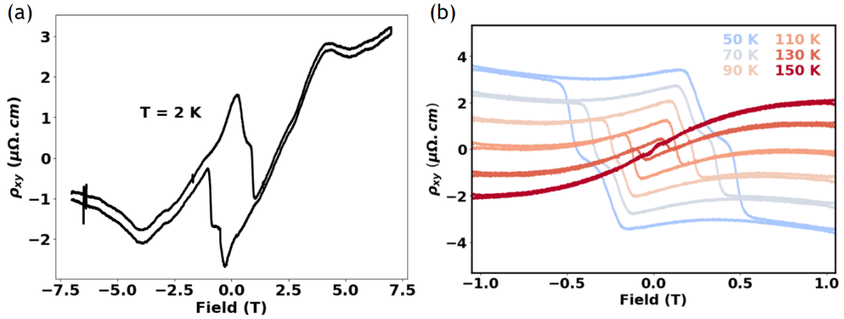
Figure 5.13: (a) Hall resistivity of 5 ML Cr 2 Te 3 on graphene/SiC measured at 2 K, without any treatment of the data. (b) Temperature dependent signal after subtraction of an arbitrary slope of 4 \mu\Omega\cdot\text{cm}/\text{T} for comparison with Fig. 5.7.
