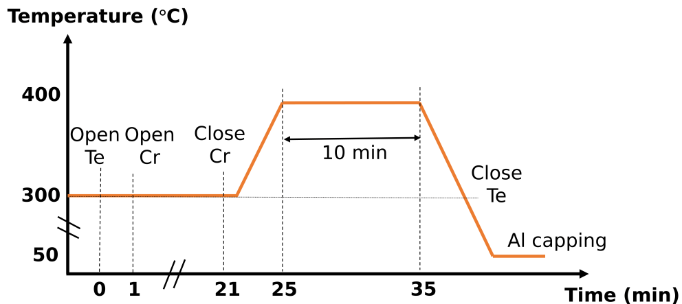
Figure 3.6: Sketch of the deposition procedure for 5 layers of \text{Cr}_2\text{Te}_3 . The growth temperature was 300°C and in situ annealing was performed at 400°C. An Al capping film of 3 nm was then deposited at 50°C.
