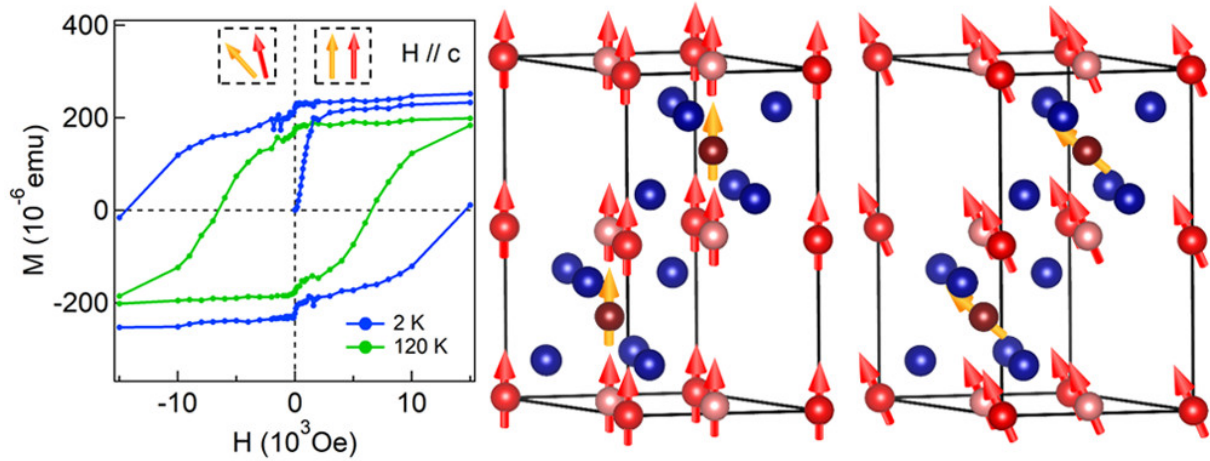
Figure 1.26: Canted spin structure of \text{Cr}_2\text{Te}_3 , taken from [47]. On the left, SQUID measurements of a thin \text{Cr}_2\text{Te}_3 film (8 nm thick). In the middle, an Ising spin model, and a canted one on the right. Cr atoms in the intercalated layers do not have the same canting angle as the one of Cr atoms in the fully occupied planes.
