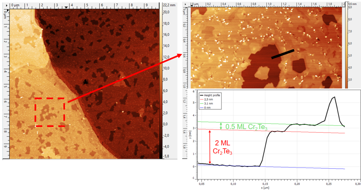
Figure 3.13: AFM images of 2 layers of Cr 2 Te 3 deposited on graphene/SiC. On the left, 10 × 10 \mu\text{m} scan centred around a step of the SiC substrate. The color scale height is defined on the right. The right image is a 2 × 2 \mu\text{m} zoom of the area in the red dashed square. A line profile is taken along the black line and shown in the graph below, with indication of heights relative to the graphene surface.
