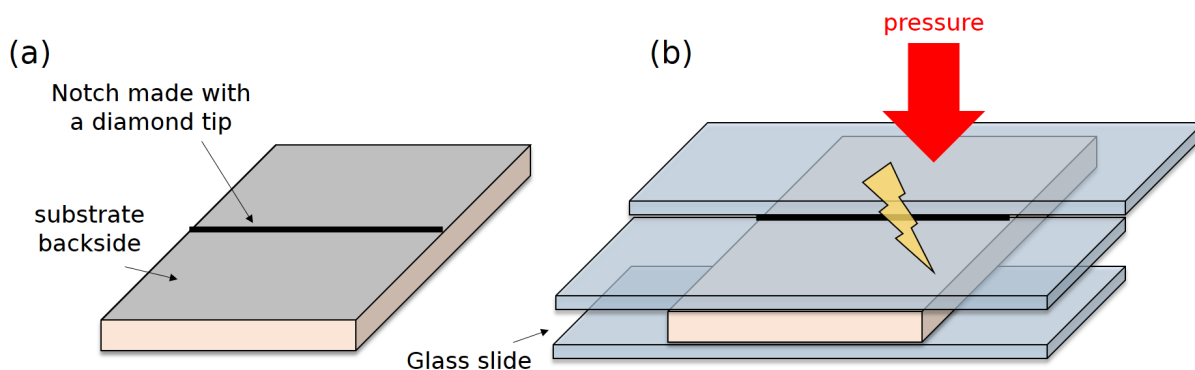
Figure 2.3: Schematic drawing of the steps to cleave a substrate. (a) We scratch the backside of the substrate using a diamond tip along the desired cleaving direction. (b) With the help of three glass slides, we put pressure to cleave along the notch, similarly to the method to separate squares of a chocolate bar.
