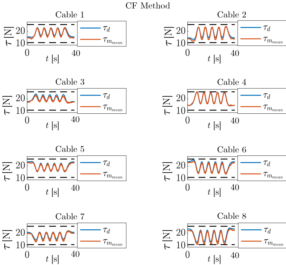
Figure I.2.21: ICF: desired and measured tension for each cable.
