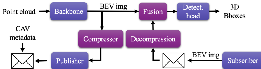
Figure 3.4 – Mid Collaboration framework. The ego vehicle fuses the BEV image of its point cloud with those broadcast by other agents to improve its performance.
