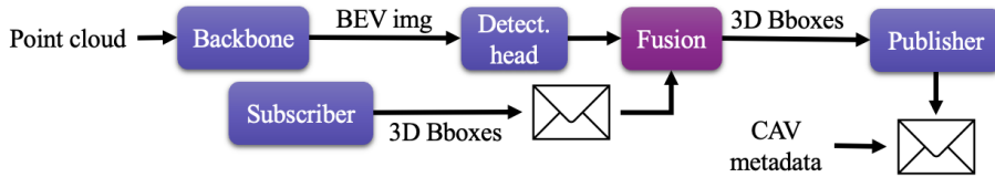
Figure 3.3 – Late Collaboration framework. Objects detected by other agents are fused with those detected by the ego vehicle to form its final output.
