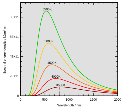
Figure 3.3: Illustration of the radiation density emitted by a black body at different temperatures. The wavelength of the radiation peak increases as the temperature decreases, i.e. wavelength is inversely proportional to the temperature. Image obtained from 4C , Wiens law , modified by Evelyn Gutierrez, CC BY-SA 3.0
