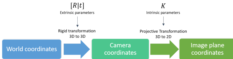
Figure 2.4: Projection of 3D points from the world frame into the image plane.
