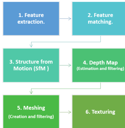
Figure 2.7: General 3D SfM reconstruction pipeline implemented in Meshroom, a well-known open source software for passive 3D reconstruction.
