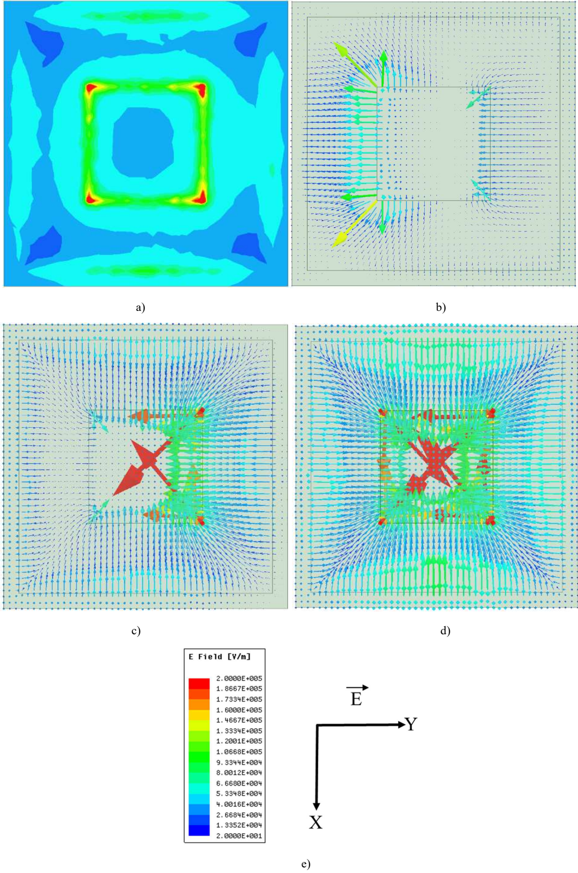
Fig.3.7 Electric field distribution of the unit cell under oblique incidence in TM case ( \phi_{inc}=90^\circ , \theta_{inc}=22.54^\circ , f=40\text{GHz} , h=5.2\text{mm} , L_r=1.5\text{mm} , with resonance). a) Complex magnitude. b) Time-varying field ( \omega t=0^\circ ). c) Time-varying field ( \omega t=45^\circ ). d) Time-varying field ( \omega t=90^\circ ). e) Scale
