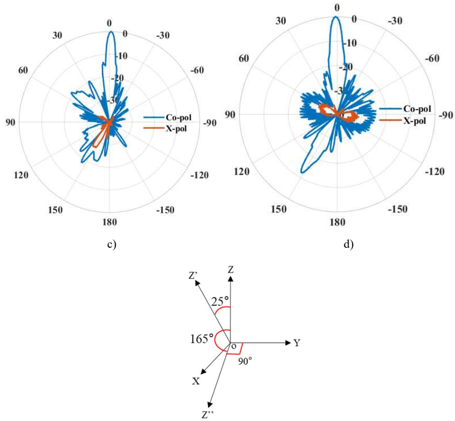
Fig.4.23 Normalized radiation patterns of TRA2 (dB) at 19 GHz - a) yoz plane (reflected beam). b) xoz' plane (reflected beam). c) yoz'' plane (transmitted beam). d) xoz'' plane (transmitted beam)
