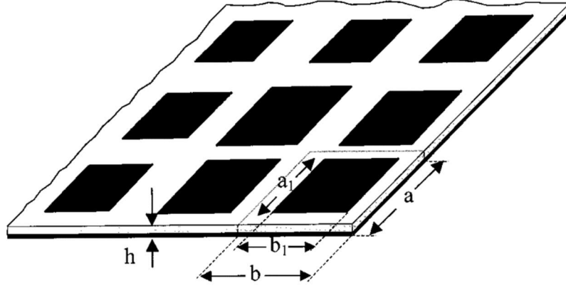
Fig.1.6 schematic models of reflectarray cells with variable size [39].
