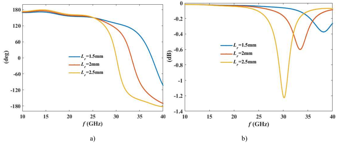
Fig.3.3 Frequency response of the unit cell ( h=5\text{mm} , normal incidence). a) Reflection phase. b) Magnitude.
