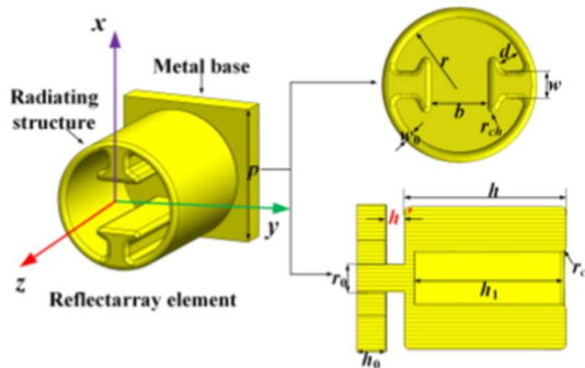
Fig.1.19 Geometry of the unit cell in [53].
