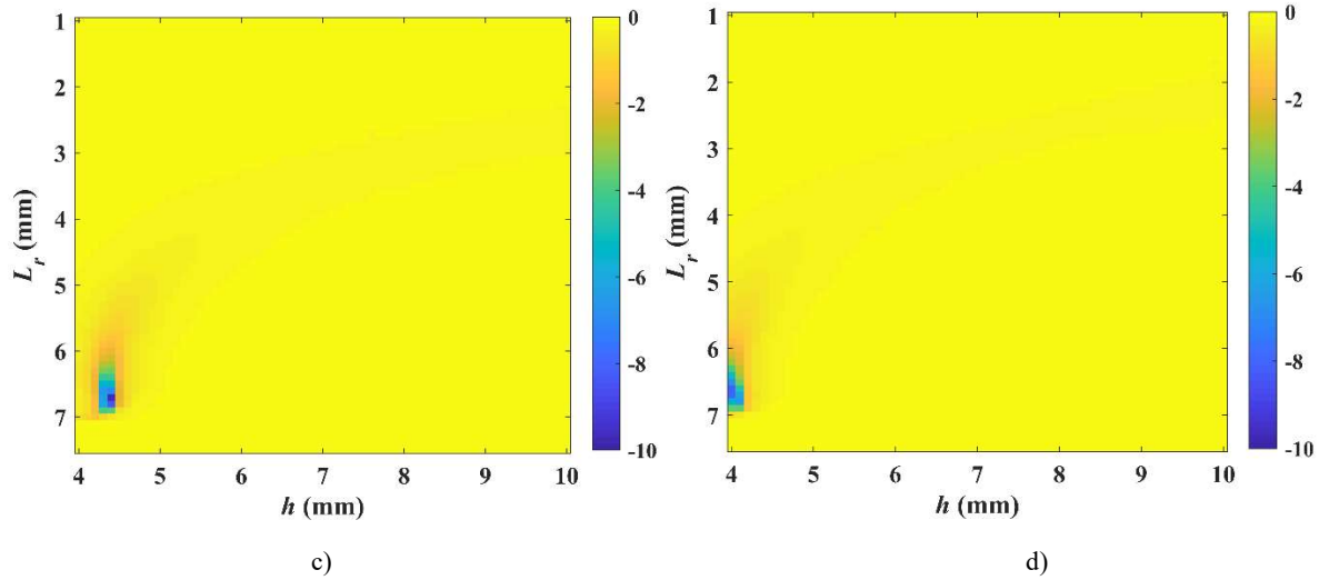
Fig.4.26 S-parameters of the PCSW (x-polarization, \phi_{mc}=90^\circ , \theta_{mc}=25^\circ ). a) Phase ( S_{11} ) at 19.5GHz. b) Phase ( S_{11} ) at 20.5GHz. c) Mag ( S_{11} ) at 19.5GHz. d) Mag ( S_{11} ) at 20.5GHz.
