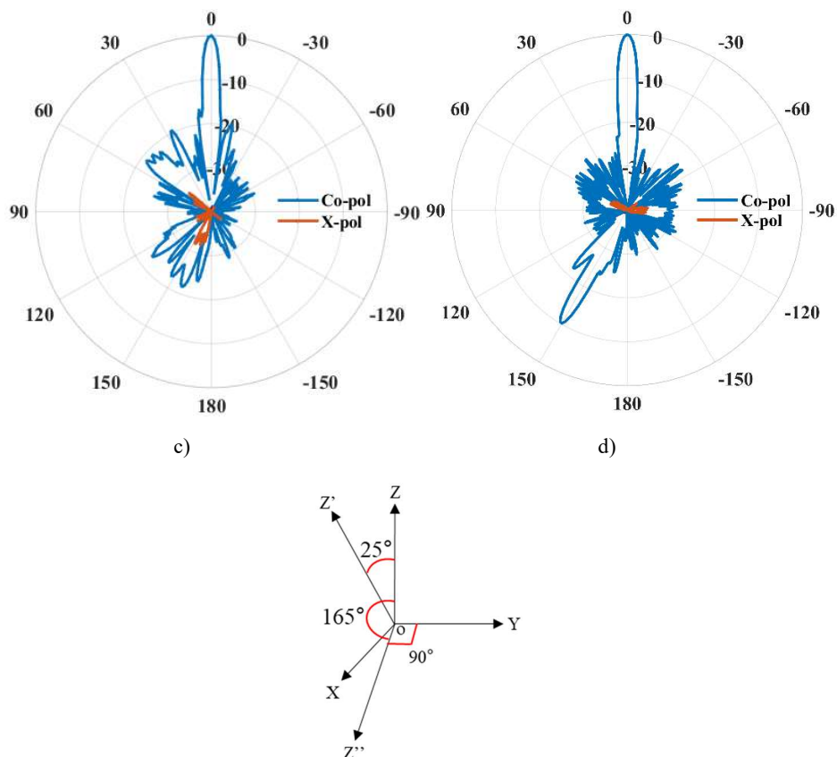
Fig.4.22 Normalized radiation patterns of TRA2 (dB) at 20 GHz - a) yoz plane (reflected beam). b) xoz' plane (reflected beam). c) yoz'' plane (transmitted beam). d) xoz'' plane (transmitted beam)
