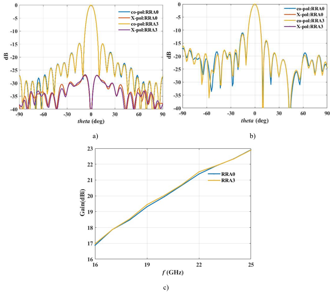
Fig.3.31 The comparison between RRA0 and RRA3 at 20GHz (y-polar excitation). a) Radiation pattern (xoz' plane). b) Radiation pattern (y'oz' plane). c) Gain versus frequency
