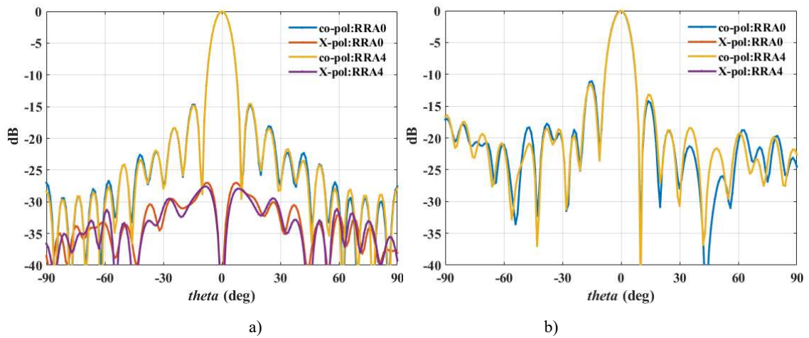
Fig.3.41 Radiation field of RRA4. a) 20GHz. b) 40GHz.
