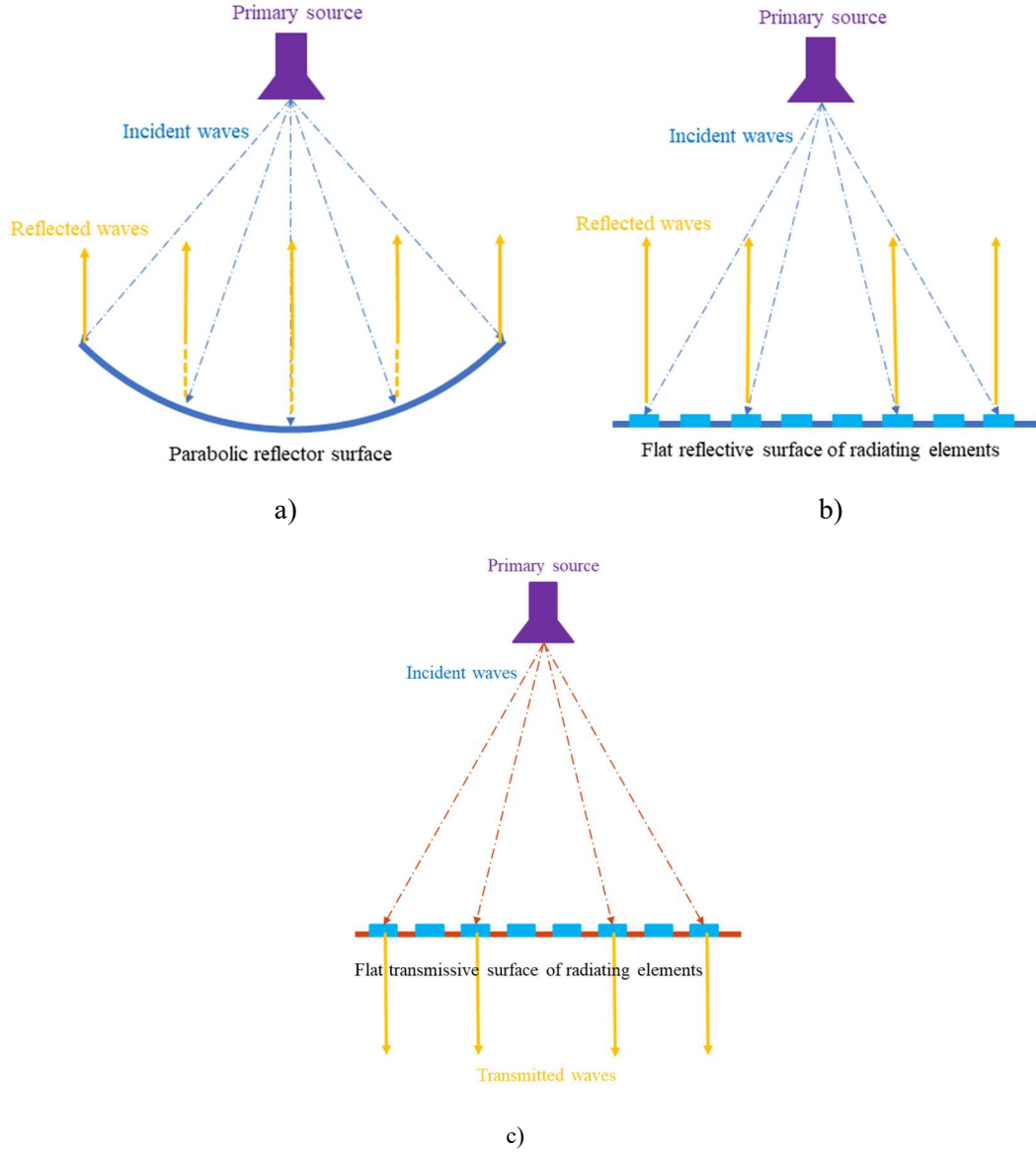
Fig.1.1.1 Principle of: a) Parabolic reflector. b) Reflectarray. c) Transmitarray.
