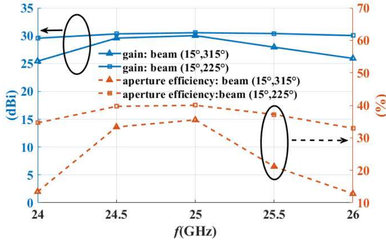
Fig.5.22 Gain responses and aperture efficiencies of two beams.
