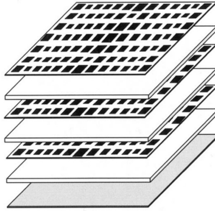
Fig.1.7 schematic model of a three-layer reflectarray using the cells with variable size [40].
