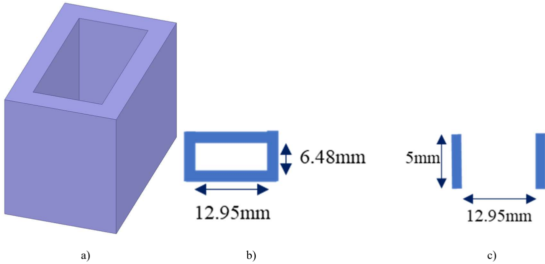
Fig.3.14 Feed antenna (lower band). a) 3D view. b) Top view. c) Sectional view.
