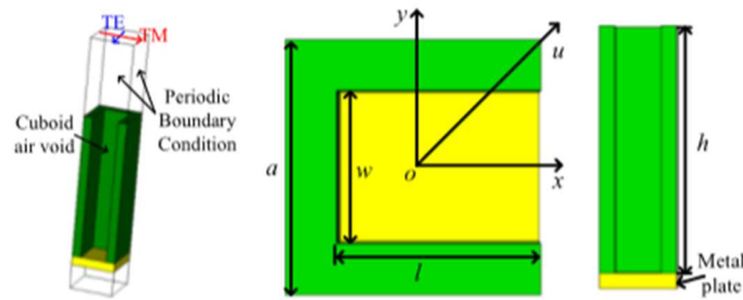
Fig.1.31 Geometry of the unit cell in [114].
