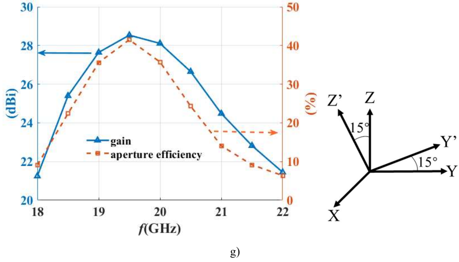
Fig.5.11 Performances in lower frequency band. a) Radiation pattern in xoz' plane (19GHz). b) Radiation pattern in y'oz' plane (19GHz). c) Radiation pattern in xoz' plane (20GHz). d) Radiation pattern in y'oz' plane (20GHz). e) Radiation pattern in xoz' plane (21GHz). f) Radiation pattern in y'oz' plane (21GHz). g) Gain response and aperture efficiency.
