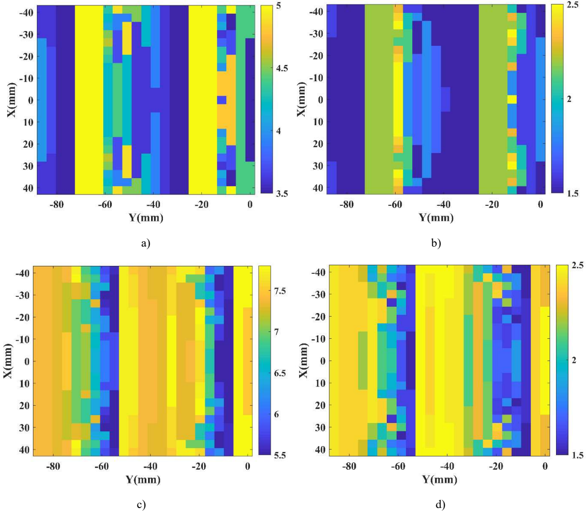
Fig.3.26 Cell geometries in RRA1 and RRA2 (mm). a) RRA1( h ). b) RRA1( L_r ). c) RRA2( h ). d) RRA2( L_r ).
