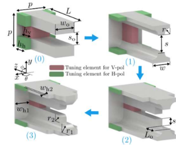
Fig.1.22 Design evolution of the unit cell in [56]
