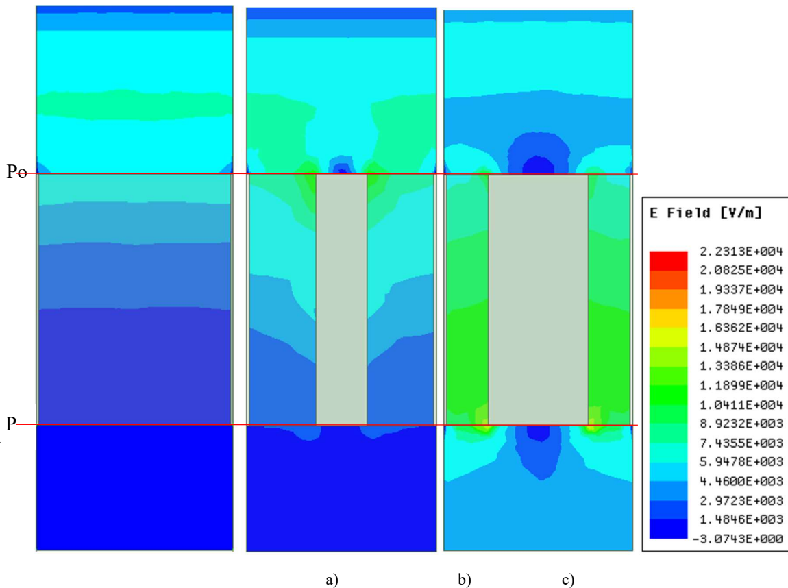
Fig.2.3 The complex magnitude of electric field (XZ plane, middle of the waveguide, normal incidence, y-polarization, f=16\text{GHz} , h=10\text{ mm} ). a) L_r=0 . b) L_r=2\text{ mm} . c) L_r=4\text{ mm} .
