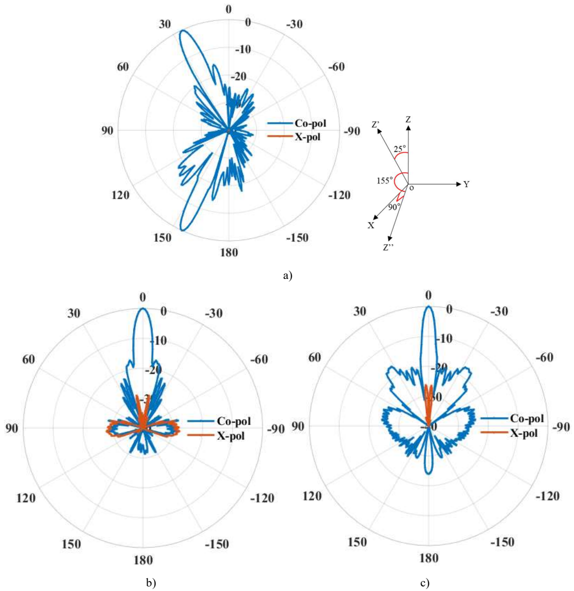
Fig.4.19 Normalized radiation patterns of TRA1 (dB) at 19 GHZ. a) yoz plane. b) xoz' plane. c) xoz'' plane.
