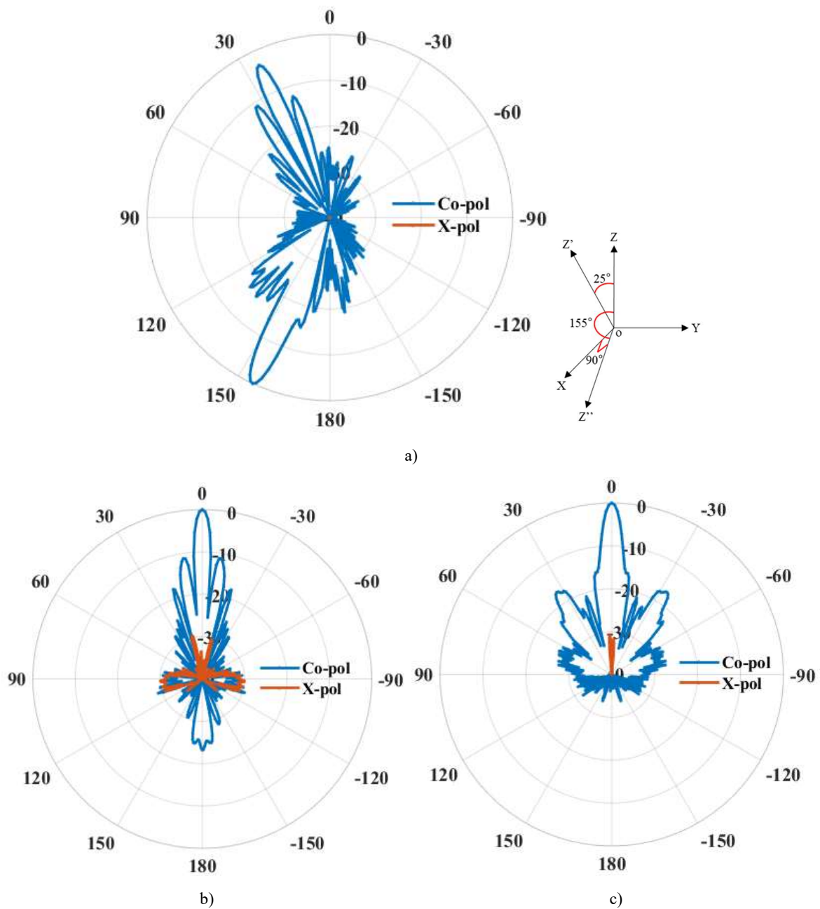
Fig.4.20 Normalized radiation patterns of TRA1 (dB) at 21 GHz. a) yoz plane. b) xoz' plane. c) xoz'' plane.
