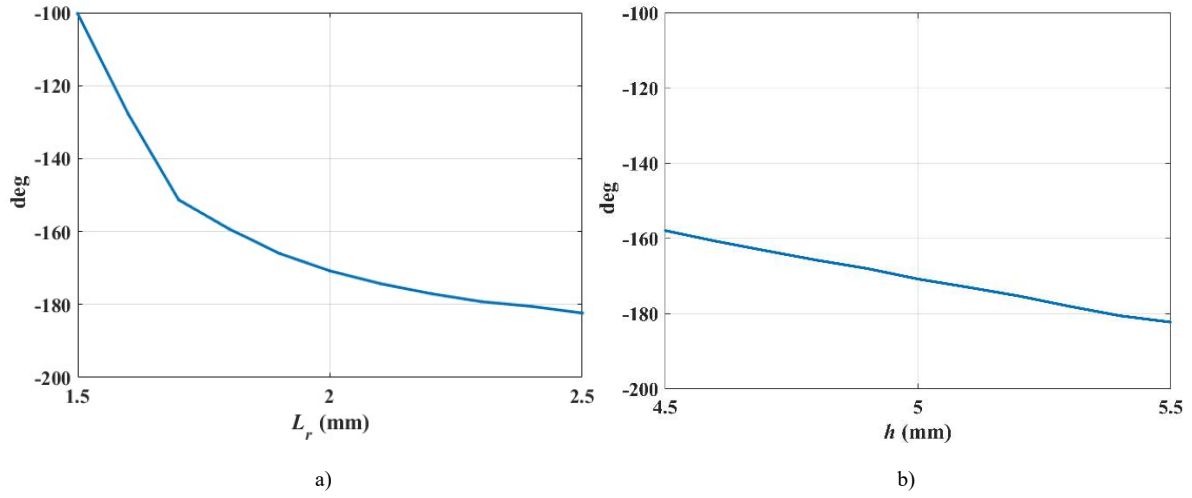
Fig.3.54 Comparison of the sensitivity of geometry on reflection phase. a) Reflection phase vs L_r (mm). b) Reflection phase vs h (mm).
