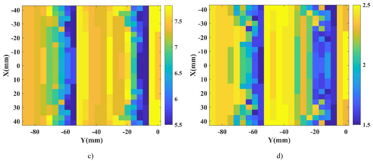
Fig.3.26 Cell geometries in RRA1 and RRA2 (mm). a) RRA1( h ). b) RRA1( L_r ). c) RRA2( h ). d) RRA2( L_r ).
