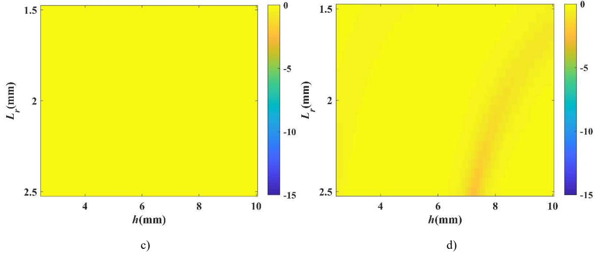
Fig.3.4 Reflection phase and magnitude under oblique incidence (TE case, \phi_{nc}=90^\circ , \theta_{nc}=22.54^\circ ). a) Phase at 20GHz (deg). b) Phase at 40GHz (deg). c) Magnitude at 20GHz (dB). d) Magnitude at 40GHz (dB).
