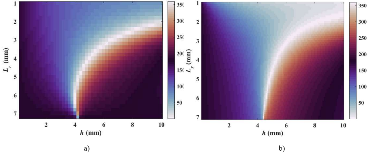
Fig.2.8 Phase of reflection coefficient at 20GHz (normal incidence). a) Full wave simulation results. b) Theoretical model.
