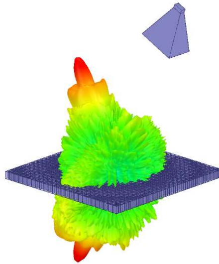
Fig.4.17 TRA1 with symmetrical beams at 20GHz and horn antenna.
