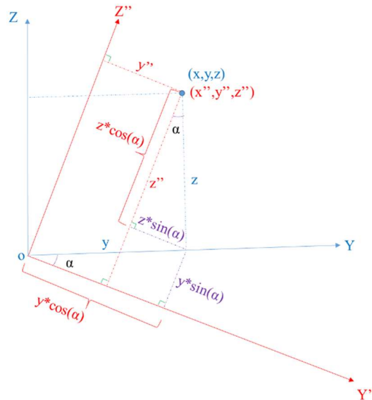
Fig.3.35 Transformation of the coordinates before and after rotation.
