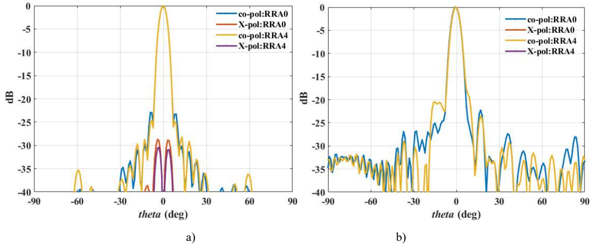
Fig.3.42 Comparison between the performances of RRA0 and RRA4 in the lower frequency band. a) Radiation pattern at 20GHz (xoz plane). b) Radiation pattern at 20GHz (yoz plane). c) Gain versus frequency.
