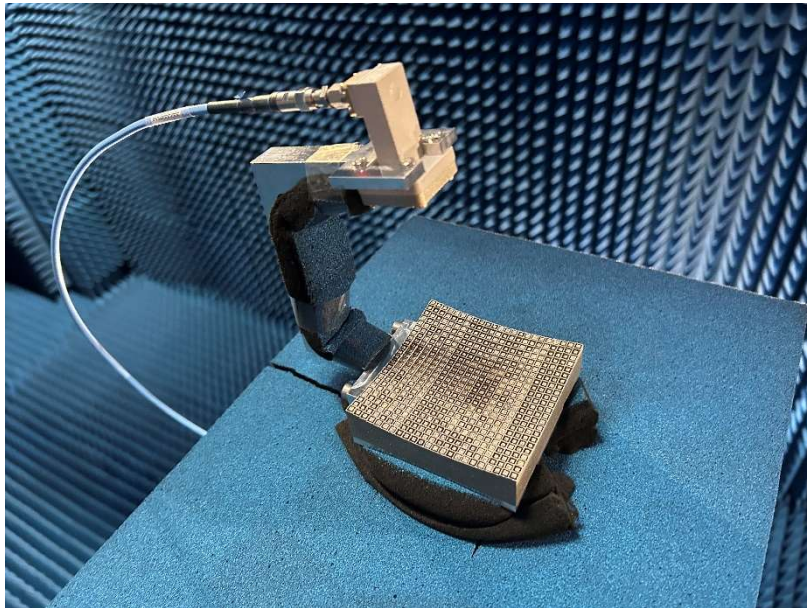
Fig.3.48 Photographs of manufactured MORRA and its measurement setup.
