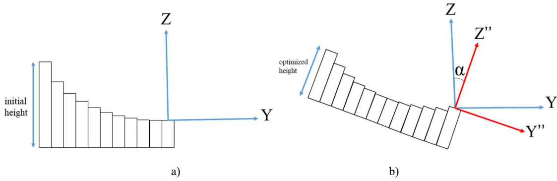
Fig.3.34 Rotation of the coordinate system (sectional view). a) The configuration before rotation. b) The configuration after rotation.
