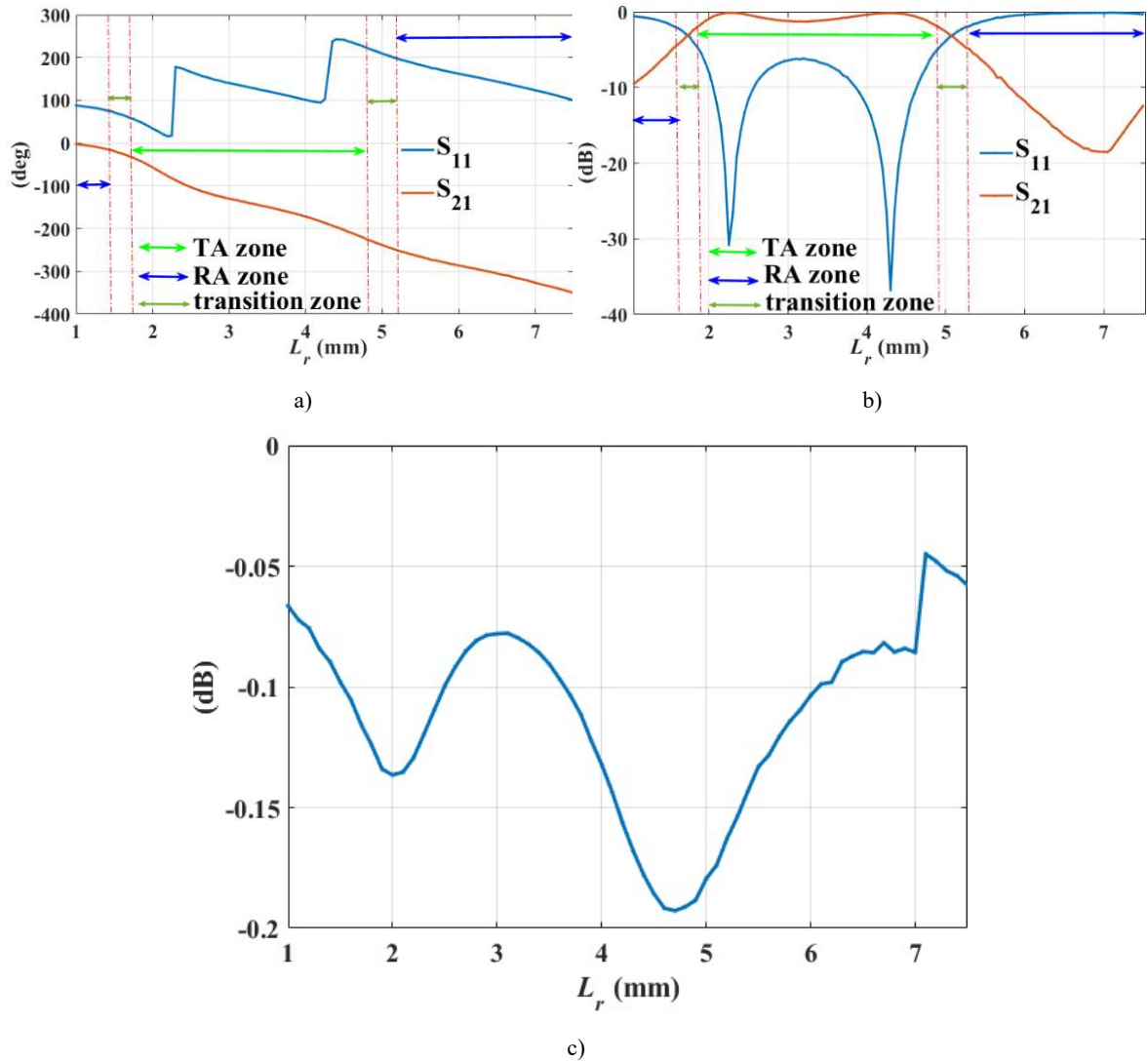
Fig.4.13 The simulated S-parameters of the PCOW ( h=10 mm, step=0.05 mm, f=20 GHz, x-polarization, \phi_{nc}=90^\circ , \theta_{nc}=25^\circ ).
