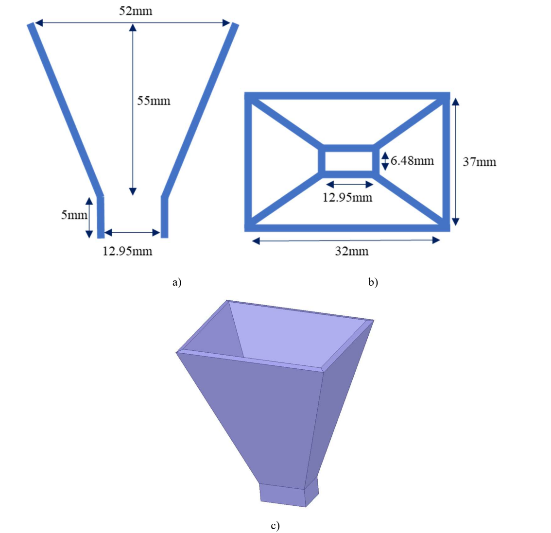
Fig.4.3 The designed horn antenna. a) Sectional view. b) Top view. c) 3D view
