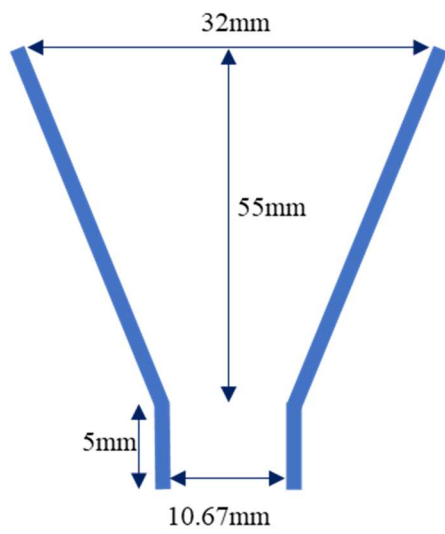
Fig.5.4 Designed horn antenna (20GHz). a) Sectional view. b) Top view. c) 3D view.
