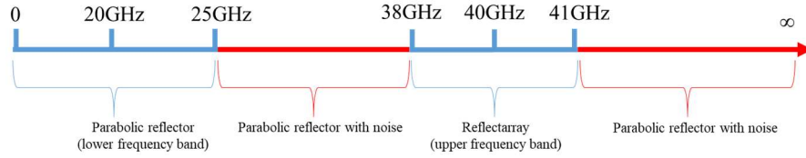
Fig.3.23 Operating modes of the proposed MORRA
