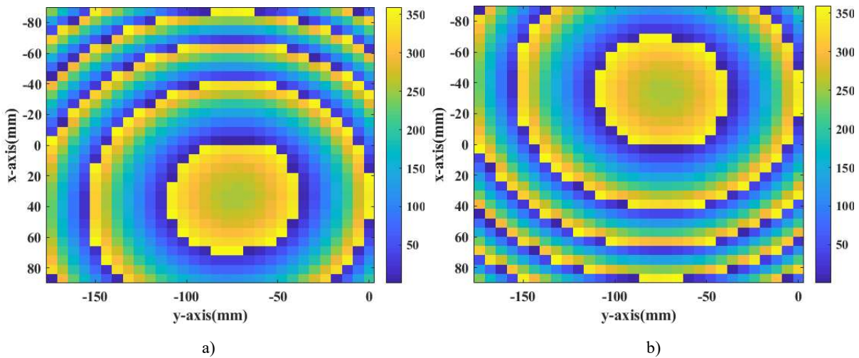
Fig.5.16 Distribution of required phase shift over the cells (deg). a) For beam (15°, 315°). b) For beam (15°, 225°).
