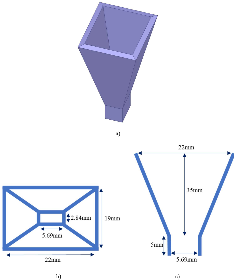
Fig.3.14 Feed antenna (lower band). a) 3D view. b) Top view. c) Sectional view.
