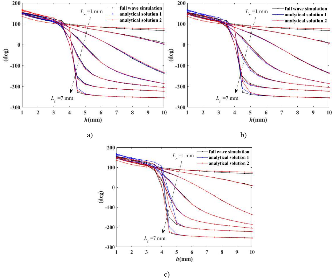
Fig.2.21 Reflection phase. a) Combination 1. b) Combination 2. c) Combination 3.
