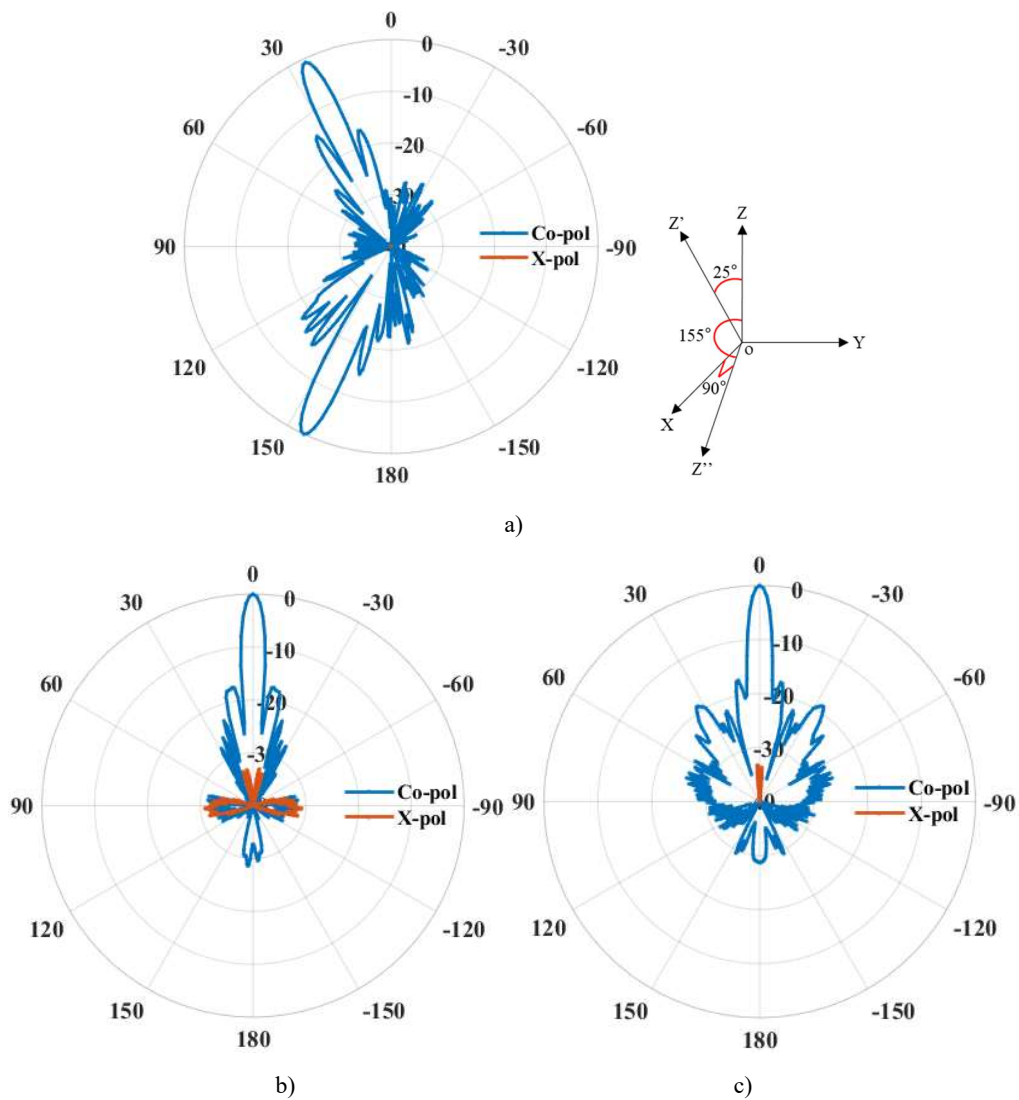
Fig.4.17 TRA1 with symmetrical beams at 20GHz and horn antenna.
