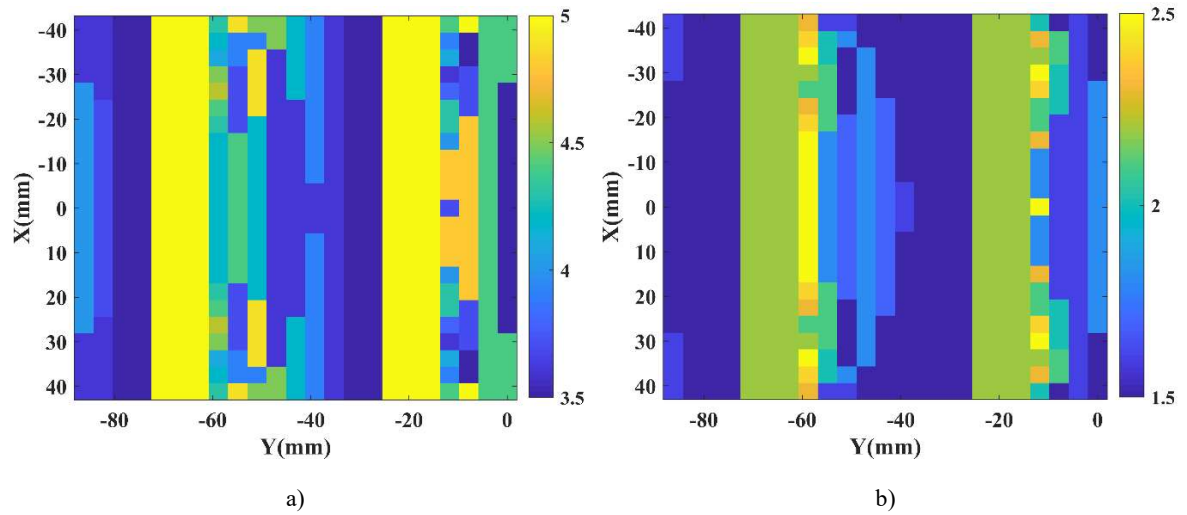
Fig.3.25 Phase error distribution of 3 different RRAs at 40GHz (deg). a) RRA0. b) RRA1. c) RRA2.
