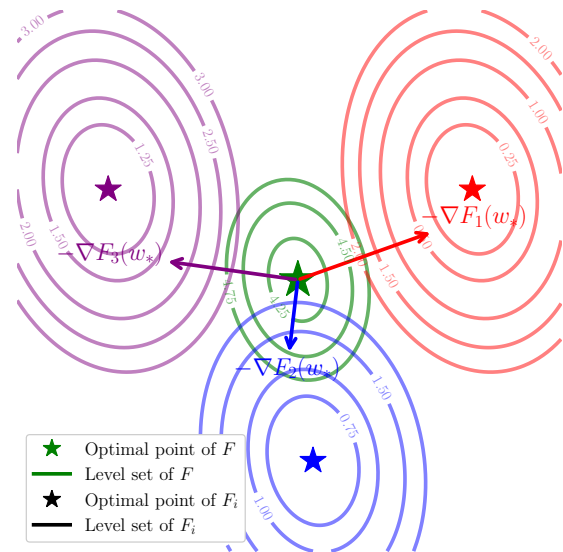
Figure 1.6: Illustration of heterogeneity on three clients, the objective functions are quadratic. We represent the optimal points, the level set, and the opposite gradient at the optimal point.
