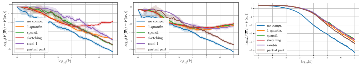
(a) Features' covariance diagonal with high eigenvalues' decay. (b) Features' covariance not diagonal with high eigenvalues' decay. (c) Features' covariance not diagonal with slow eigenvalues' decay.
