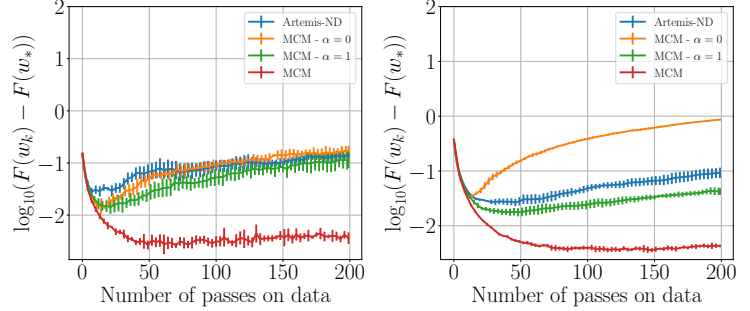
Figure 3.1: Comparing MCM on two datasets (left quantum, right a9a) with three other algorithms using a non-degraded update, \gamma = 1/L . Artemis-ND stands for Artemis with a non-degraded update.
