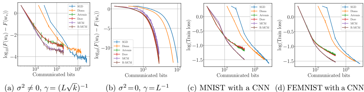
Figure 3.2: Convergence on synthetic datasets (left) and neural networks (right).
