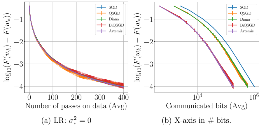
Figure B.5: Polyak-Ruppert averaging, synthetic dataset . Logistic regression on non-i.i.d. data using a full batch gradient descent (to get \sigma_* = 0 ) and a Polyak-Ruppert averaging. The convergence is sublinear as predicted by Theorem 2.2 because \sigma_* = 0 .
