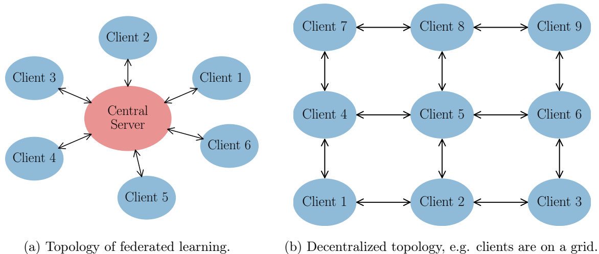
Figure 1.5: Example of two topologies in distributed learning.
