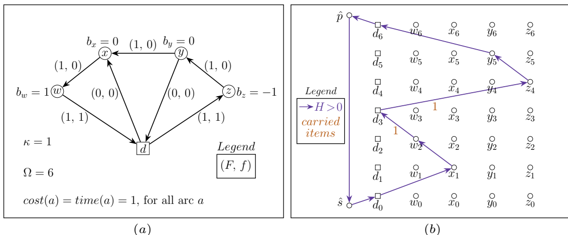
Figure 2.19: An example of the Partial Lift Problem. (a) A PIRP solution (F', f') on a digraph G = (X, A) . (b) A solution (H, h) for the TEN IRP with optimal cost among all the the TEN IRP solutions whose time-projection (F', f') is such that f' = f . Here, H is a unitary flow, and we only have depicted the arcs a with H(a) > 0 . Arcs labels indicate the number of carried items.
