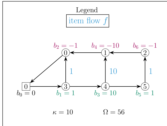
Figure 3.15: An example of item flow f over the same instance in Figure 3.14. Note that f allows to transport the items from excess vertices to deficit vertices, and is feasible-path-decomposable for the time horizon \Omega = 56 .
