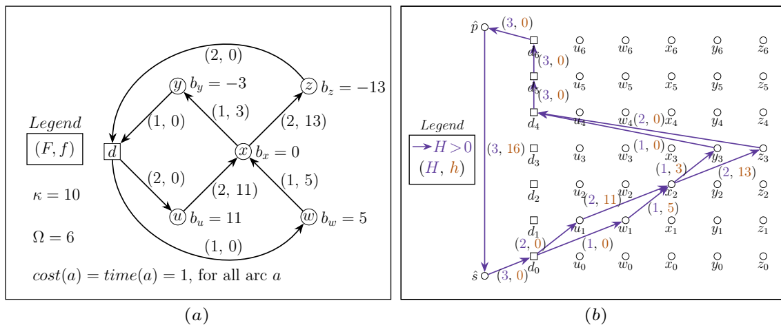
Figure 2.18: An example of the Strong Lift Problem. (a) An optimal solution (F, f) of a PIRP instance. (b) A solution (H, h) for the TEN IRP such that it is the minimal cost solution with time-projection equal to the 2-commodity flow (F, f) in (a). We only have depicted the arcs a with H(a) > 0 .
