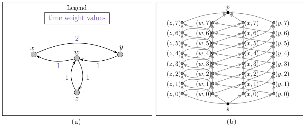
Figure 4.1: Construction of a Time-Expanded network. (a) A digraph G = (X = \{w, x, y, z\}, A = \{(z, w), (w, x), (x, y), (y, w), (w, z)\}) . Arc labels indicate the time necessary for traversing each arc. (b) The Time-Expanded network G^\Omega with time horizon [0, \Omega = 7] constructed from (a). Because the time weights are integral, we only need to consider the integral values t_i in the interval [0, 7] .
