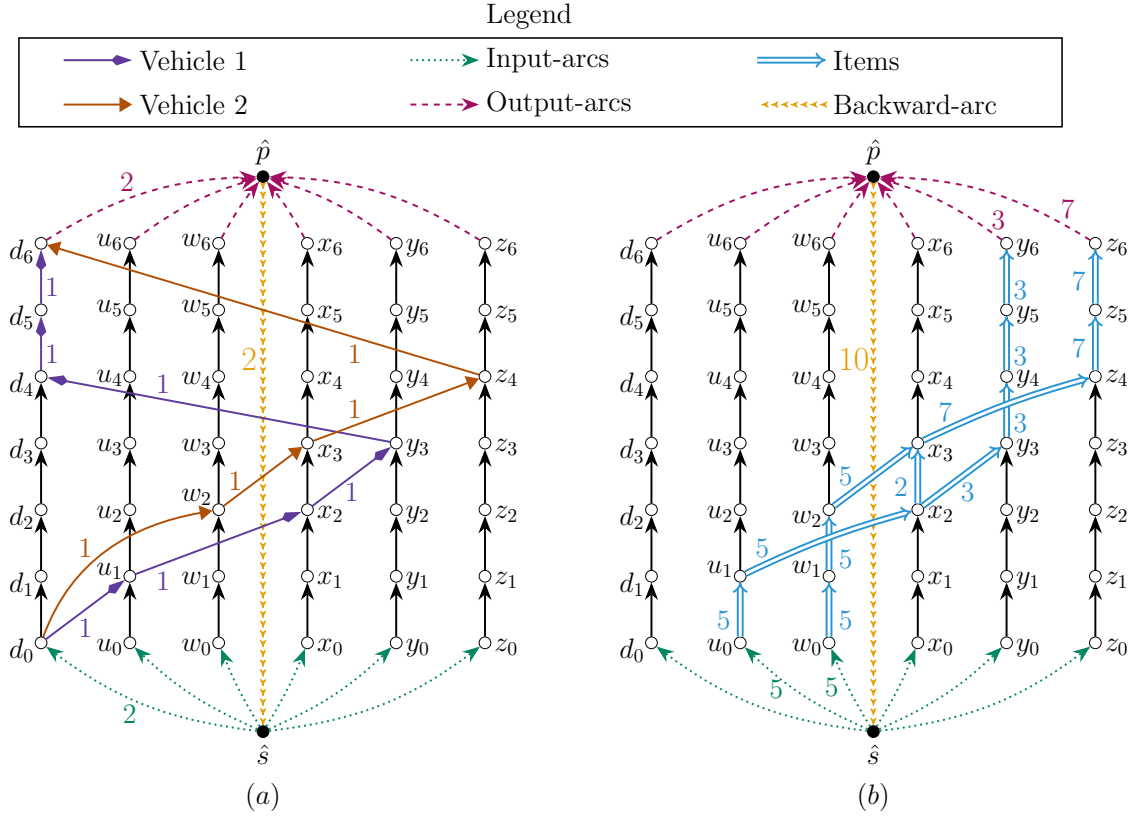
Figure 2.2: The routes and schedules from Example 2.1 viewed as a 2-commodity flow on the Time-Expanded network G^\Omega = (X^\Omega, A^\Omega) . (a) Vehicle flow H in G^\Omega . (b) Item flow h in G^\Omega .
