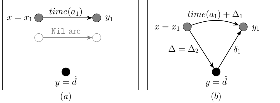
Figure 4.6: A virtual-arc a^{virt} = (x, y, a_1, a_2) with a_2 = \text{Nil} , y = \hat{d} , and x \neq \hat{o} . (a) Components of a^{virt} . (b) The effect of adding the arc a^{virt} in (a) to digraph H . It increases the value \text{time}(a_1) by \Delta_1 , creates a new real-arc (x_1, \hat{d}) with \text{time}((x_1, \hat{d})) = \Delta = \Delta_2 , and creates a new real-arc (\hat{d}, y_1) with \text{time}((\hat{d}, y_1)) = \delta_1 .
