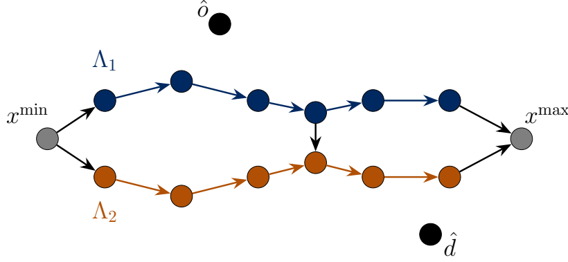
Figure 4.2: Two isolated vertices \hat{o} and \hat{d} , and a connected digraph H = (X, A) involving paths \Lambda_1 and \Lambda_2 . Note that \hat{o} and \hat{d} are not vertices of H .
