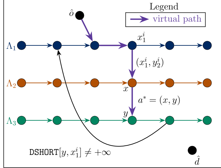
Figure 4.9: The figure used in the proof of Lemma 4.3. Given a state s = (y, virt(s)) with virt(s) = (a_1^{virt} = (x_1^1, y_1^1, a_1^1, a_2^2), \dots, a_\nu^{virt} = (x_1^\nu, y_1^\nu, a_1^\nu, a_2^\nu)) , we can verify that the virtual path from \hat{o} to y codified by s induces a cycle in A \cup A^{add}(\pi) by checking if DSHORT[y, x_1^i] \neq \infty for some i = 1, \dots, \nu .
