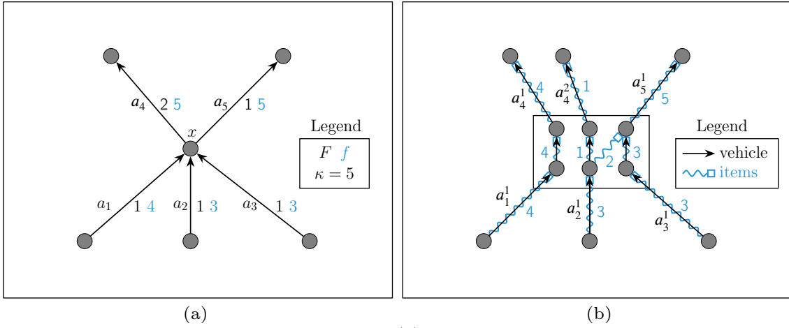
Figure 3.1: The Strong Lift Problem. (a) A set of arcs a_1, a_2, a_3, a_4, a_5 that are incident with a common vertex x , together with their corresponding flow values in a PIRP solution (F, f) . (b) “Expanding” vertex x makes appear the way vehicles and items distribute themselves between the arcs a_1, a_2, a_3 which arrive into x and the arcs a_4, a_5 which leave x .
