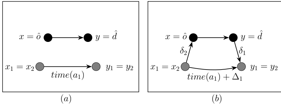
Figure 4.7: A virtual-arc a^{virt} = (x, y, a_1, a_2) with x = \hat{o} , y = \hat{d} , and a_1 = a_2 \in A . (a) Components of a^{virt} . (b) The effect of adding the arc a^{virt} in (a) to digraph H . It increases the value \text{time}(a_1) by \Delta_1 , creates a new real-arc (\hat{o}, \hat{d}) with \text{time}((\hat{o}, \hat{d})) = \Delta , creates a new real-arc (x_2, \hat{o}) with \text{time}((x_2, \hat{o})) = \delta_2 , and creates a new real-arc (\hat{d}, y_1) with \text{time}((\hat{d}, y_1)) = \delta_1 .
