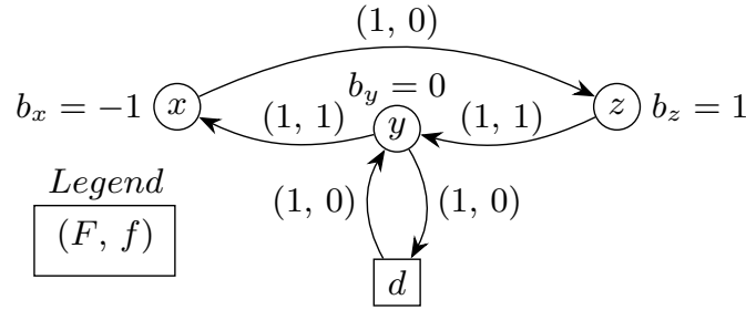
Figure 2.16: A solution of PIRP which cannot be lifted.
