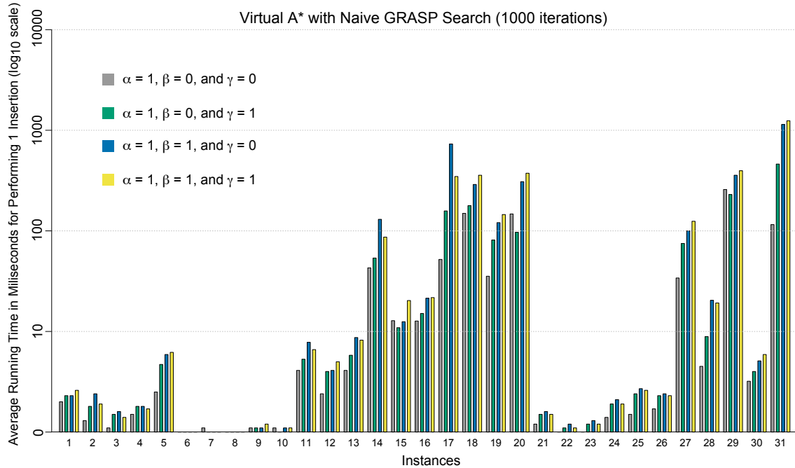
Figure 4.23: The average running time in milliseconds for performing the insertion of one request while considering the different combinations of cost parameters with \alpha = 1 , \beta \in \{0, 1\} , and \gamma \in \{0, 1\} . These values were calculated by averaging the running times per iteration of executing Algorithm 10 with 1000 iterations over each instance in Table B.4. Note the logarithmic scale ( \log_{10} ).
