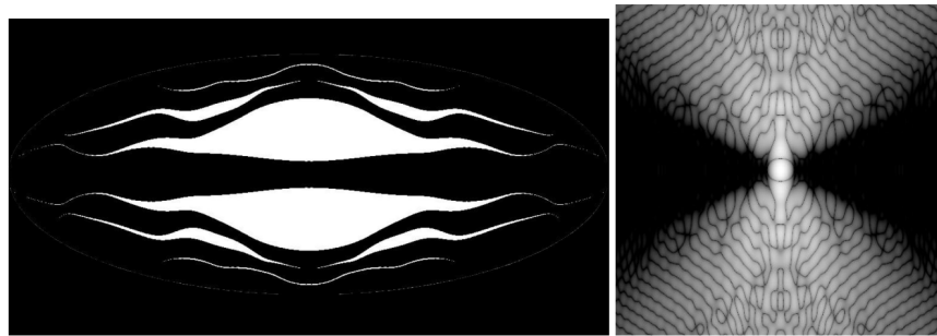
Figure 2.3: An example of a shaped pupil with multiple openings designed for an elliptical aperture. A contrast of 10^{-10} along the x-axis can be achieved up to a distance of 4 \lambda/D (Kasdin et al., 2005).
