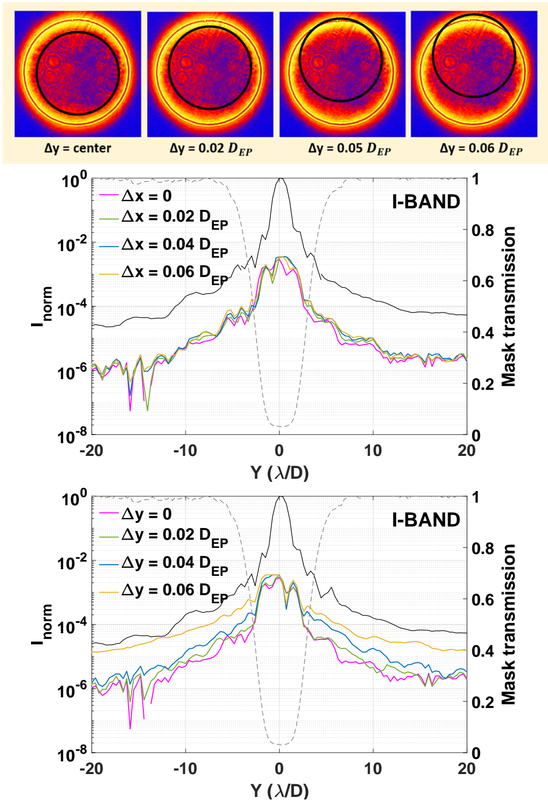
Figure 4.24: Normalized irradiance for each corresponding LS (black circle) misalignment along the y-axis. A misalignment of up to 84 \mu\text{m} ( 0.02 D_{EP} ) does not significantly affect the normalized irradiance at the IWA_X \approx 3.00 \lambda/D .
