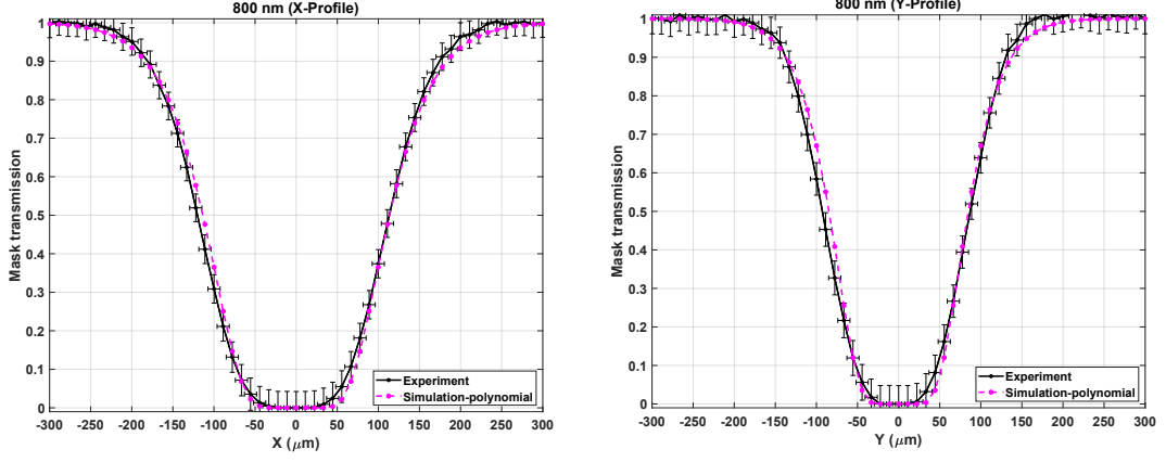
Figure 4.8: Comparison between the theoretical and measured mask response along the major axis of the mask (x-axis) and the minor axis (y-axis). Horizontal error bars are equal to \pm 1 pixel, while vertical error bars represent a standard deviation from the 101 flat-field image obtained.
