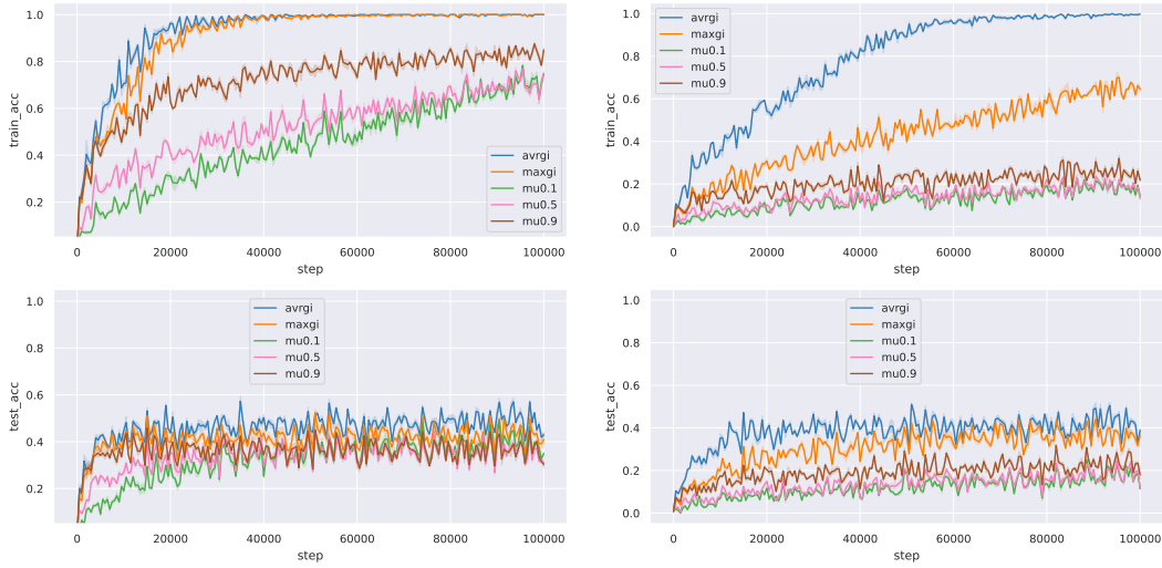
Figure 2.4: CIFAR100: Training (top) and test (bottom) accuracies for adagrad -like ( \mu \in (0.1, 0.5, 0.9) ), maxgi and avrgi variants with \alpha = 5.10^{-4} (left) and \alpha = 5.10^{-5} (right) on the resnet18 architecture
