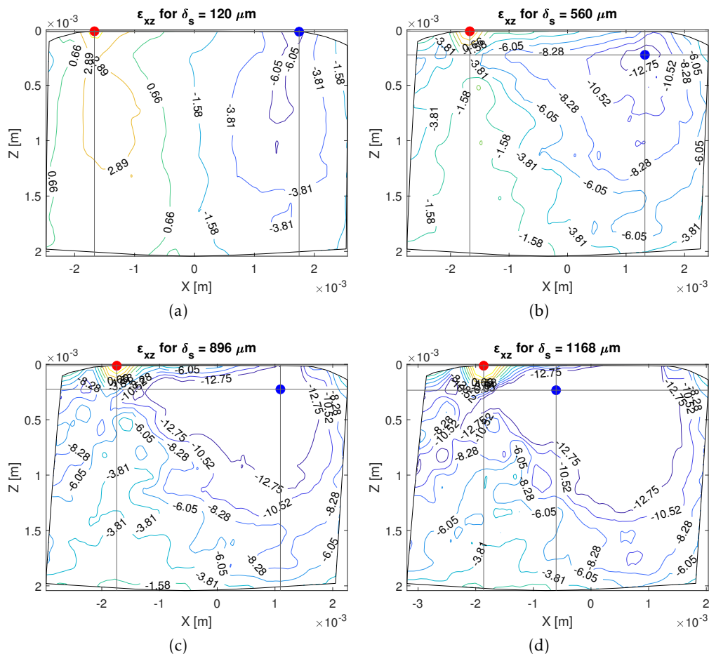
Figure 4.25: Contour plots of the strain component \varepsilon_{xz} (in %) on the central X - Z plane obtained with the DVC measurement for the specimen B-10-A at four consecutive shear steps. The red and blue points stand, respectively, for the maximum and minimum values of the strain in the relative plot.
