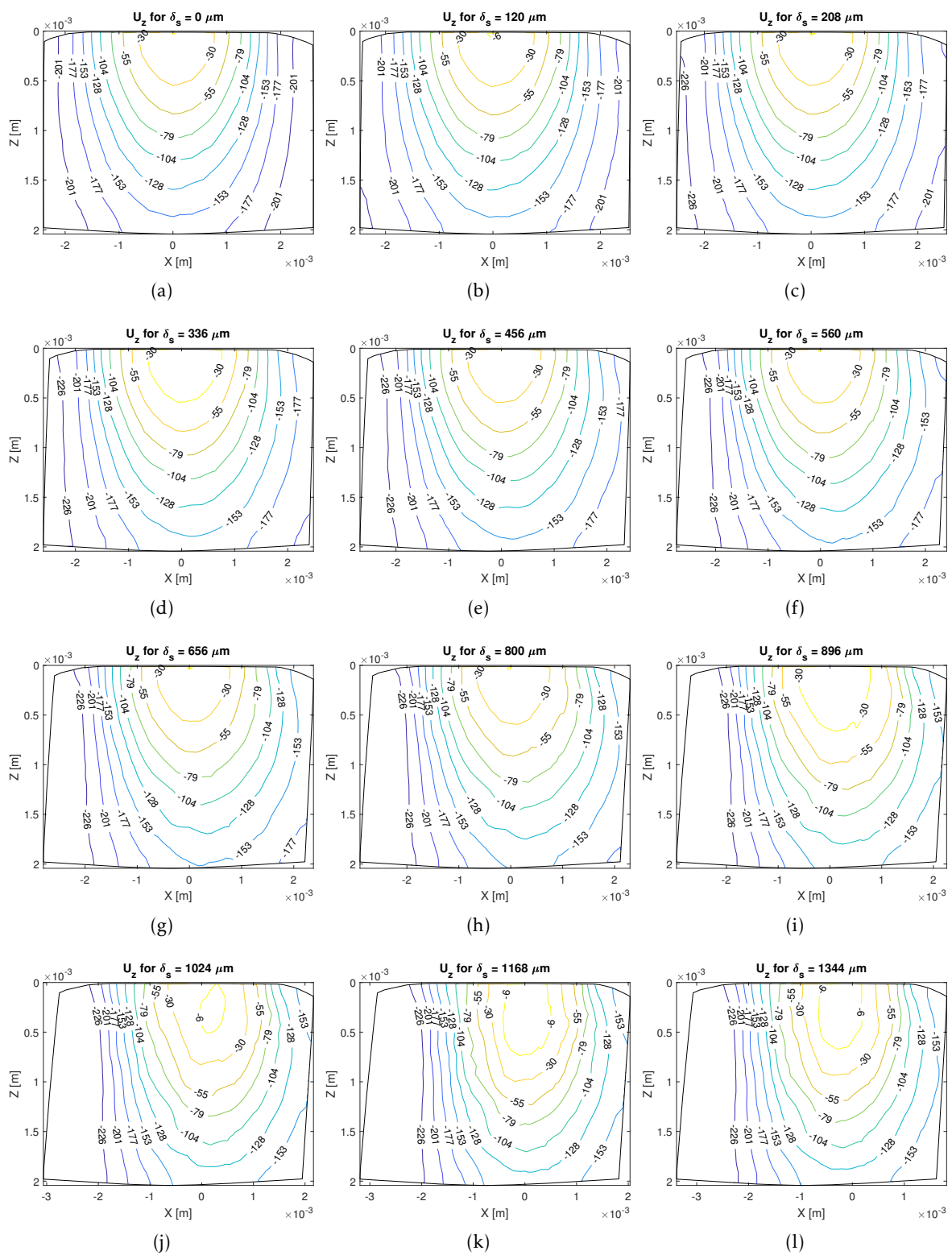
Figure 6.10: Isolines of the component U_z during shear (data are in micrometers) starting from the contour plot at the end of normal compression. The ROI is deformed according to the displacement field. Specimen B-10-A.
