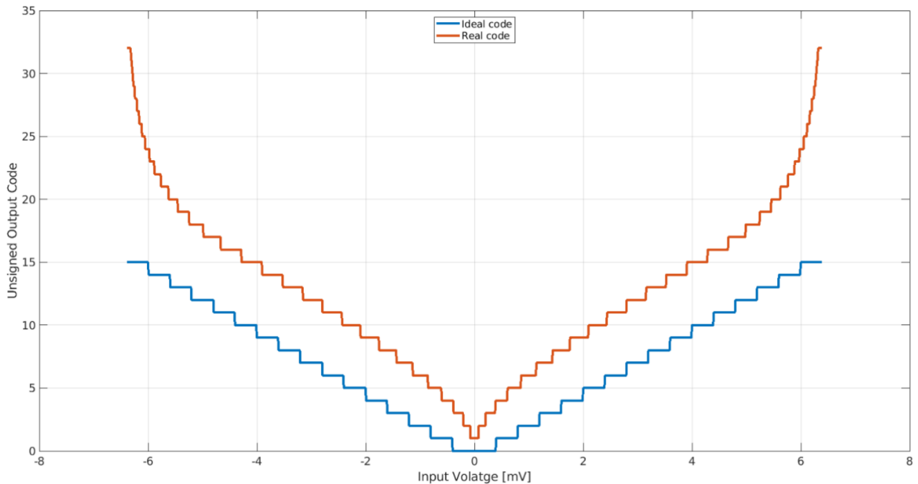
Figure 82 – Simulated unsigned output code vs. ideal unsigned output code over the \pm 4 bit input range (LSB = 400\mu\text{V} , BW = 637MHz, Timestep 50ps, 16 steps)
