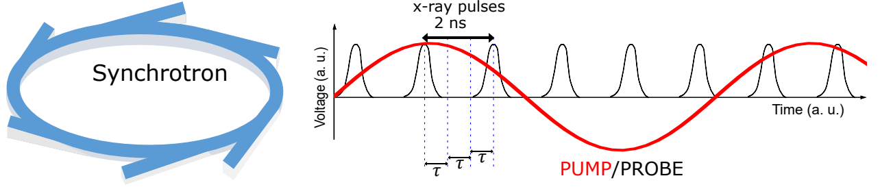
Fig. 3.14: Pump-probe mechanism | Schematics of the pump-probe setup. The photons from the synchrotron arrive every 2 ns (500 MHz). The pump period is a fractional multiple of the probe period and this creates a shift of \tau after each pump cycle between pump and probe. This adds up to the full 2 ns probe period after an integer number M of pump cycles, resulting in a time resolution of \tau for the acquisition. In this example: N = 17 , M = 3 , T_P = 11.33 ns, \tau = 0.667 ns.
