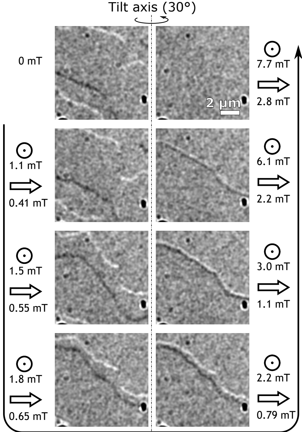
Fig. 6.18: Magnetic field series observation in TEM | Fresnel magnetic field series of the saturation of the stack. Defocus has been measured at 33 nm. Values of magnetic field both in- and out-of-plane are given according to the measured tilt of 30°. Images are 10x10 \mu\text{m}^2 in size.
