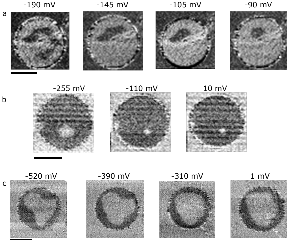
Fig. 6.8: DC voltage dependencies for different magnetic textures in a 2 \mu m MTJ pillar | a Sequence of STXM images showing voltage dependence of the magnetic texture in the MTJ at -2.3 mT. b Another sequence of successive STXM images showing isolated skyrmions for different DC voltages and an out-of-plane external magnetic field of 4 mT. c Skyrmions also showing a variation in size with the DC voltage at an external out-of-plane field of -2.3 mT. The scale bar in every sequence is 1 \mu m. The images in are normalized with respect to an STXM image of the dot in the AP resistance state at a field of -20 mT.
