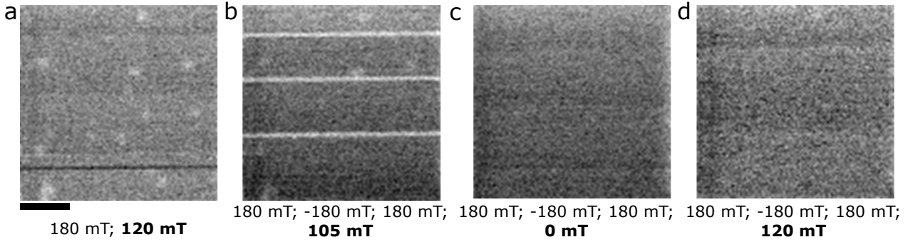
Fig. 5.12: Erasing and nucleating SAF skyrmions with x-rays | Sequence of successive STXM imaging (Fe L_3 edge) to study the effect of the x-ray beam on the skyrmion stabilization. a STXM image for a perpendicular magnetic field of 120 mT (after applying a field of 180 mT) showing magnetic skyrmions. b STXM image after a field sequence of 180 mT; -180 mT; 180 mT; 105 mT. No image was acquired during the field sweep sequence. The white lines are experimental errors. c Same at zero field where no skyrmions are observed. d Same after a field sequence 180 mT; -180 mT; 180 mT; 120 mT, having erased the skyrmions. The numbers in bold are the field applied at the imaging moment. The scale bar is 1 \mu\text{m} .
