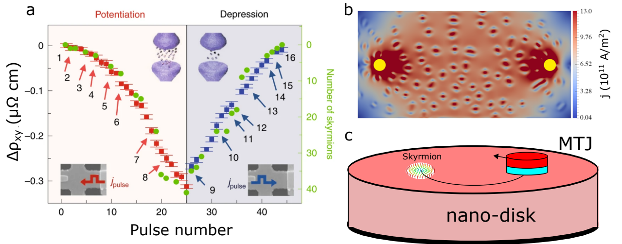
Fig. 2.9: Towards for non-conventional skyrmion-based applications | a Correlation between Hall resistivity measurements (left axis) with the number of skyrmions (right axis) while different polarity pulses are applied. It shows potentiation (red) and depression (blue) depending on the pulse polarity. From [150]. b Distribution of the current in the skyrmionic magnetic texture. The yellow dots are nanocontacts and a voltage (110 mV) is going across them. From [152]. c Schematic of a skyrmionic nano-oscillator where a skyrmion would oscillate and be detected by a MTJ. Some labels have been rewritten for better visualization.
