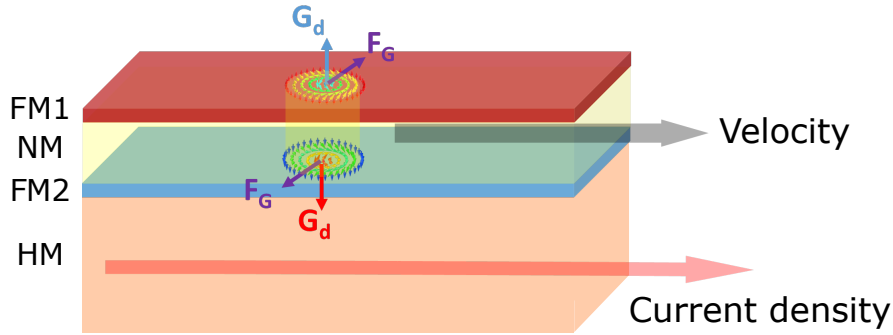
Fig. 2.12: Dynamics of SAF skyrmions in synthetic antiferromagnets | A schematic representation of the dynamics in SAF stacks. FM 1 and FM 2 are AF coupled via the NM. The skyrmions in the individual ferromagnets have opposite polarity but same chirality and are coupled through RKKY interaction. Their respective gyromagnetic forces cancel each other out, resulting in zero transverse displacement. The current goes through the HM and the resulting velocity is parallel to it.
