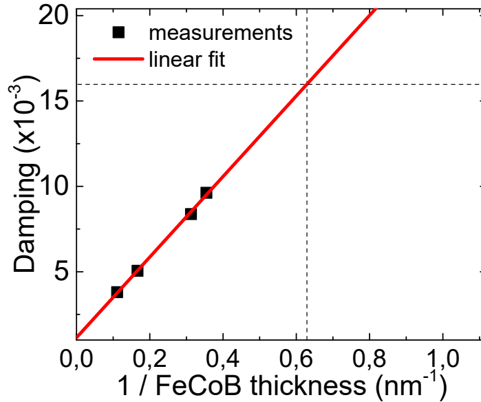
Fig. 6.17: Ferromagnetic resonance measurements | Magnetic damping measurements for different FeCoB thickness measured by FMR showing a linear dependence of the damping with respect to the inverse of the film thickness.
