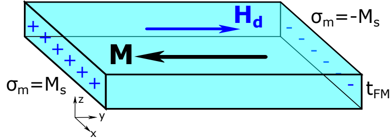
Fig. 1.1: Demagnetizing field | In a thin film geometry, the magnetization tends to align along the plane in order to minimize the magnetic charges it creates. These charges are responsible of creating the demagnetizing field inside the sample which is oriented against the magnetization direction.
