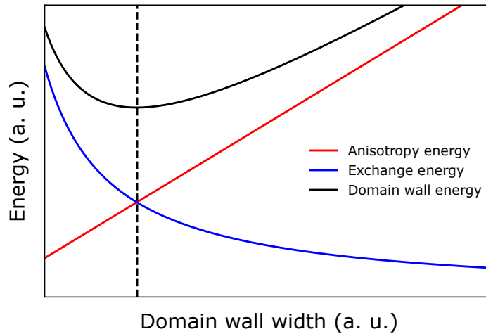
Fig. 1.6: Domain wall energies | Domain wall energy (black) and both exchange (blue) and anisotropy (red) energy contributions as a function of the domain wall width. As the vertical dotted line shows, the minimum in the domain wall energy is the point at which the exchange energy and the anisotropy energy are equal.
