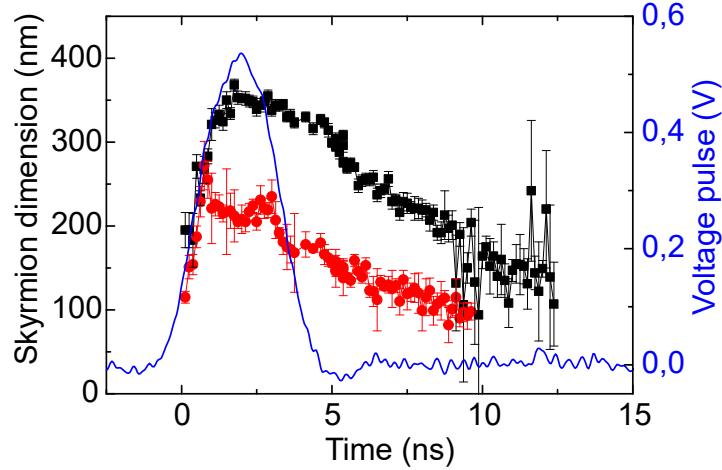
Fig. 4.5: Time evolution of the skyrmion dimension | Diameter values along both x (black) and y (red) directions vs time for the SAF skyrmion. The applied voltage of the pulse is in blue. We induced 3 ns width current pulses with an average current density of about 8.2 \cdot 10^{11} A/m 2 in this case.
