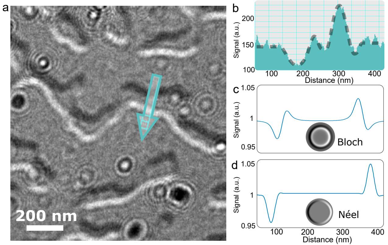
Fig. 6.19: Micromagnetic simulations for TEM analysis | Fresnel contrast obtain at 30^\circ of tilt with a defocus of 85 nm (inset is the same image obtained at 0^\circ of tilt). The experimental contrast profile of the dashed area is shown on top of the right column and compared to the profiles simulated for Néel and Bloch magnetic bubble configuration below (2D contrast displayed as inset under the curves).
