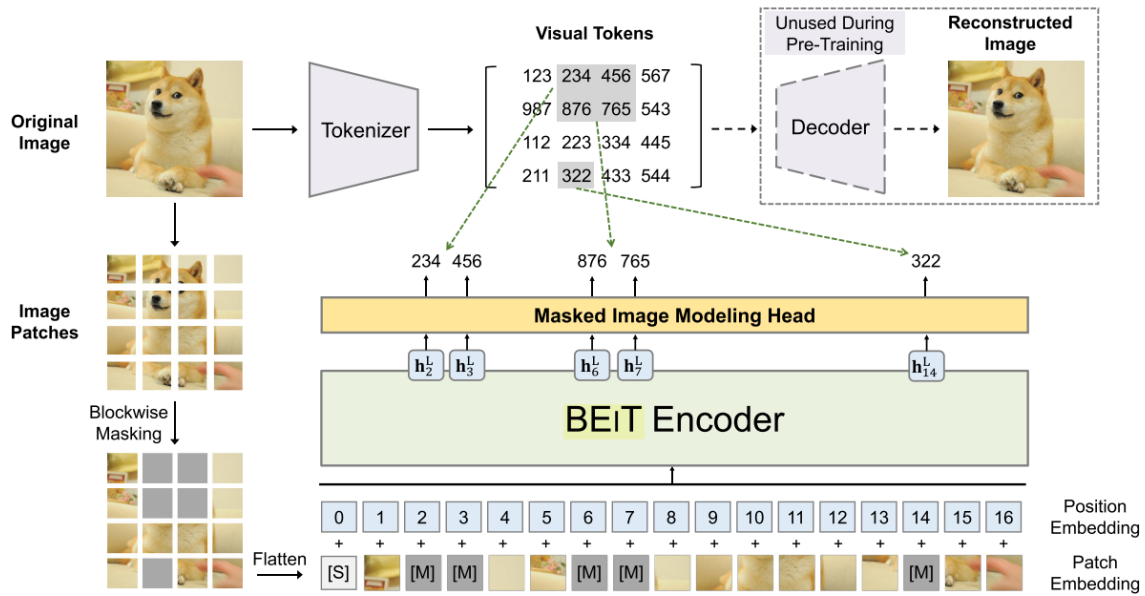
Figure 3.20: Illustration of BEiT [BDPW22] from its paper. The input image is tokenized to input patches, each associated with a visual token computed by a tokenizer. Some patches are corrupted and replaced with a learned masked token. The tokens pass through a transformer encoder and the objective function is to predict the visual tokens of the masked patches.
