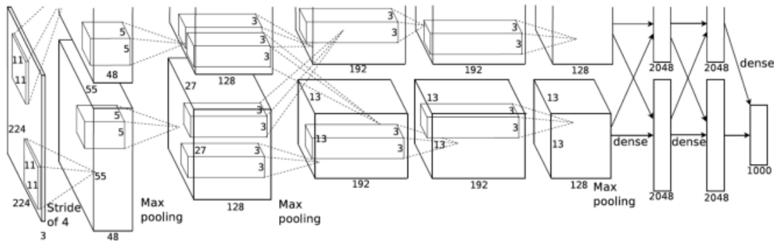
Figure 2.9: AlexNet [KSH12] architecture.
