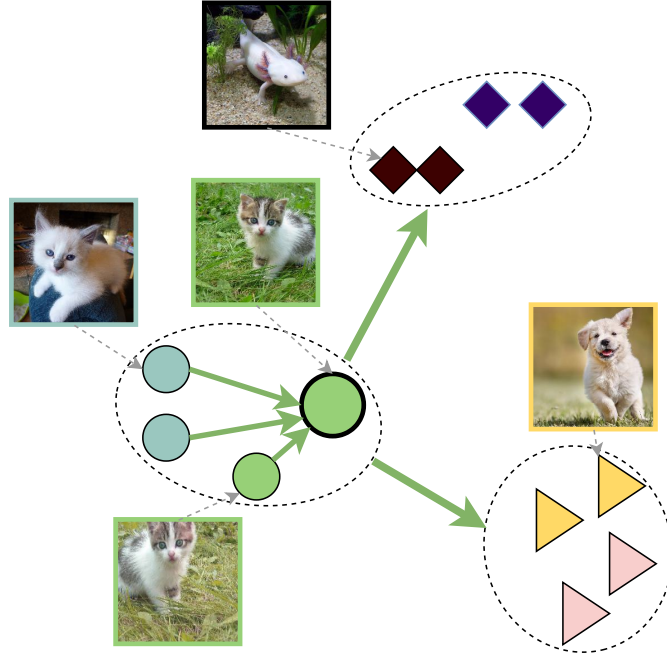
Figure 4.3: Illustration of Similarity Contrastive Estimation (SCE). SCE correctly aligns positives to learn discriminative features and models relations among instances.
