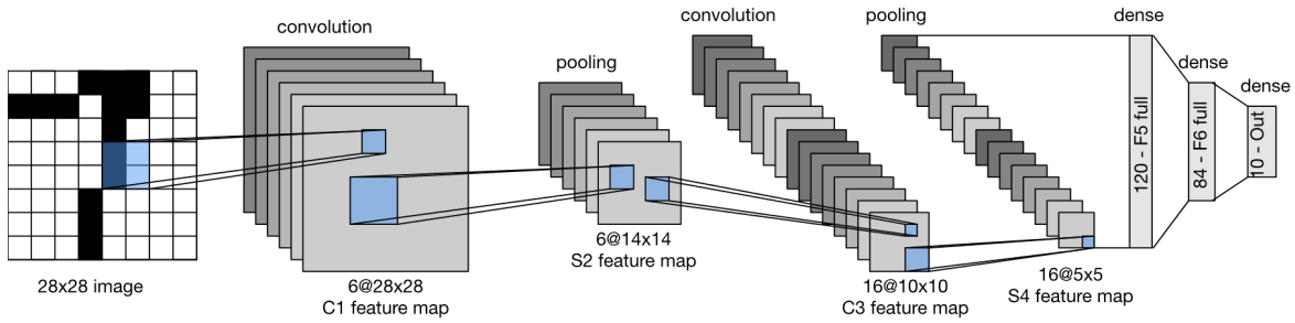
Figure 2.8: LeNet architecture [LBBH98].
