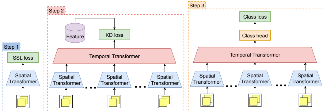
Figure 6.2: Overview of COMEDIAN training pipeline. Step 1: Pretraining of the spatial transformer. Step 2: Pretraining of the spatial and temporal transformers. Step 3: fine-tuning to the action spotting task.
