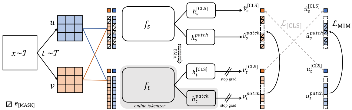
Figure 3.23: Illustration of iBoT from [ZWW + 22b]. Some patches going through the student branches are masked to perform Masked features prediction of the teacher’s outputs. A global contrastive loss is applied to the class tokens.
