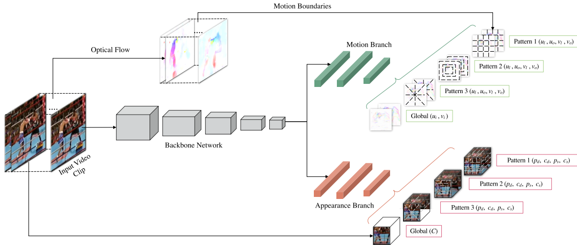
Figure 3.5: Illustration of appearance and motion statistics prediction from [WJB + 19]. Motion and RGB patterns of interest are first extracted to provide supervision to the network.
