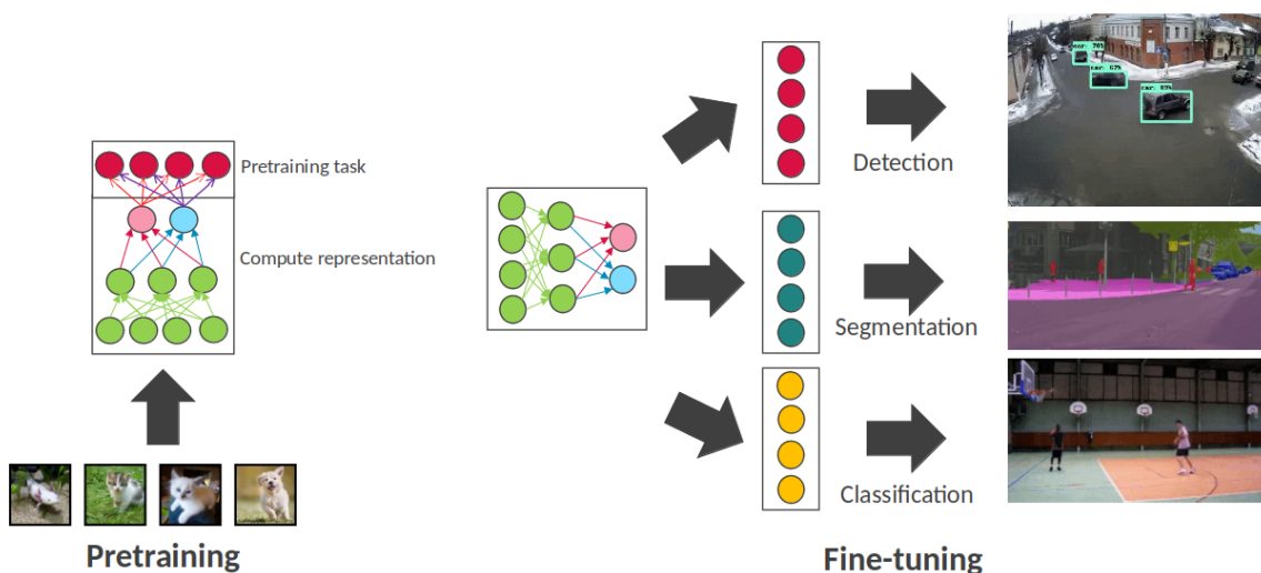
Figure 2.15: (left) Representation learning of a NN separated in two-parts, the backbone that learns representation and the predictor that solve the pretraining task. (right) Finetuning of the backbone or/and training of an NN to specialize in a task.
