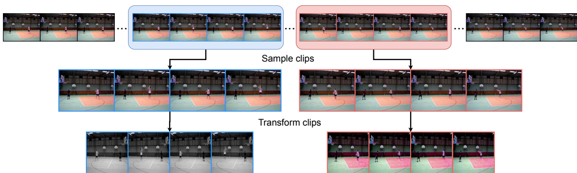
Figure 3.17: Two clips sampled randomly from a video and independently transformed to form positive views.
