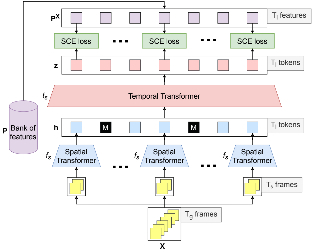
Figure 6.4: Pretraining of the spatial and temporal transformers via knowledge distillation of a bank of features with the SCE loss. Some spatial output tokens are masked.
