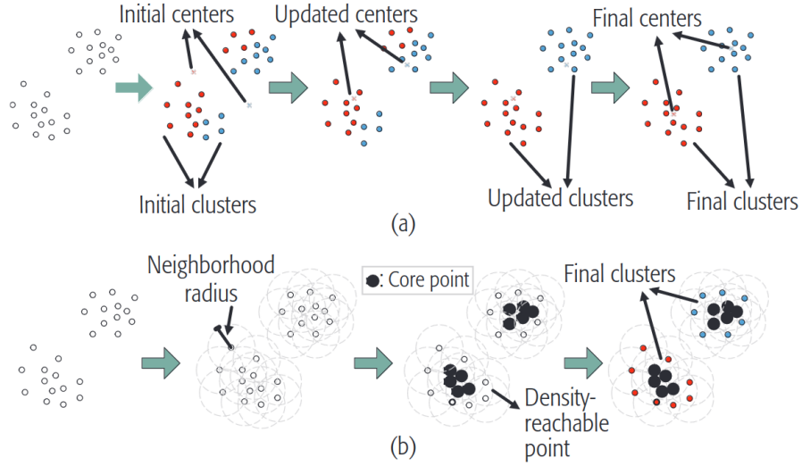
Figure 3.6: (a) k-Means algorithm. (b) DBSCAN algorithm. From [HAM + 18].
