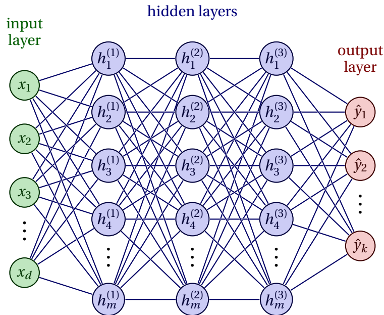
Figure 2.5: Multi-Layer Perceptron composed of an input layer, three hidden layers, and an output layer. It contains fully connected layers, therefore, neurons of each layer are connected to all neurons of the previous layer and all the neurons of the next layer.
