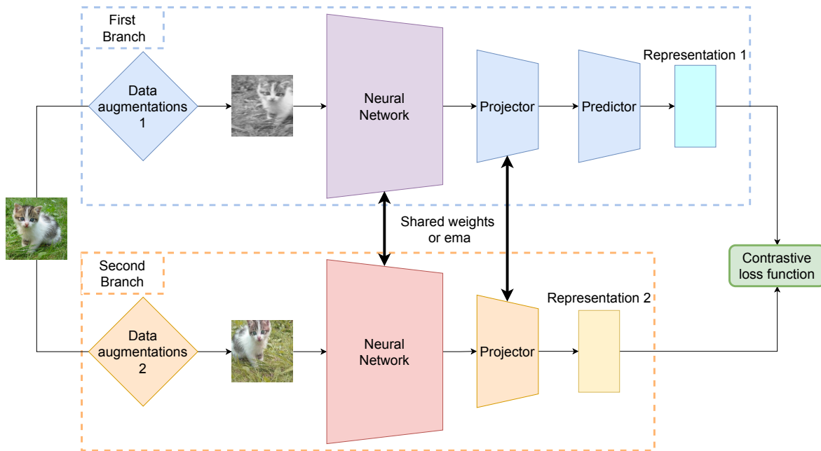
Figure 3.10: Siamese architecture to perform contrastive learning. An input goes through two branches that contain the same architecture: a data augmentation to form positive views, a neural network and a projector. Optionally the first branch can contain a predictor. Depending on the method, the second branch can share the same weights as the first branch or be updated by an Exponential Moving Average (ema) of the first branch. The contrastive loss function is applied to the output positive representations of both branches. The neural network of the first branch is kept at the end of training.
