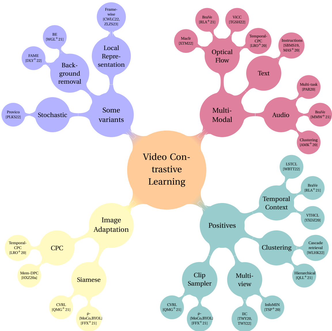
Figure 3.19: Overview of the general concepts and main methods for video contrastive learning.
