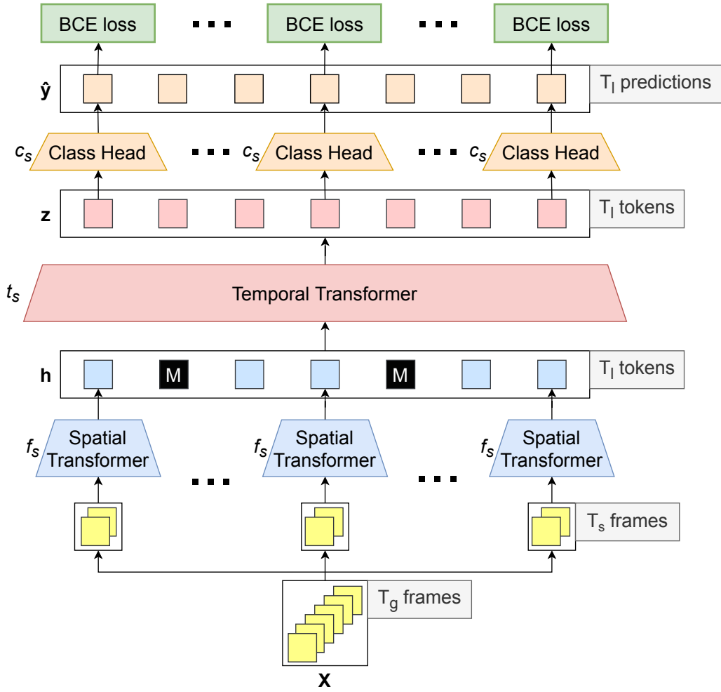
Figure 6.5: Fine-tuning to the action spotting task. Some spatial output tokens are masked.
