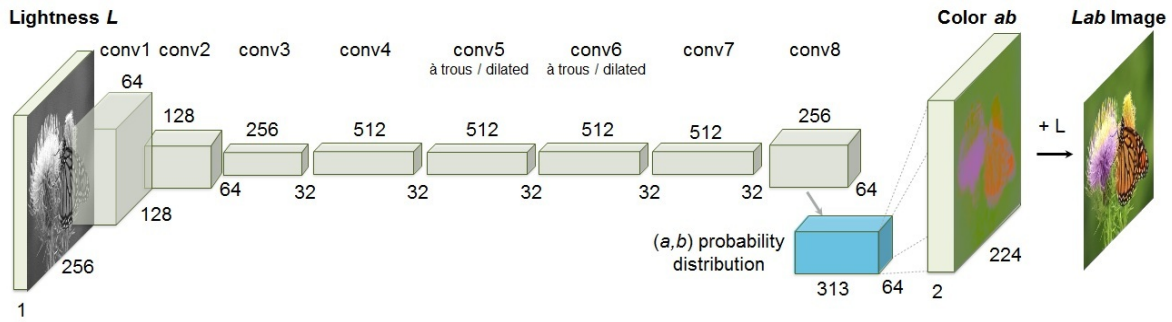
Figure 3.3: Illustration of colorization pretext task from [ZIE16].
