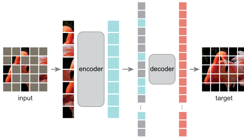
Figure 3.21: Illustration of MAE [HCX + 22] from its paper. Some patches are masked. The visible tokens pass through an encoder and its output is complemented by learnable mask tokens at the positions of masked patches. These tokens are fed to a decoder and The objective function is to predict the pixels of the original masked patches.
