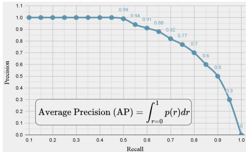
Figure 2.24: Precision given Recall from [Anw23]. AP is the area under the curve. Each point corresponds to a different threshold to consider predictions from 0 to 1.
