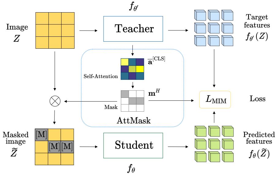
Figure 3.22: Illustration of high-attention teacher-guided masking from [KGP + 22].
