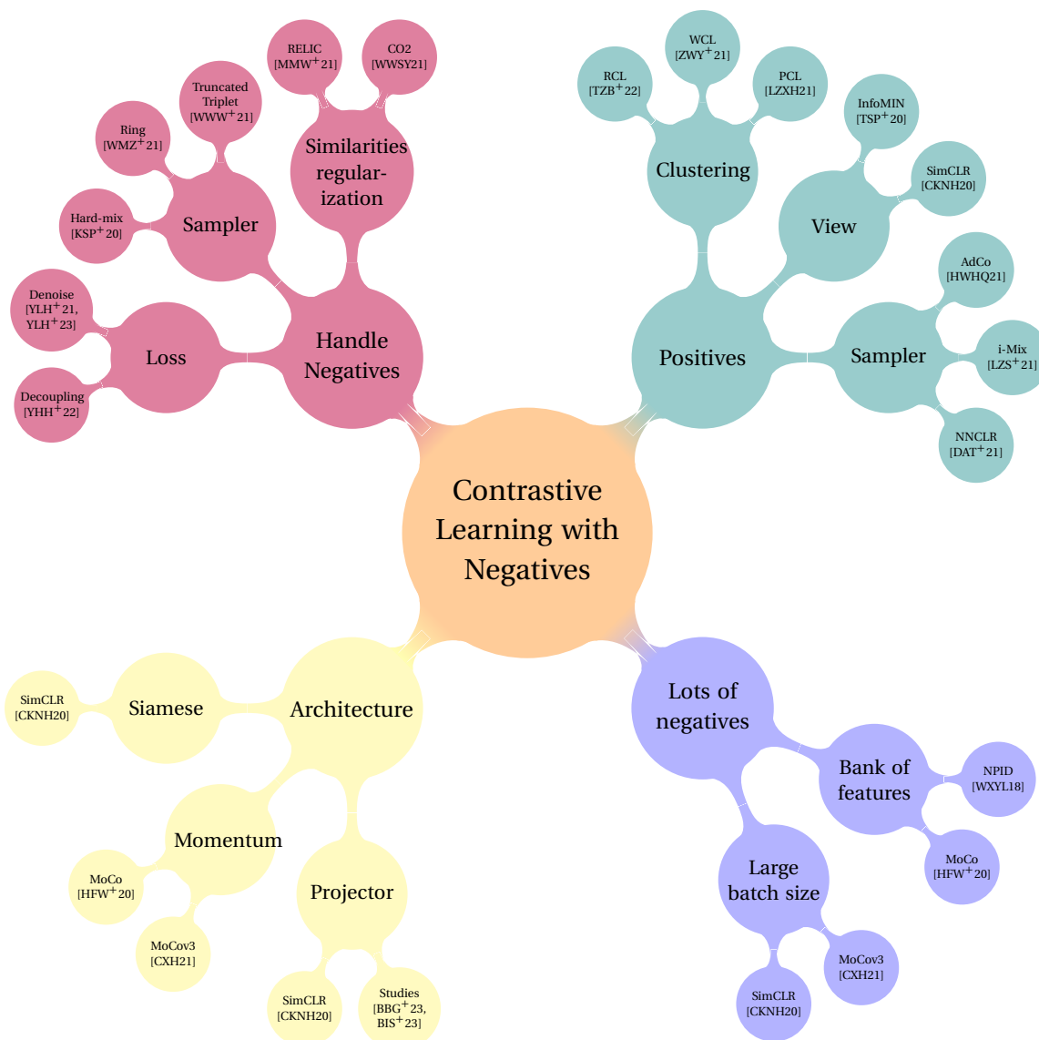
Figure 3.14: Overview of the general concepts and main methods for image contrastive learning using negatives.
