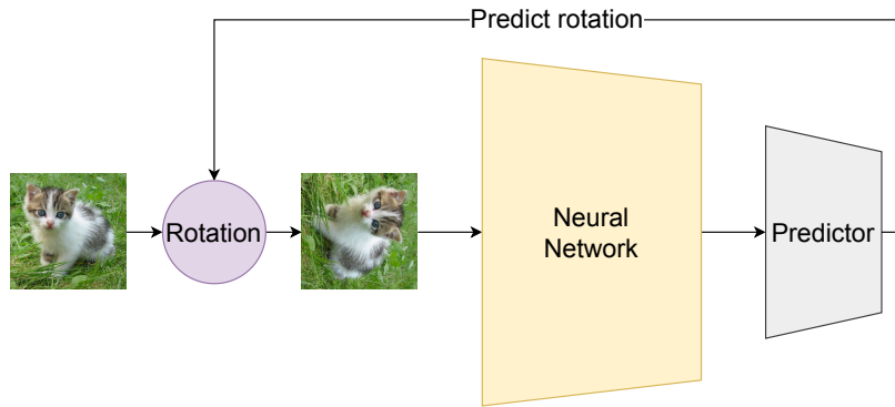
Figure 2.16: Rotation prediction pretext task. Input is rotated and the NN followed by a predictor seeks to predict the rotation applied.
