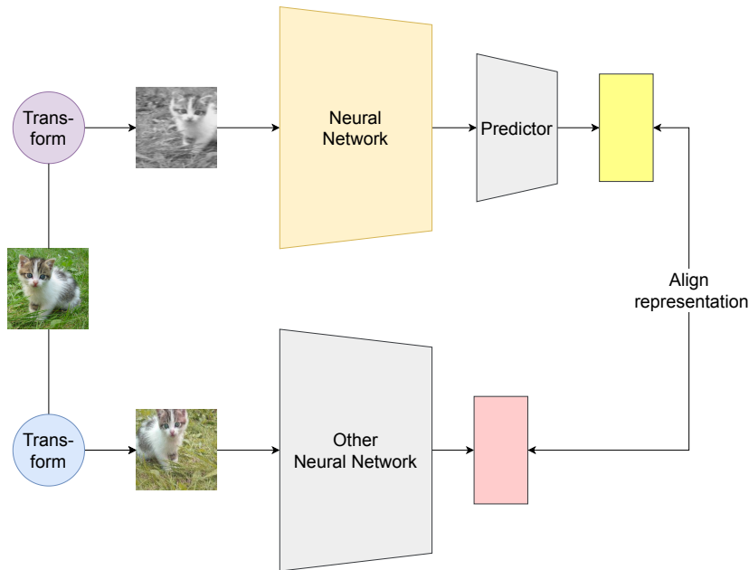
Figure 2.18: Instance discrimination CL. An image is augmented twice and passes through a Siamese NN architecture. The first branch contains the NN to pretrain and a predictor that seeks to predict the representation output of the NN in the second branch. The latter can have the same architecture and weights as the first branch or different.
