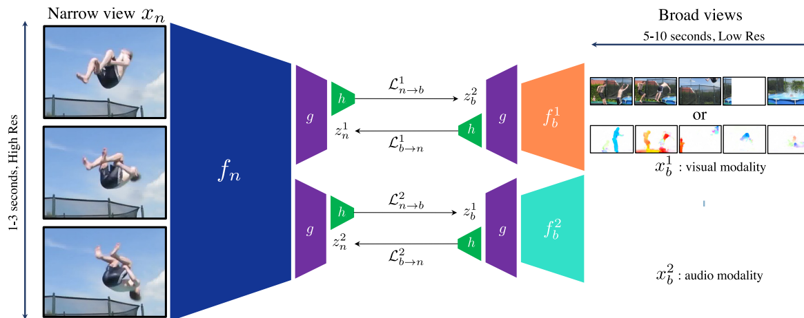
Figure 3.18: Illustration of BraVe from [RLA + 21]. Contrastive Learning is applied from an asymmetric pipeline via a high-resolution view with a narrow temporal context and a low-resolution view with a broad temporal context. It supports multi-modality.
