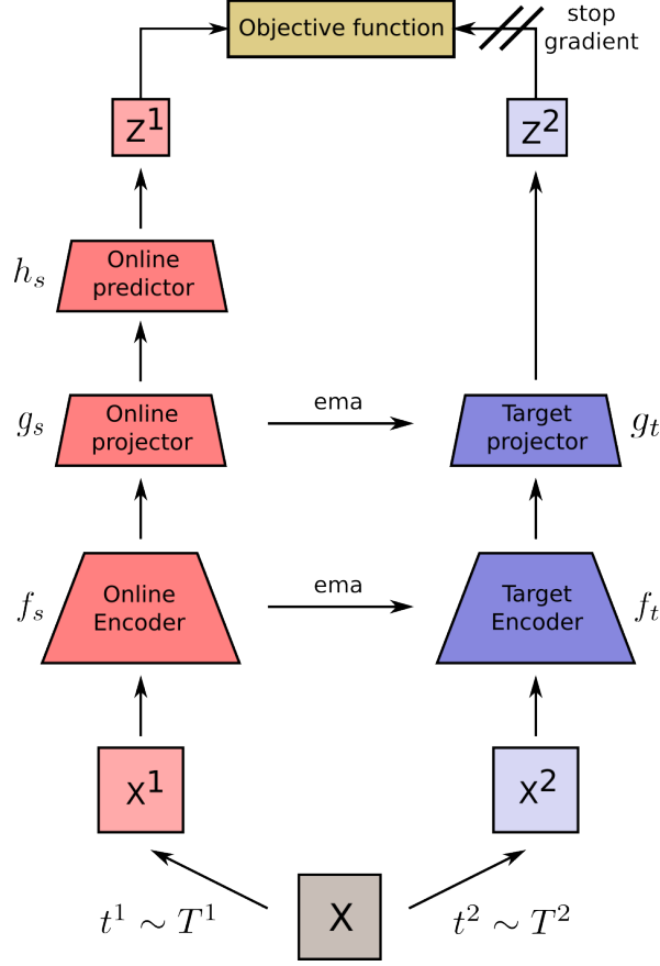
Figure 4.1: Illustration of the siamese pipeline shared by MoCov2 [CFGH20], ReSSL [ZYW + 21] and SCE. A batch \mathbf{x} of images is augmented with two different data augmentation distributions T^1 and T^2 to form \mathbf{x}^1 = t^1(\mathbf{x}) and \mathbf{x}^2 = t^2(\mathbf{x}) with t^1 \sim T^1 and t^2 \sim T^2 . The representation \mathbf{z}^1 is computed through an online encoder f_s , projector g_s and optionally a predictor h_s such as \mathbf{z}^1 = h_s(g_s(f_s(\mathbf{x}^1))) . A parallel target branch updated by an exponential moving average of the online branch, or ema , computes \mathbf{z}^2 = g_t(f_t(\mathbf{x}^2)) with f_t and g_t the target encoder and projector. The representations are passed to the objective function that is different for each method.
