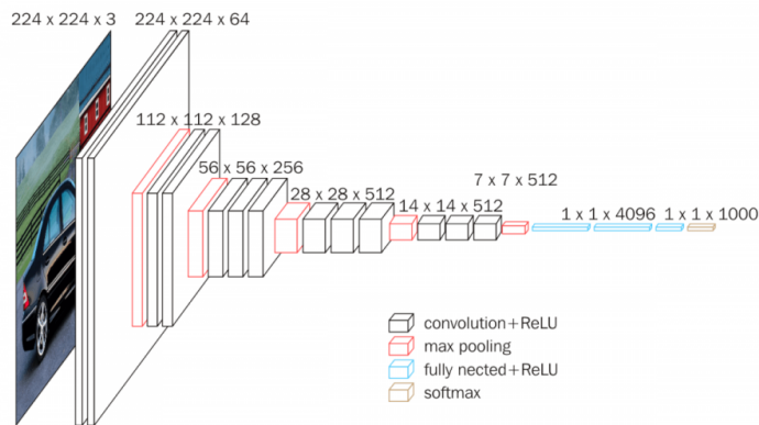
Figure 2.10: VGG [SZ15] architecture. Each block maintains a resolution.
