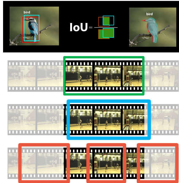
Figure 2.23: Detection examples for (up) a good bird object detection with high IOU with the ground truth from [ope23] (down) temporal action detection with green ground truth, blue good detection and red bad detections from [XZW + 17].
