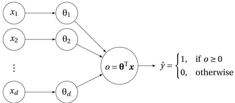
Figure 2.3: Perceptron with parameters \theta and the threshold 0 that receives \mathbf{x} as input.
