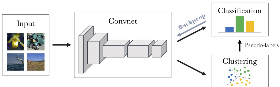
Figure 3.7: Illustration of Deep Cluster from [CBJD18]. Clusters are computed iteratively from the Neural Network image representations.
