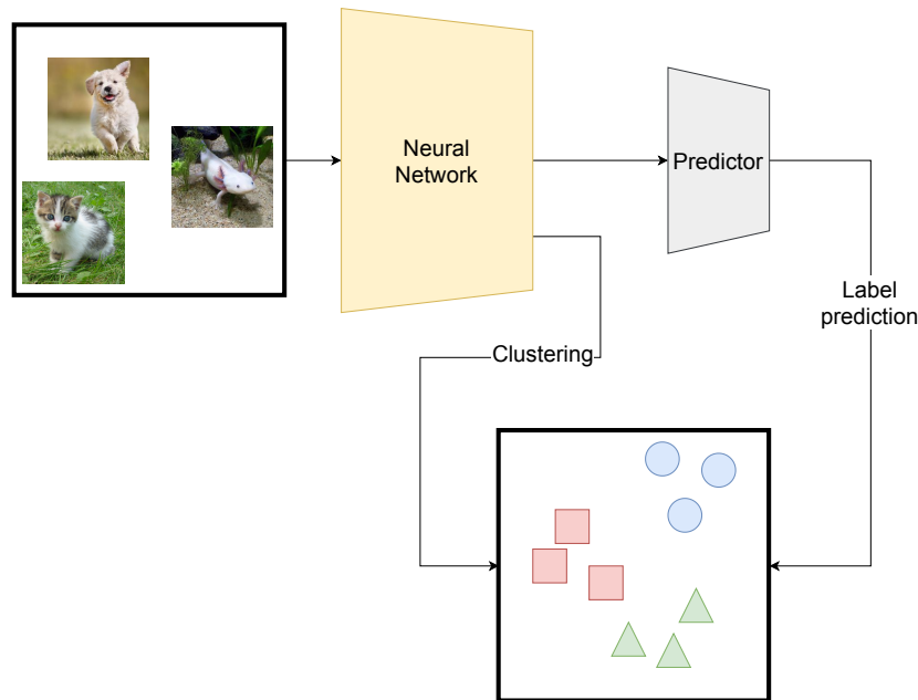
Figure 2.17: Clustering based on a NN representation from a dataset or a batch of data. The SSL task is to predict the pseudo-labels. The clustering can be performed once or multiple times throughout training.
