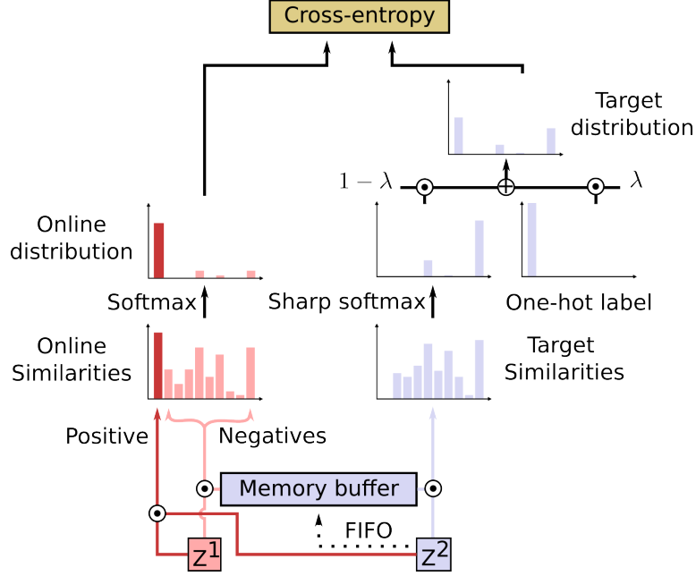
Figure 4.4: Objective function of SCE. The representations from the target branch \mathbf{z}^2 are used to compute the inter-instance target distribution by applying a sharp softmax to the cosine similarities between \mathbf{z}^2 and a memory buffer of representations from the momentum branch. This distribution is mixed via a 1 - \lambda factor with a one-hot label factor \lambda to form the target distribution. Online similarities between \mathbf{z}^1 and the memory buffer plus its positive in \mathbf{z}^2 are also computed. The online distribution is computed via softmax applied to the online similarities. The objective function is the cross entropy between the target and the online distributions.
