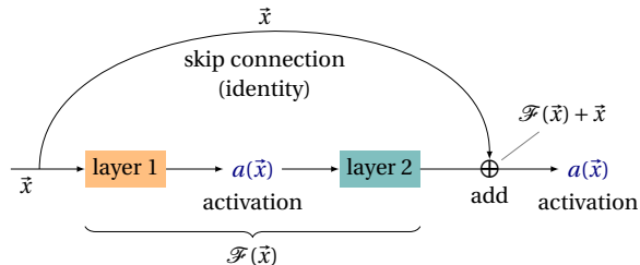
Figure 2.11: Residual connection [HZRS16].
