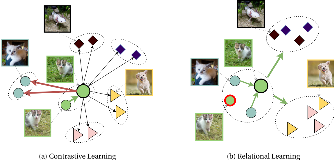
Figure 4.2: Illustration of (a) Contrastive Learning and (b) Relational Learning. Contrastive Learning correctly pushes negatives away and learns positive discriminative features but lacks modeling relations among instances. Relational Learning correctly models relations among instances but lacks discriminative positive features.
