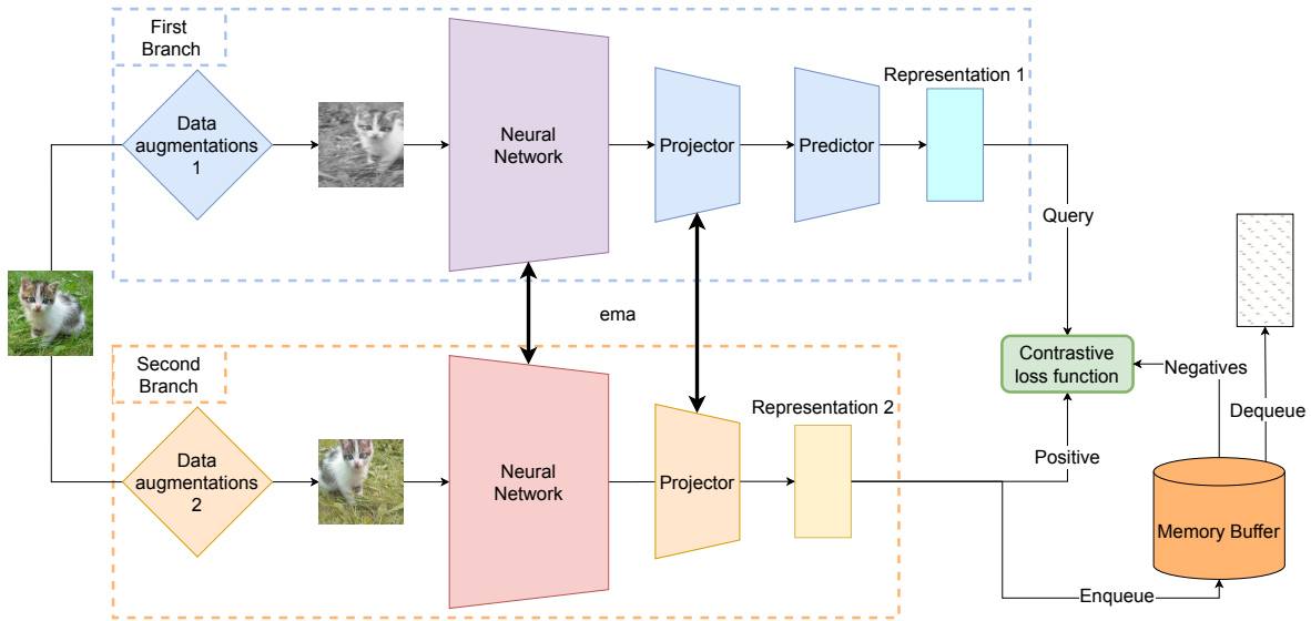
Figure 3.12: Siamese architecture to perform contrastive learning with a momentum memory buffer. It is the same architecture as in Fig. 3.10 with an Exponential Moving Average (ema) update for the second branch and its output of the second branch feeds a momentum memory via a First In First Out (FIFO) update. The momentum memory buffer serves as a collection of negatives for the contrastive loss.
