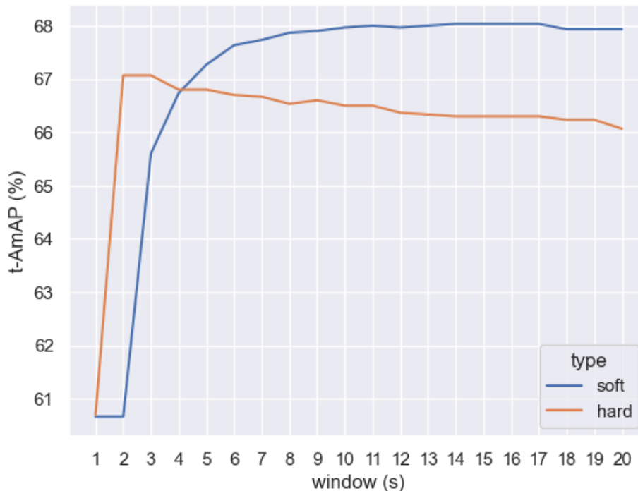
Figure C.1: Influence of the soft and hard NMS and its window size in second on the t-AmAP.
