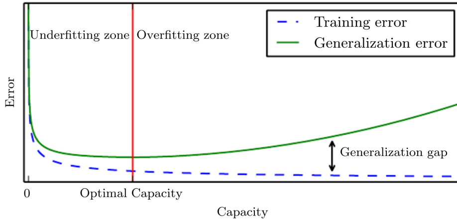
Figure 2.4: Relationship between capacity and error illustrated by [GBC16]. Underfitting happens when the model has low capacity so it cannot fit properly training data and has both high training and generalization error, the latter estimated on a testing set. Overfitting happens when the model has too much capacity that leads to learning irrelevant training features that minimize training error but increase generalization error causing a wide generalization gap .
