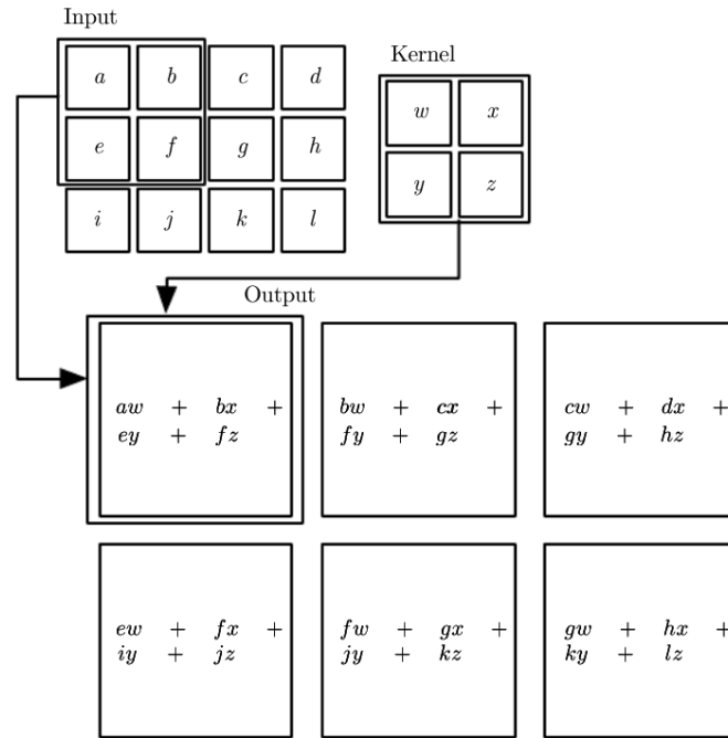
Figure 2.6: Cross-correlations of a 3 \times 4 input with a 2 \times 2 kernel. Figure from [GBC16].
