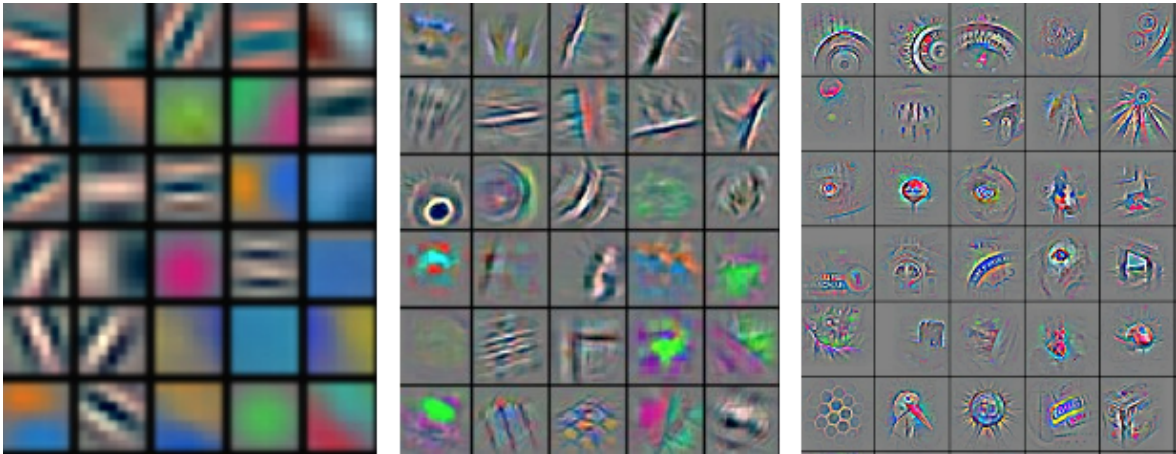
Figure 2.7: Filters learned by successive convolutional layers by AlexNet [KSH12].
