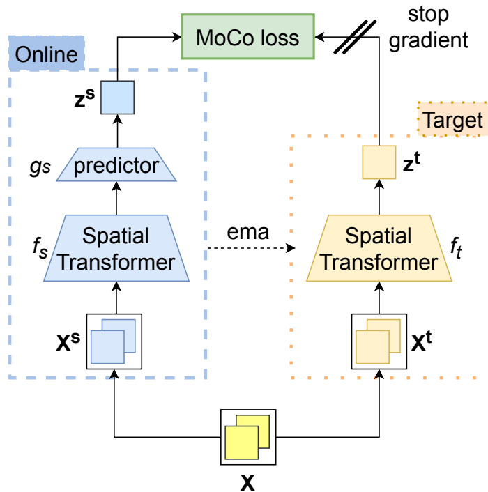
Figure 6.3: Pretraining of the spatial transformer.
