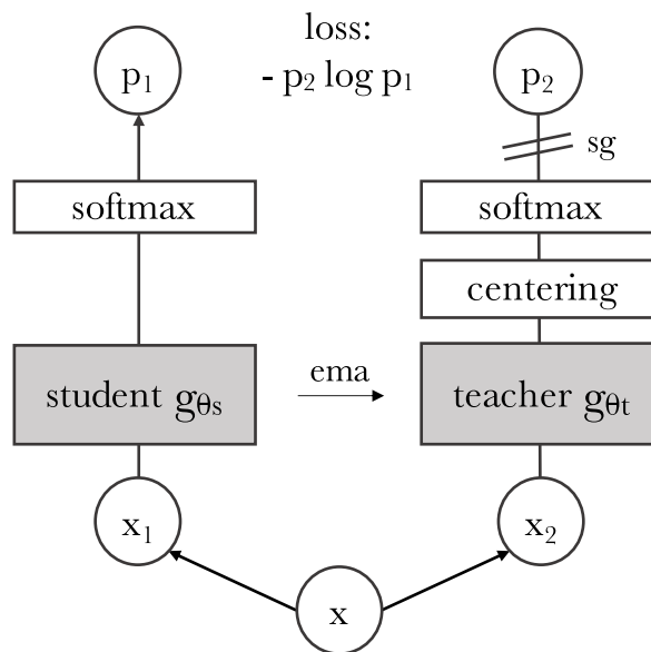
Figure 3.16: Illustration of DINO from [CTM + 21]. The target branch produces a soft prediction over a set of pseudo-classes regularized by centering to avoid collapses. The student branch seeks to predict the target distribution.
