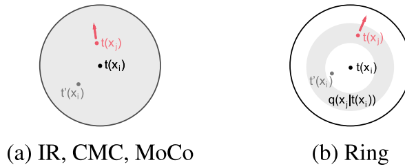
Figure 3.13: Illustration from [WMZ + 21] to compare (a) standard contrastive learning negative sampler and (b) Ring negative sampler [WMZ + 21]. In black the representation of an example x_i , in gray the representation of its positive and in red the representation of its negative. The gray area is the support of the distribution to sample negatives. Ring only considers negatives further away from the query than its positive and closer than a margin whilst standard contrastive learning does not have a constraint.
