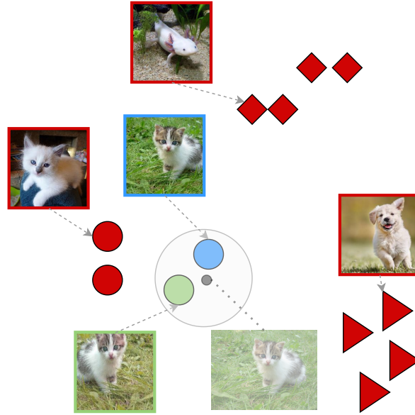
Figure 3.9: Illustration of a query cat (blue circle), its positive (green circle) which is the same cat as the query after some data augmentations, and all the negatives (red shapes). Because there are no labels, even highly similar images are considered as negatives.
