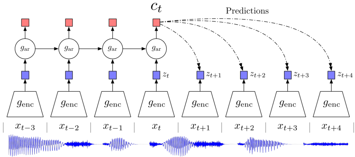
Figure 3.8: From [vdOLV18], a context is built from representations of input data. The generated context is used to predict the future representation and contrasted with negative representations from other instances.
