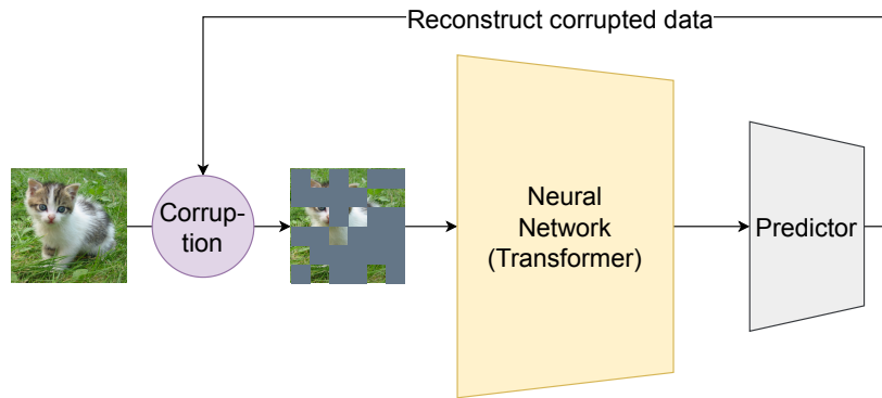
Figure 2.19: Input data is corrupted by masking part of it. The SSL task is to reconstruct the missing parts.
