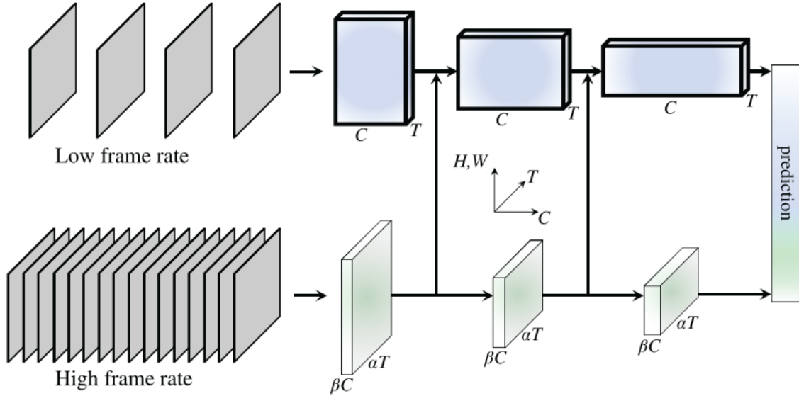
Figure 2.12: SlowFast architecture, from [FFMH19]. The slow path receives a low frame rate video and has wide convolutions while the fast path receives the same video at a fast frame rate with shallow convolutions. The predictions of both paths are fused at their output and the fast path distills motion information in the slow path at different depths.
