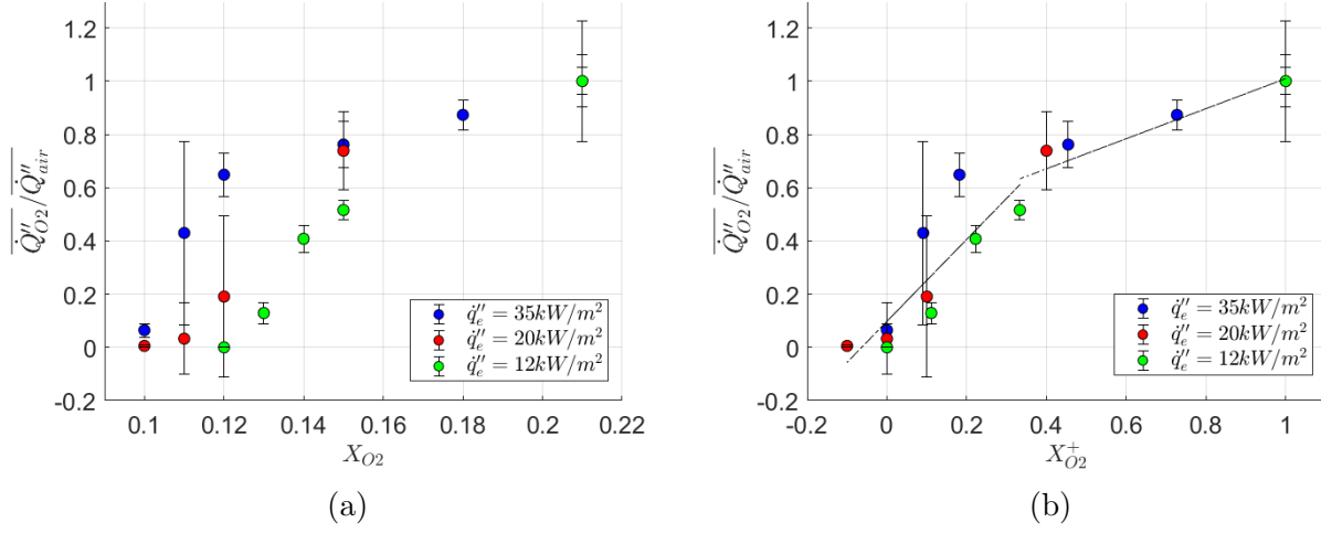
Figure 4.33: a) Ratio \frac{\overline{\dot{Q}_{O_2}''}}{\overline{\dot{Q}_{air}''}} for different external heat flux against X_{O_2} . b) Ratio \frac{\overline{\dot{Q}_{O_2}''}}{\overline{\dot{Q}_{air}''}} for different external heat flux against X_{O_2}^+ .
