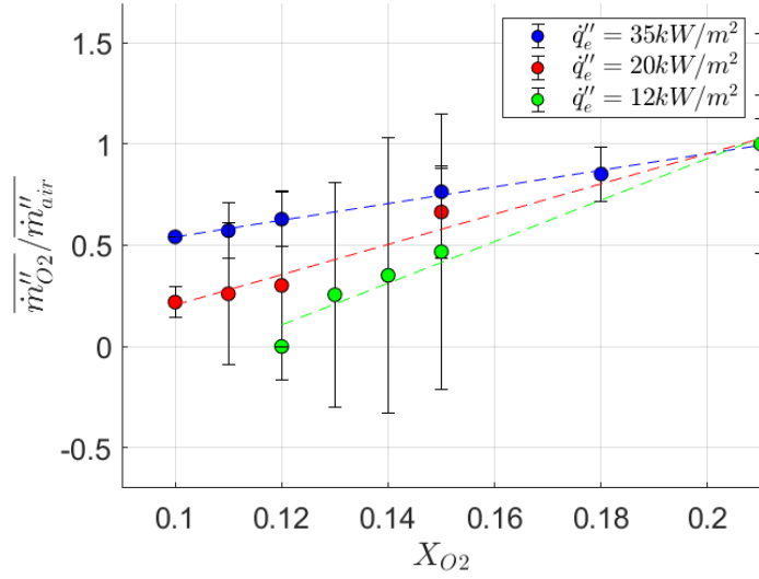
Figure 4.18: Ratio \frac{\overline{\dot{m}''_{O_2}}}{\overline{\dot{m}''_{air}}} for several oxygen concentrations and external heat fluxes.
