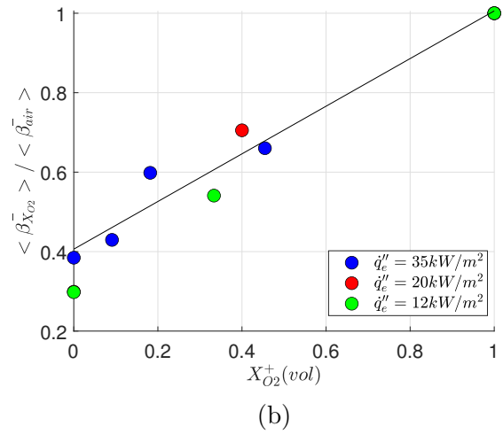
Figure 4.24: a) Ratio \frac{\langle \bar{\beta}_{O_2} \rangle}{\langle \bar{\beta}_{air} \rangle} against X_{O_2} . b) Ratio \frac{\langle \bar{\beta}_{O_2} \rangle}{\langle \bar{\beta}_{air} \rangle} against X_{O_2}^+
