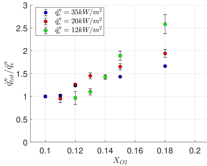
Figure 4.27: Ratio of \dot{q}_{tot}'' to \dot{q}_e'' for different oxygen concentrations and external heat fluxes
