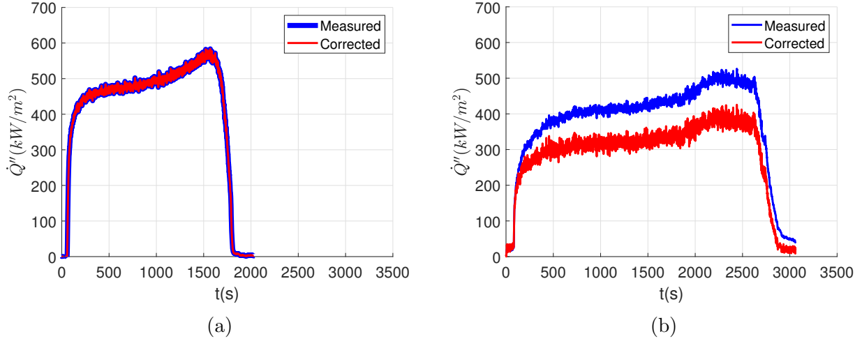
Figure 2.4: Illustration of the measured and corrected heat release rate per unit surface with a) under air and b) under vitiated atmosphere
