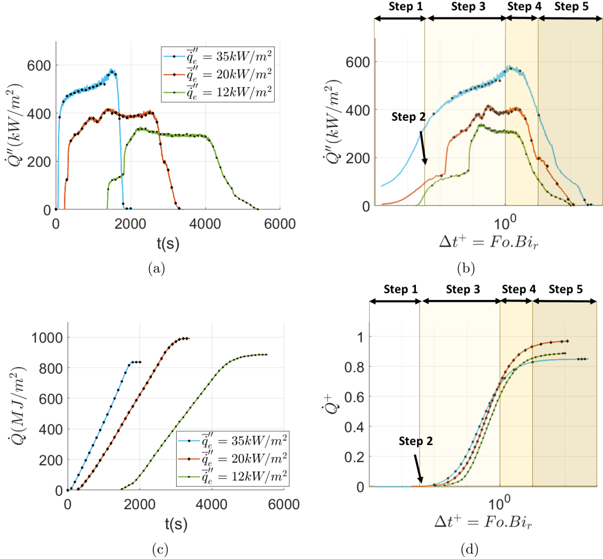
Figure 3.5: a) Heat release rate \dot{Q}'' with respect to time under air for several external heat fluxes. b) Heat release rate \dot{Q}'' with respect to t^+ under air for several external heat fluxes. c) Total heat release \dot{Q} with respect to time under air for several external heat fluxes. d) Dimensionless total heat release \dot{Q}^+ with respect to t^+ under air for several external heat fluxes.
