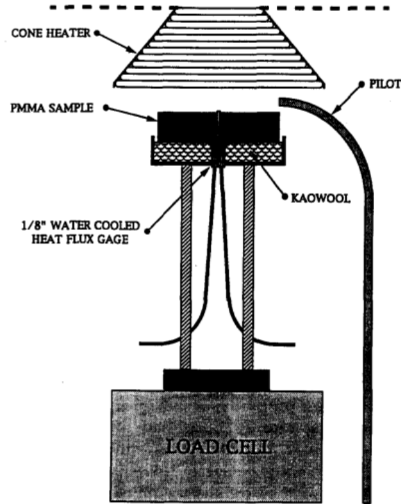
Figure 1.3: Apparatus used in reference [28].
