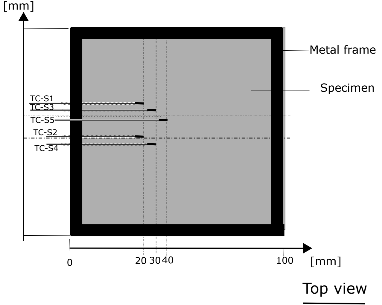
Figure 2.9: Top view of the disposition of the in-sample thermocouples
