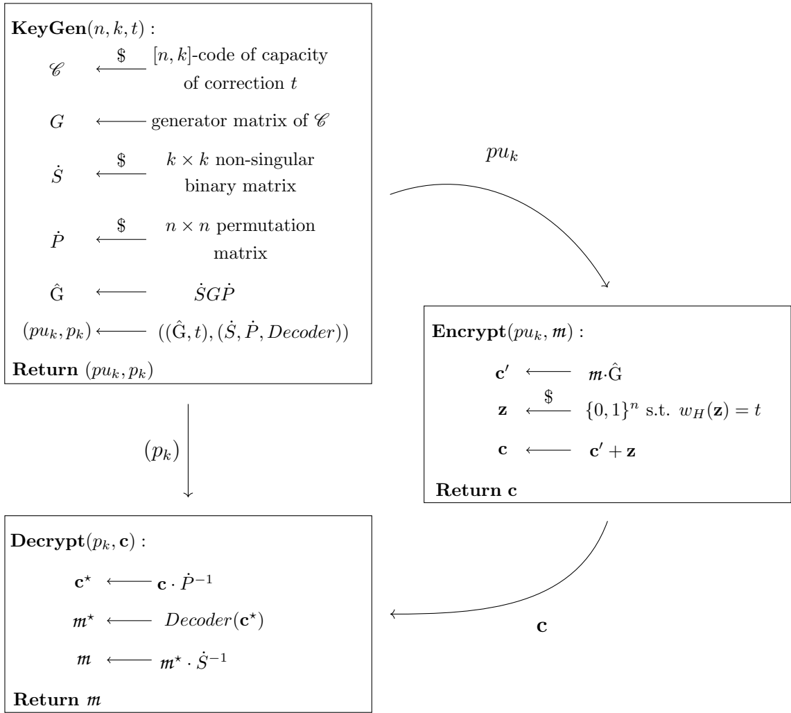
Figure 2.5: McEliece public-key encryption
