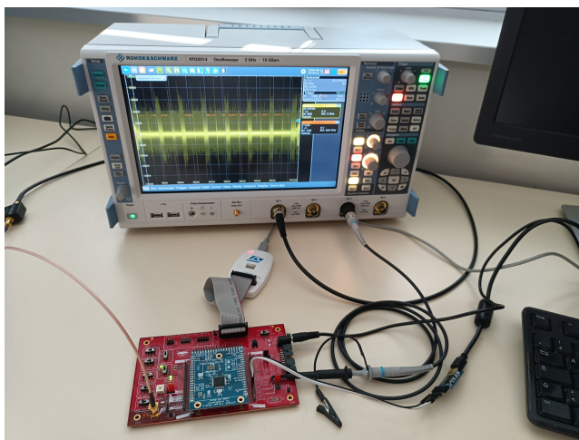
Figure 5.1: Setup for power analysis attacks on the Cortex-M4.
