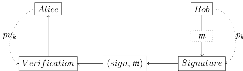
Figure 1.4: Digital signature.
