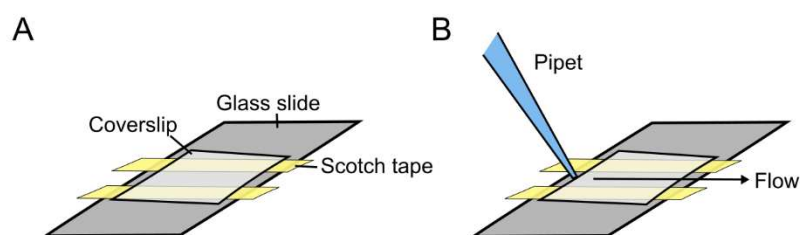
Figure 2.5 Flow chambers. A) Flow chambers were constructed from a glass slide, double sided scotch tape and a coverslip. B) Samples were applied on one side of the chamber and aspirated through the chamber by use of a tissue (not shown in the scheme).
