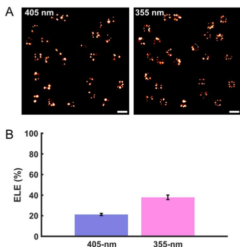
Figure 8. Simulated cryo-SMLM of rsEGFP2-labeled Nup96 in NPCs. (A) Reconstructed images using 355 or 405 nm illumination. (B) Effective labeling efficiency (ELE) using 355 nm or 405 nm illumination. ELE was extracted from the analysis of 100 NPCs (Figure S19), and error bars were derived by bootstrapping. Scale bar: 0.5 \mu\text{m} .
