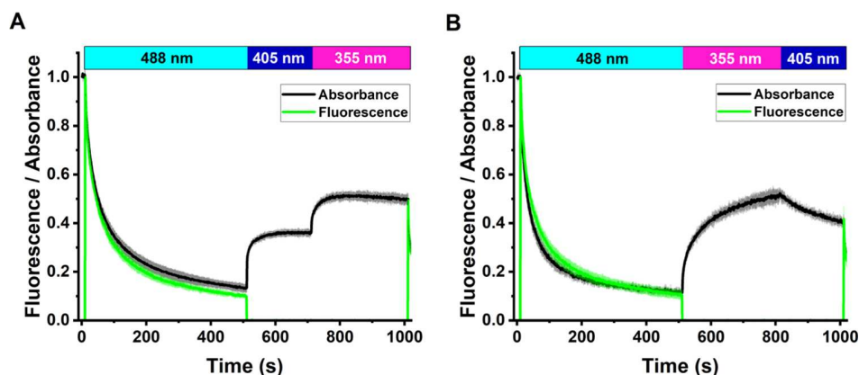
Figure 3. Recovery of rsEGFP2 on-state by subsequent illumination with 405 and 355 nm light. Absorbance and fluorescence levels are calculated by integration of the absorption and fluorescence emission spectra in 470–500 and 495–630 nm spectral ranges, respectively. (A) Recovery by 405 nm light followed by 355 nm light. (B) Recovery by 355 nm light followed by 405 nm light. Absorbance (gray) and fluorescence (green) evolutions are measured at 110 K by illumination at 488 (0.4 kW/cm 2 ), 405 (0.3 kW/cm 2 ), and 355 nm (0.025 kW/cm 2 ), according to the schemes indicated in the upper bars. Absorbance and fluorescence are normalized to 1 at start of acquisition. Fluorescence was only measured in the presence of 488 nm light. The mean \pm s.d. of n = 3 measurements is shown.
