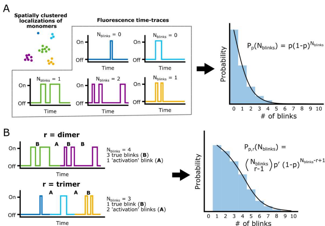
Figure 1.24 Molecular counting by blinking statistics. A) The the probability of a fluorophore to blink ( 1-p ) can be determined by analysis of the blinking histogram of the monomeric fluorophore. B) Knowing p , the unknown stoichiometry ( r ) of a complex can be estimated from the blinking histogram of the complex. Note that for oligomers the blinking histogram is right shifted by r-1 because the activation of each fluorophore, except the first fluorophore of the complex, results in a 'fake' blink (activation blink). This model assumes a 100% effective labelling efficiency (PCE + labelling efficiency + detection efficiency). More sophisticated models can handle incomplete labelling, complicated photophysical models and mixtures of oligomeric states as referenced in the text.
