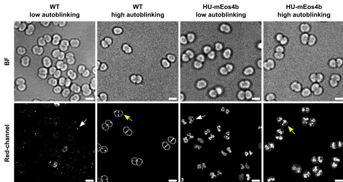
Figure 2.7 Autoblinking of Deinococcus radiodurans . PALM data of WT and HU-mEos4b labeled DR cells were collected under standard imaging conditions (see below, 40,000-60,000 frames). Autoblinking levels were highly variable between samples, but could be controlled, to some extent, by washing the cells in M9DR medium prior to imaging. Autoblinking sometimes appeared as isolated clusters of localizations (white arrows) and sometimes as a smooth staining of the cell membrane (yellow arrows). Scale bar = 2 \mu m.
