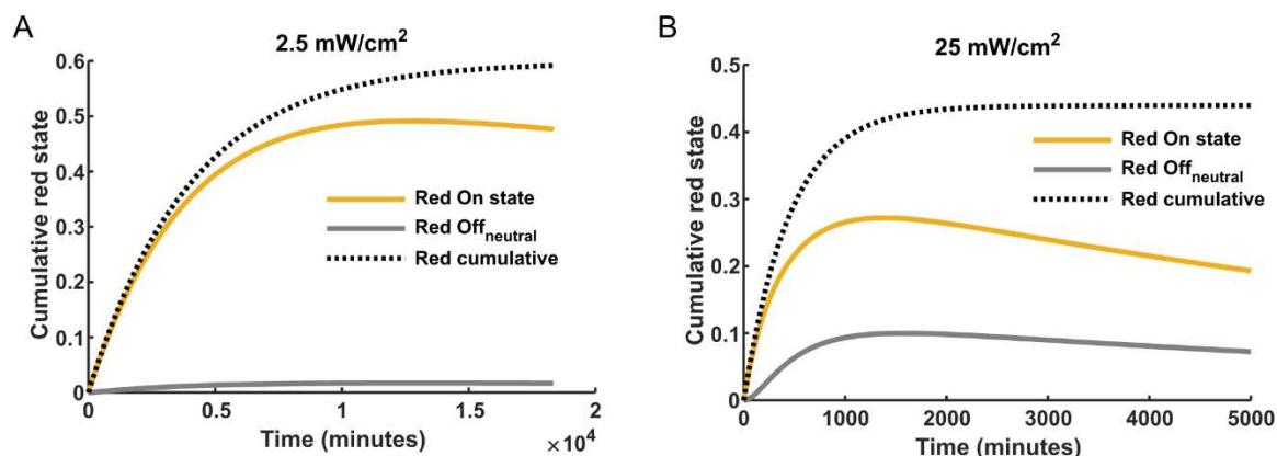
Supplementary Figure 7. Formation of Off neutral affects estimation of the PCE. Photoconversion was simulated under continuous illumination with 405 nm light at 2.5 mW/cm 2 (A) and 25 mW/cm 2 (B). Shown are the progressions of the cumulative red state (black dotted curves), the red On state (yellow curves) and the Off neutral state (grey curves).
