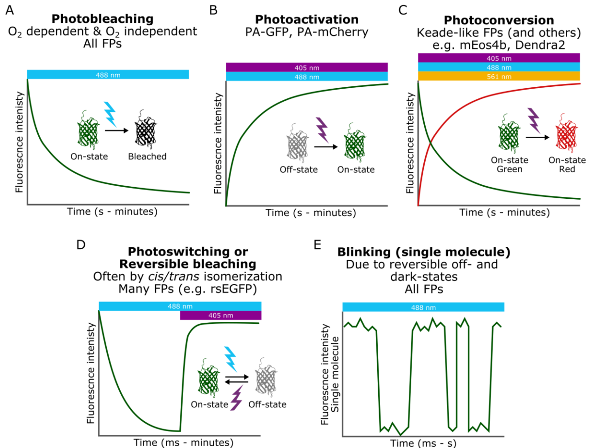
Figure 1.9 Common phototransformations of FPs. A) All FPs are susceptible to irreversible photobleaching, which may proceed via O 2 dependent or independent mechanisms. B) Photoactivation is the irreversible conversion of FPs from a non- or weakly-fluorescent state into a fluorescent state. Typical examples are PAGFP and PAmCherry, which are activated by 405 nm light. C) Photoconversion is the light induced change in absorption and emission spectra of a FP. Typical examples are Keade-like FPs, such as mEos4b and Dendra2, which convert from a green emitting into a red emitting state upon excitation with 405 nm light. D) Photoswitching or reversible bleaching is the reversible loss of fluorescence, often by cis/trans isomerization of the chromophore. The fluorescent on-state can typically be recovered by excitation of the off-state with blue-shifted light. E) The formation of transient dark states (photoswitching/reversible photobleaching) gives rise to blinking at the ms to s time scale. Figure inspired by 86 .
