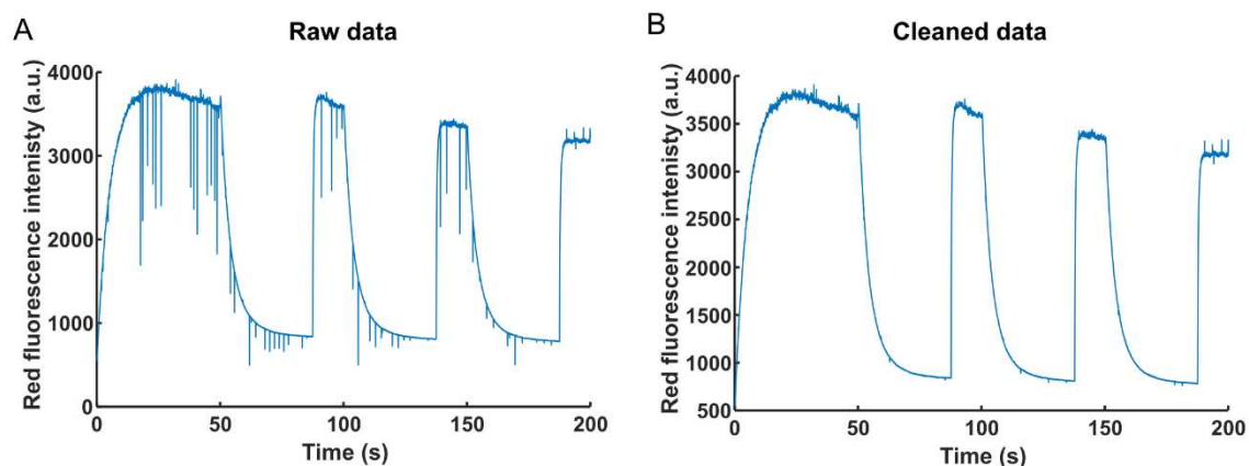
Figure 2.16 Cleaning of the ensemble fluorescence data. A) Raw data of a red state photoswitching experiment at pH 8. B) The same data after replacement of erroneous low intensity values.
