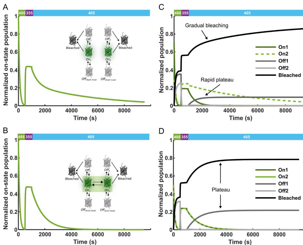
Figure 3.52 Comparison of the switching behavior of rsEGFP2 at CT without and with fast exchange between On1 and On2. Simulations of rsEGFP2 photoswitching under sequential illumination with 488 nm ( 400 \text{ W/cm}^2 ), 355 nm ( 25 \text{ W/cm}^2 ) and 405 nm ( 300 \text{ W/cm}^2 ) light as in Figure 3.50C . Switching was simulations assuming no exchange (A and C) or fast exchange (B and D) between On1 and On2. The progression of the total on-state population (On1 + On2) is shown in A and B. C and D show the progressions of the individual states.
