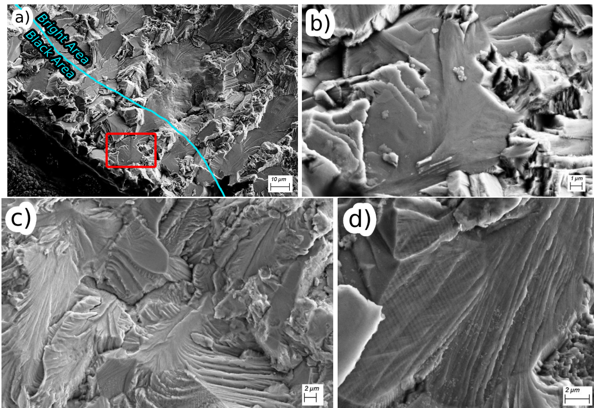
Figure 4.4 | SEM detailed views of the Black Area and the Bright Area of a crack fracture surface which propagated in a specimen with a chimney (Specimen nb 48 cycled at 300 MPa during 5.04 \times 10^5 cycles). (a) zoom on the Black Area with crystallographic aspect located in the red rectangle of Figure 4.3a. The blue curve separates the Bright Area and the Black Area which is very narrow. (b) detailed view of a facet in the Black Area located in the red rectangle of (a). (c) zoom on the Bright Area with planar features. (d) detailed view of a planar feature from the Bright Area showing extensive striations. (c) and (d) are located in the yellow rectangle of Figure 4.3a.
