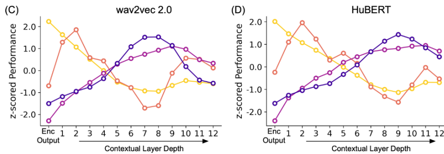
(b) Probing by layer of speech units in Self-Supervised Audio Embeddings. Source: [Vaidya et al., 2022].
