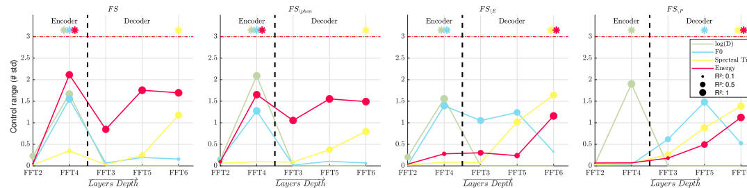
(d) Controllability of supra-segmental features for FastSpeech2 variants
