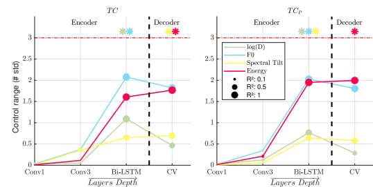
(c) Controllability of supra-segmental features for Tacotron2 variants
