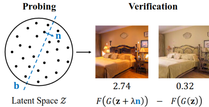
(a) Causal Control of lighting in closed room with GAN network. Source: [Yang et al., 2021].
