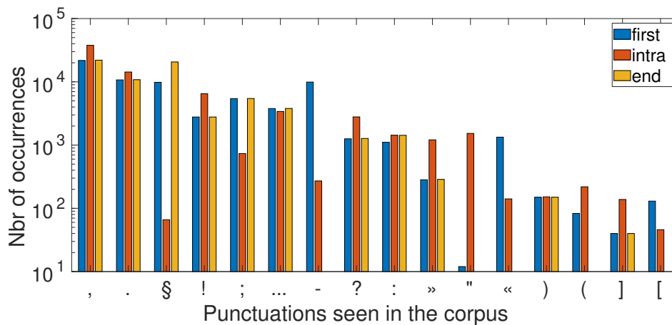
Figure 3.3: Counts of first, intra and ending punctuation marks in the new segmentation of the NEB corpus.
