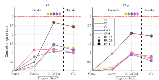
(a) Controllability of segmental features for Tacotron2 variants
