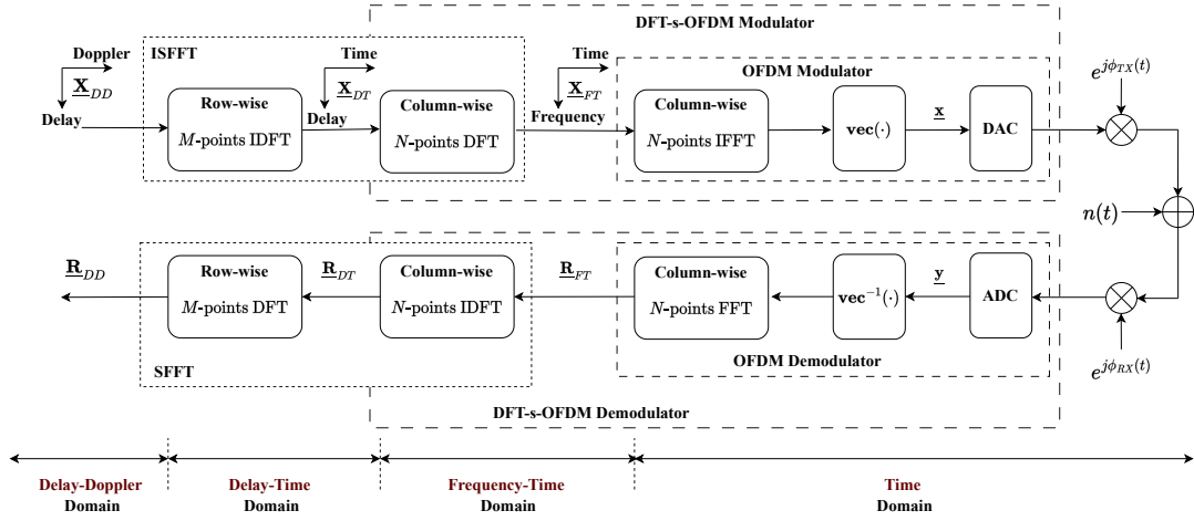
Figure 2.10: OTFS system model
