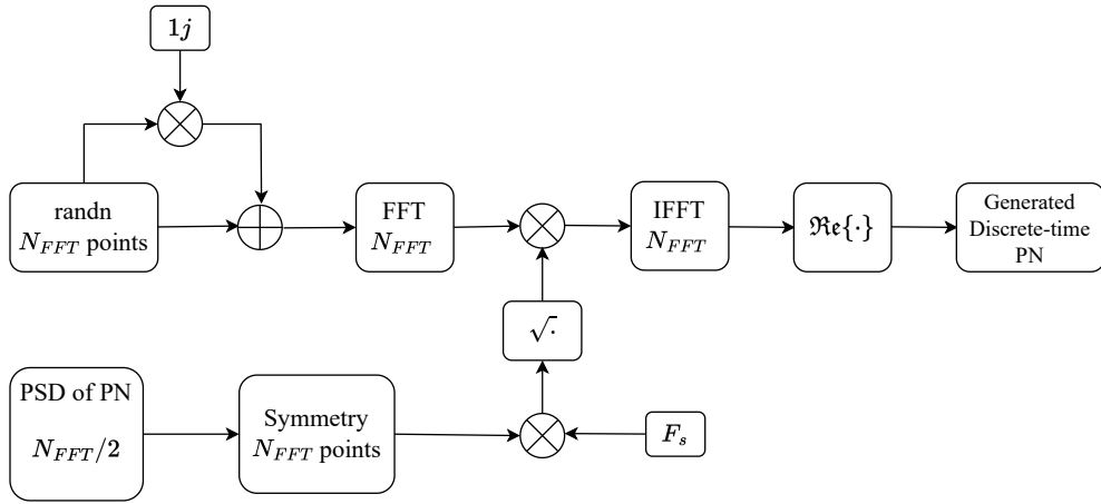
Figure 2.6: Discrete-time PN generation method.
