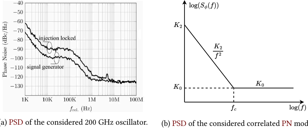
Figure 2.1: PSD Models
