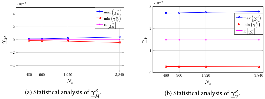
Figure 5.6: Statistical analysis of \gamma_k using Second configuration
