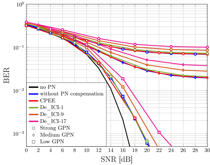
Figure 5.11: OFDM performance: BER in function of the SNR for a 16-QAM, N_s=480 and N_f=512 .
