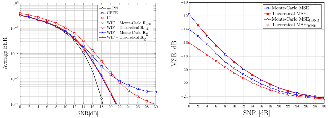
(a) Uncoded BER performance of a SC system. We use a 16-QAM modulation with the insertion of 16 pilots per block, considering blocks of size N_{sb} = 1024 .
