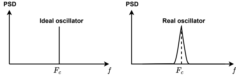
Figure 1.3: Power Spectral Density (PSD) of Ideal vs. Real oscillator response
