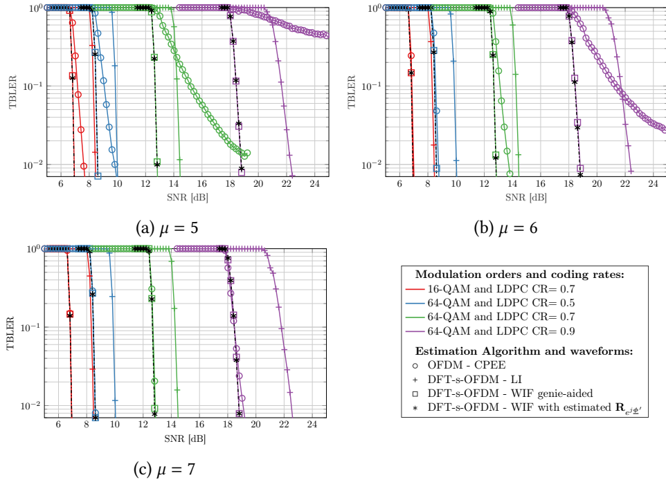
Figure 3.7: Performance of DFT-s-OFDM and OFDM systems in terms of TBLER as a function of SNR. The numerologies \mu = \{5, 6, 7\} and the measured PN in Section 2.2.3 are considered.
