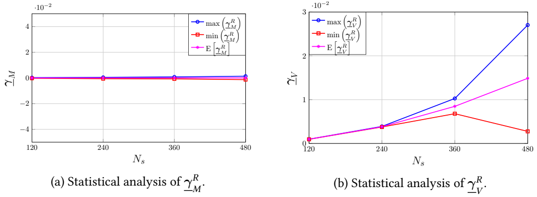
Figure 5.5: Statistical analysis of \gamma_k using First configuration
