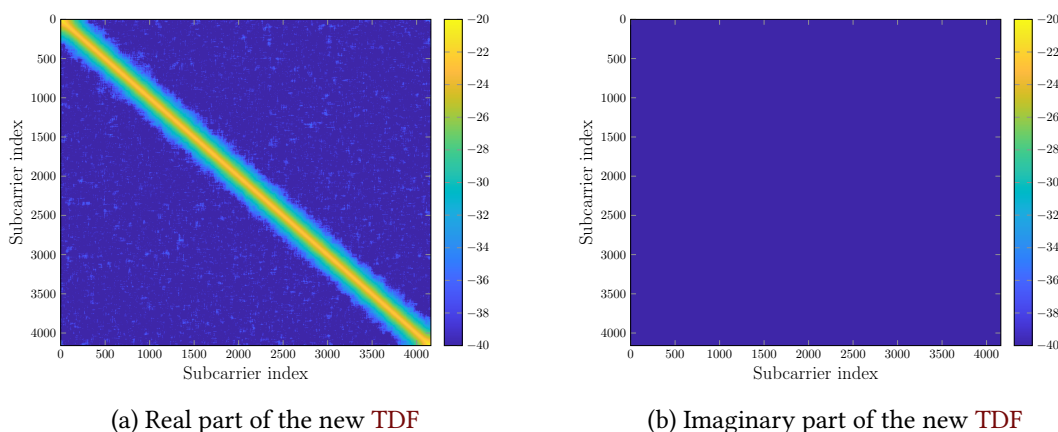
Figure 4.11: Illustration of the power of new TDF coefficients in [dB].
