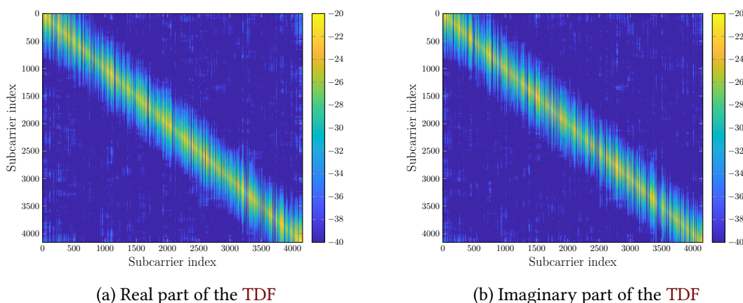
Figure 4.10: Illustration of the power of TDF coefficients in [dB].
