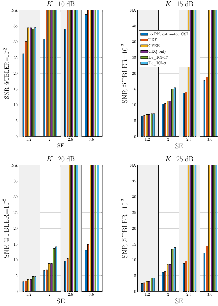
Figure 4.5: SNR [dB] values to achieve a TBLE of 10^{-2} as a function of the SE for F_c=140 GHz. 16-QAM modulation scheme is considered and different values of K are considered. "NA" stands for "Non Achievable".
