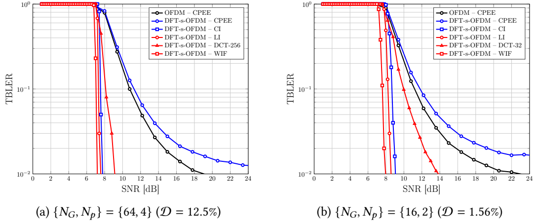
Figure 3.4: Performance comparison between OFDM and DFT-s-OFDM assuming contiguous PT-RS pattern. The 3GPP PN model 2 in Section 2.2.2 is considered.
