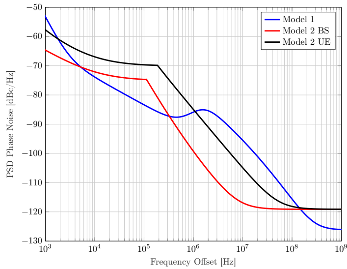
Figure 2.2: Proposed 3GPP PN Models for a 140 GHz carrier frequency
