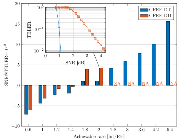
Fig. 4: Comparison of the two PN compensating strategies at 140 GHz for numerology \mu = 8 . NA stands for Not Achievable.
