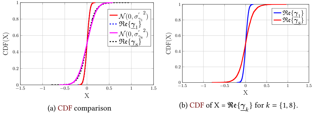
Figure 5.7: CDF of \Re\{\underline{\gamma}_k\}
