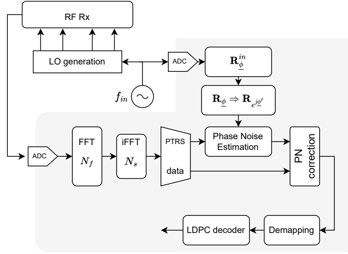
Figure 3.5: Block diagram of the proposed digital baseband receiver for DFT-s-OFDM.
