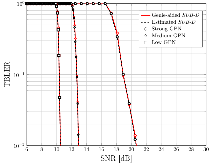
Figure 5.10: DFT-s-OFDM performance: estimated SUB-D vs. genie-aided SUB-D assuming a 16-QAM modulation, N_s = 480 , N_f = 512 and CR=0.7 .
