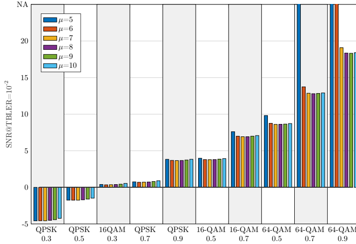
Figure 3.6: SNR [dB] values to achieve a TBLEP of 10^{-2} in OFDM system. We consider the measured PN in Section 2.2.3, several numerologies and a pilot density of 6%. "NA" stands for "Non achievable".
