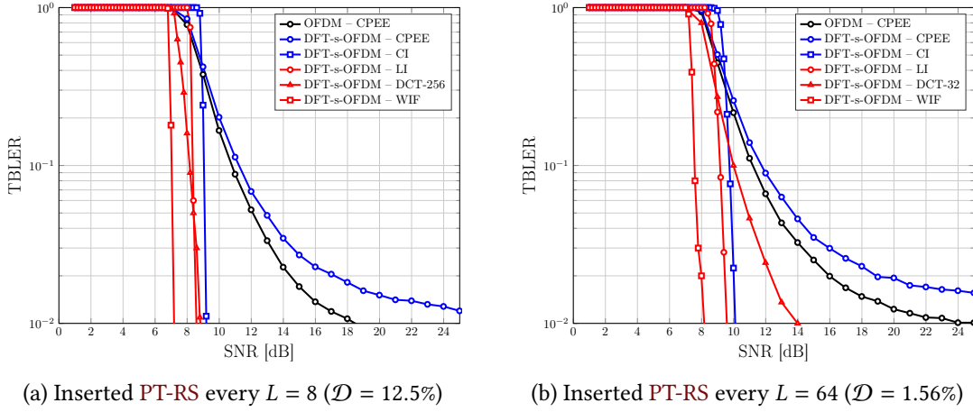
Figure 3.3: Performance comparison between OFDM and DFT-s-OFDM assuming distributed PT-RS pattern. The 3GPP PN model 2 in Section 2.2.2 is considered.
