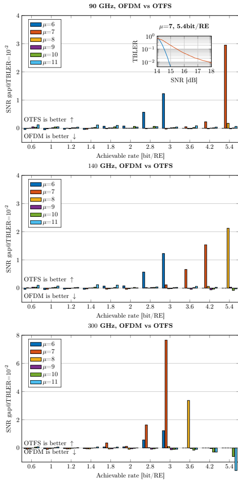
Fig. 5: Comparison of OFDM and OTFS. CPEE in the DT domain is considered for OTFS.
