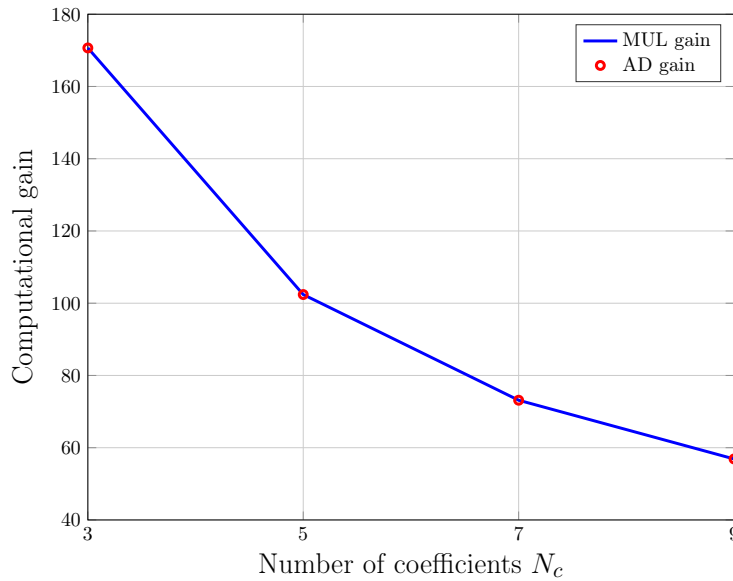
Figure 3.10: Computational gain of the low complexity WIF .
