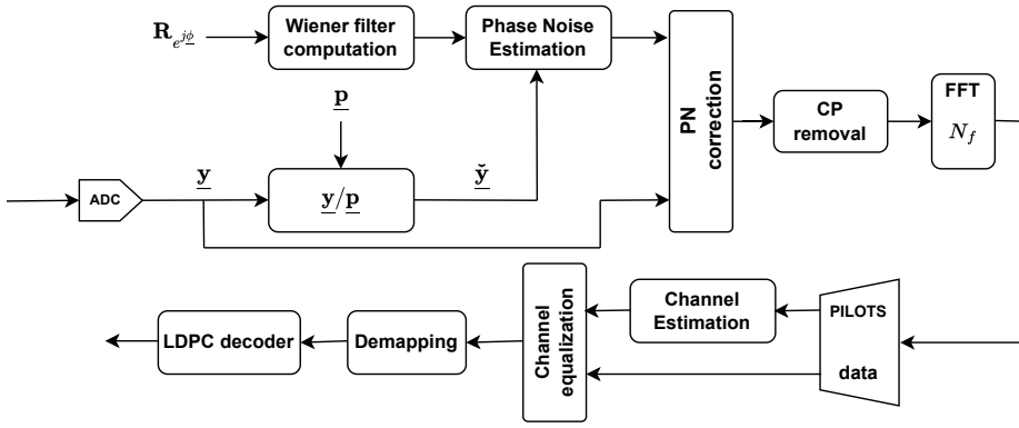
Figure 4.7: New block diagram of the receiver
