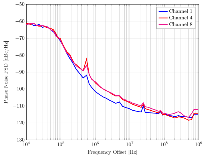
Figure 2.4: Measured PSD for channels 1, 4 and 8 for a 140 GHz carrier frequency.
