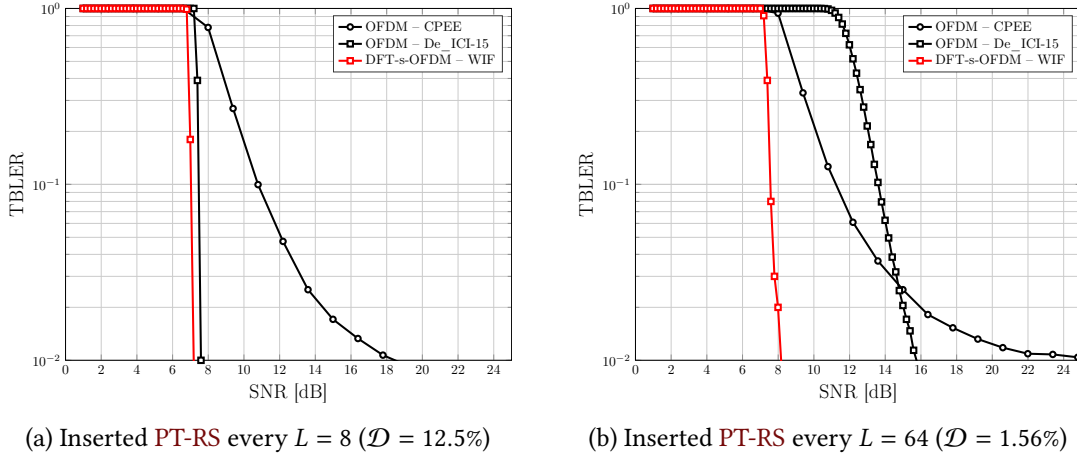
Figure 4.4: Performance comparison between OFDM and DFT-s-OFDM.
