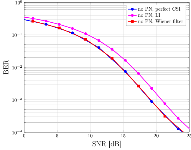
Figure 4.2: Uncoded BER as a function of SNR. Rician channel with K = 15 dB and 16-QAM are considered. The other simulation parameters are depicted in Table 4.1
