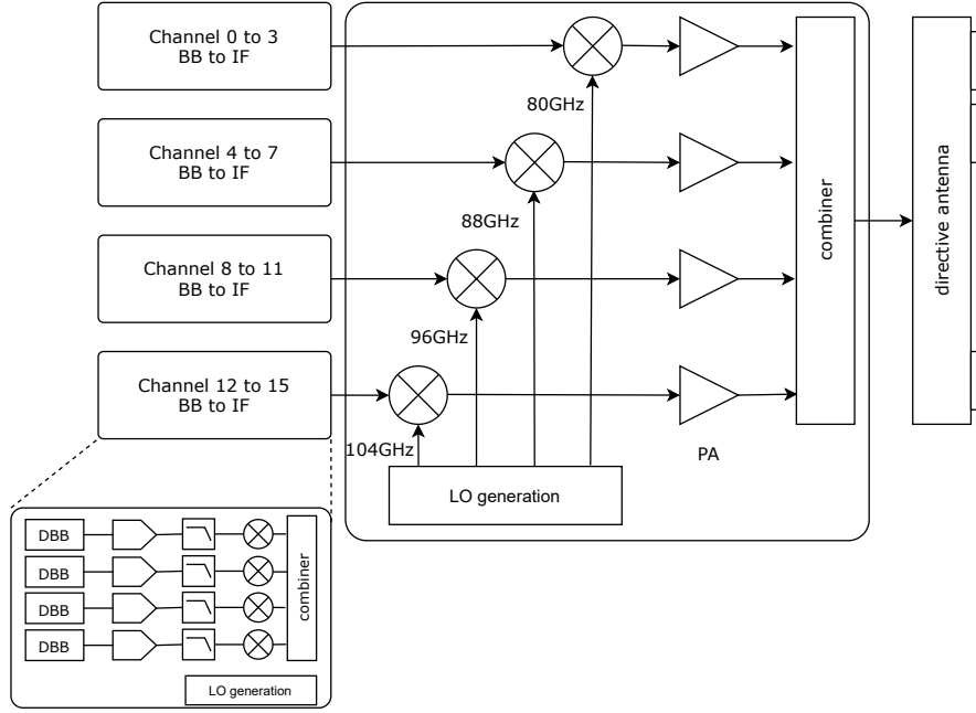
Figure 2.3: D-Band Transceiver architecture
