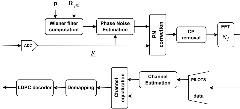
Figure 4.3: Block diagram of the receiver
