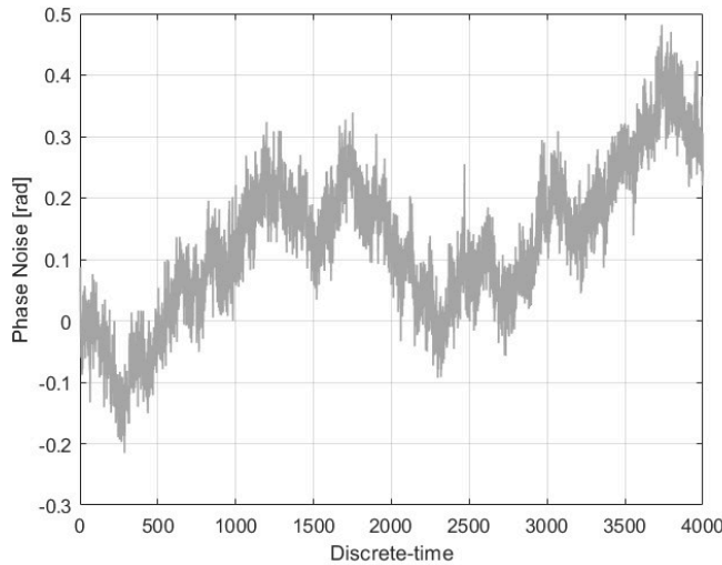
Figure 3.1: Discrete-time PN
