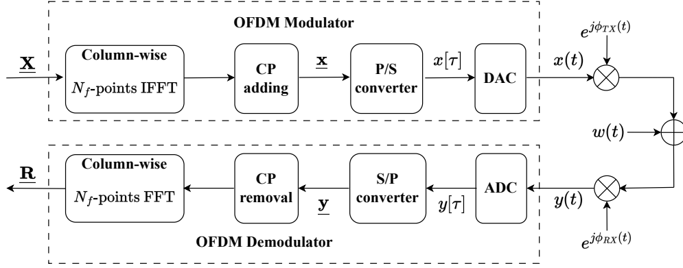
Figure 2.8: OFDM system model
