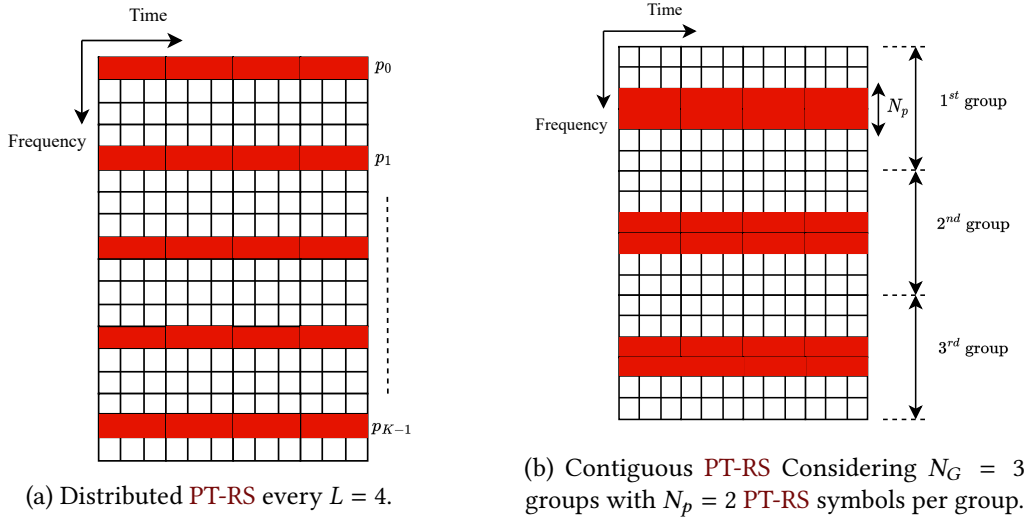
Figure 3.2: PT-RS Pattern
