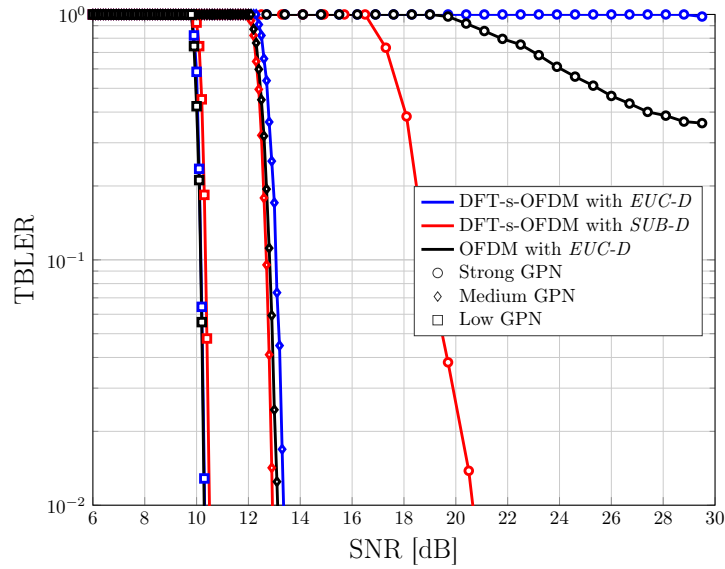
Figure 5.9: OFDM vs DFT-s-OFDM performance: TBLEER in function of the SNR for a 16-QAM modulation with N_s = 480 , N_f = 512 and CR=0.7 .
