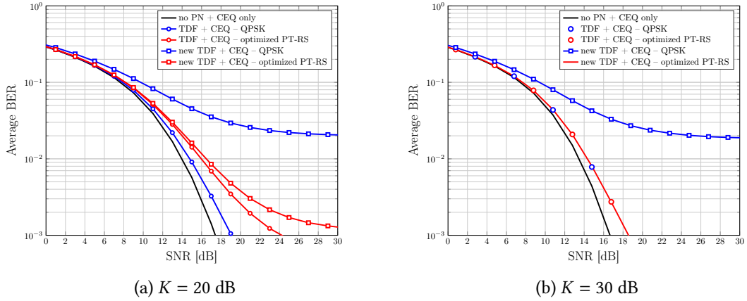
Figure 4.8: OFDM system performance with \mathcal{D} = 25\% .
