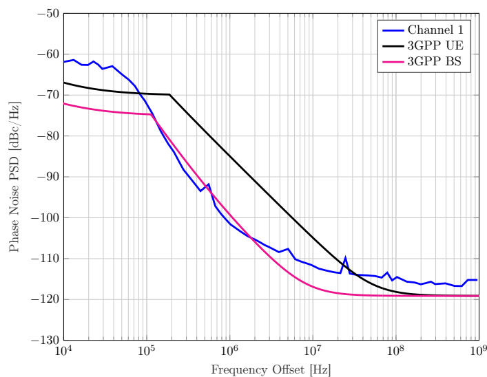
Figure 2.5: Measured PSD for channel 1 vs. 3GPP Models UE and BS for a 140 GHz carrier frequency.
