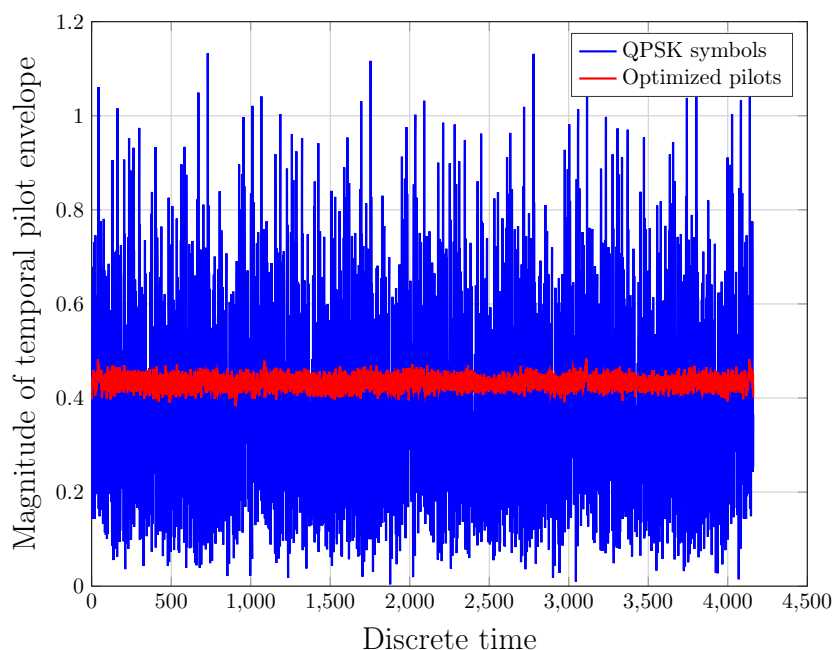
Figure 4.6: QPSK vs. optimized PT-RS symbols
