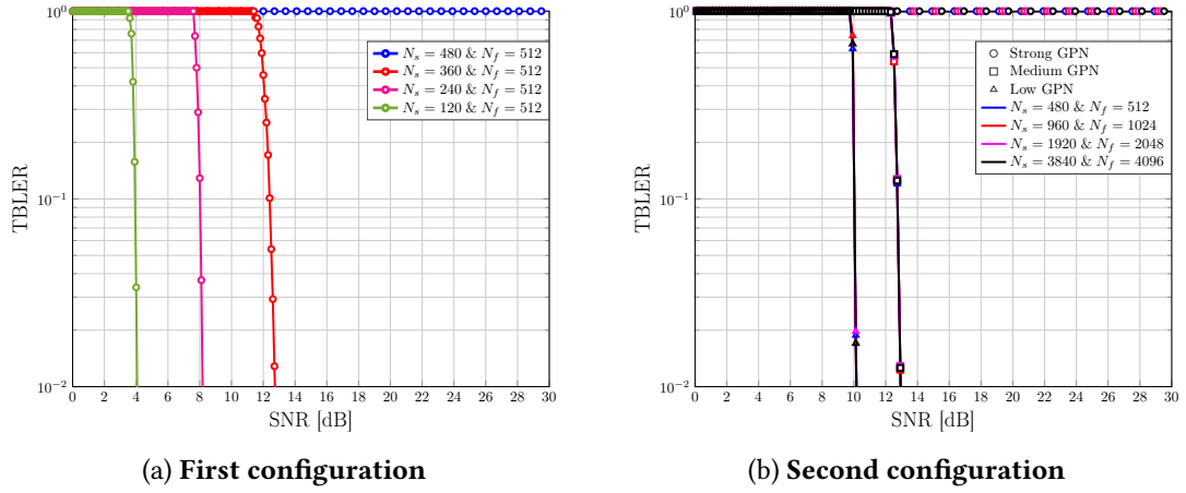
Figure 5.8: DFT-s-OFDM system performance
