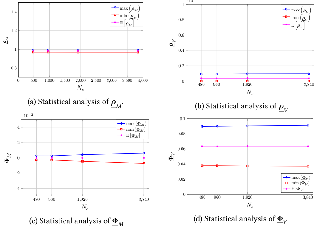
Figure 5.3: Statistical analysis of \rho_k and \Phi_k using the Second configuration
