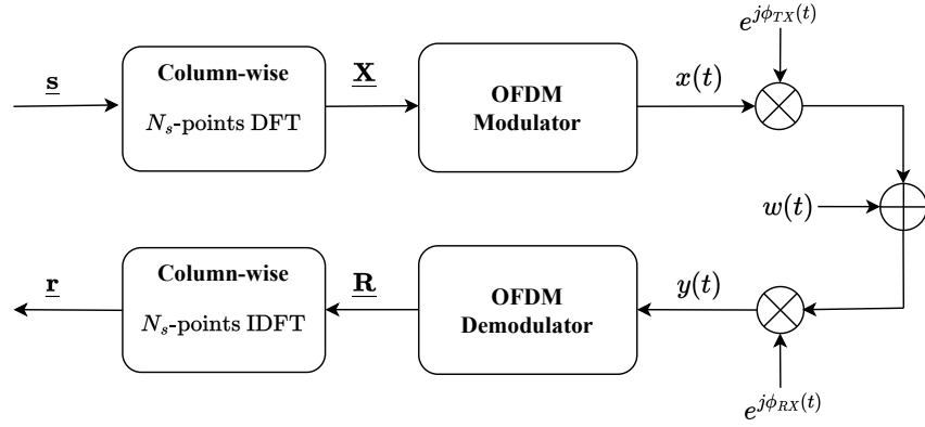
Figure 2.9: DFT-s-OFDM system model
