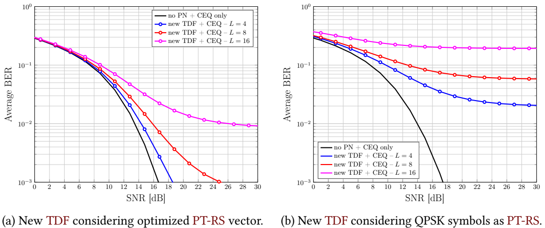
Figure 4.9: OFDM system performance with new TDF in (4.27) for different pilot density and a K -factor of 30 dB
