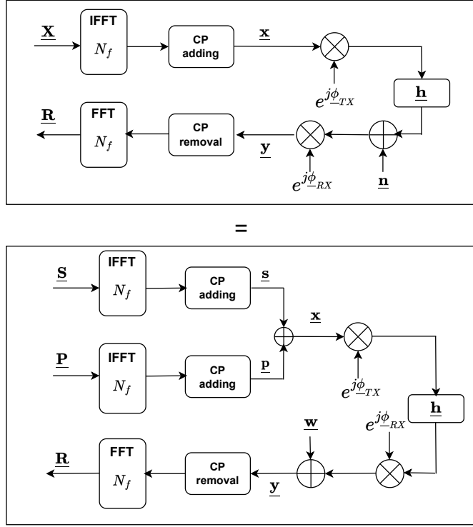
Figure 4.1: OFDM system model
