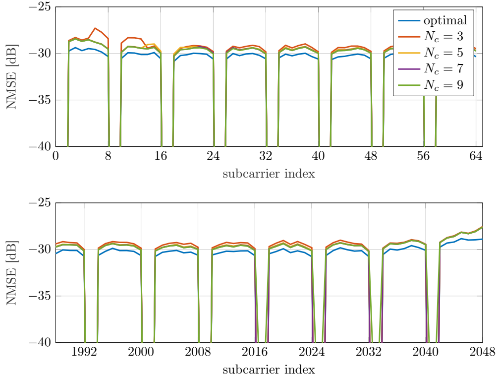
Figure 3.9: NMSE between the low complexity WIF and the optimal WIF.
