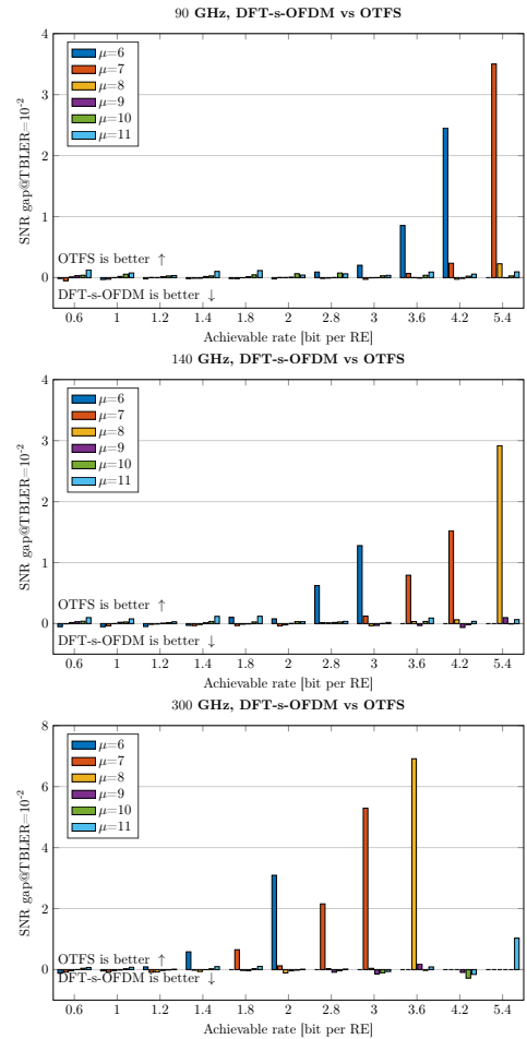
Fig. 6: Comparison of DFT-s-OFDM and OTFS. CPEE in the DT domain is considered for OTFS.
