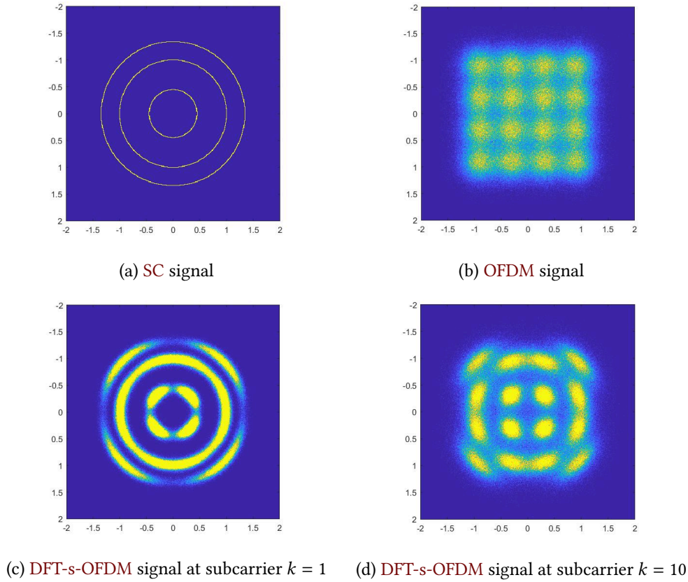
Figure 5.1: GPN distortion on 16-QAM modulated signal with SNR = 50 dB
