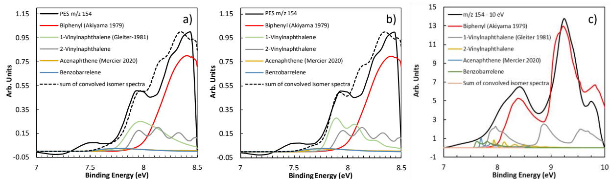
Figure 5-30. Comparison of experimental, reference and convolved isomer photoelectron spectra for m/z 154. a) using literature PES for 1-vinylnaphthalene and at 8.5 eV, b) using calculated PES for 1-vinylnaphthalene and at 8.5 eV, c) using literature PES for 1-vinylnaphthalene and at 10 eV.
