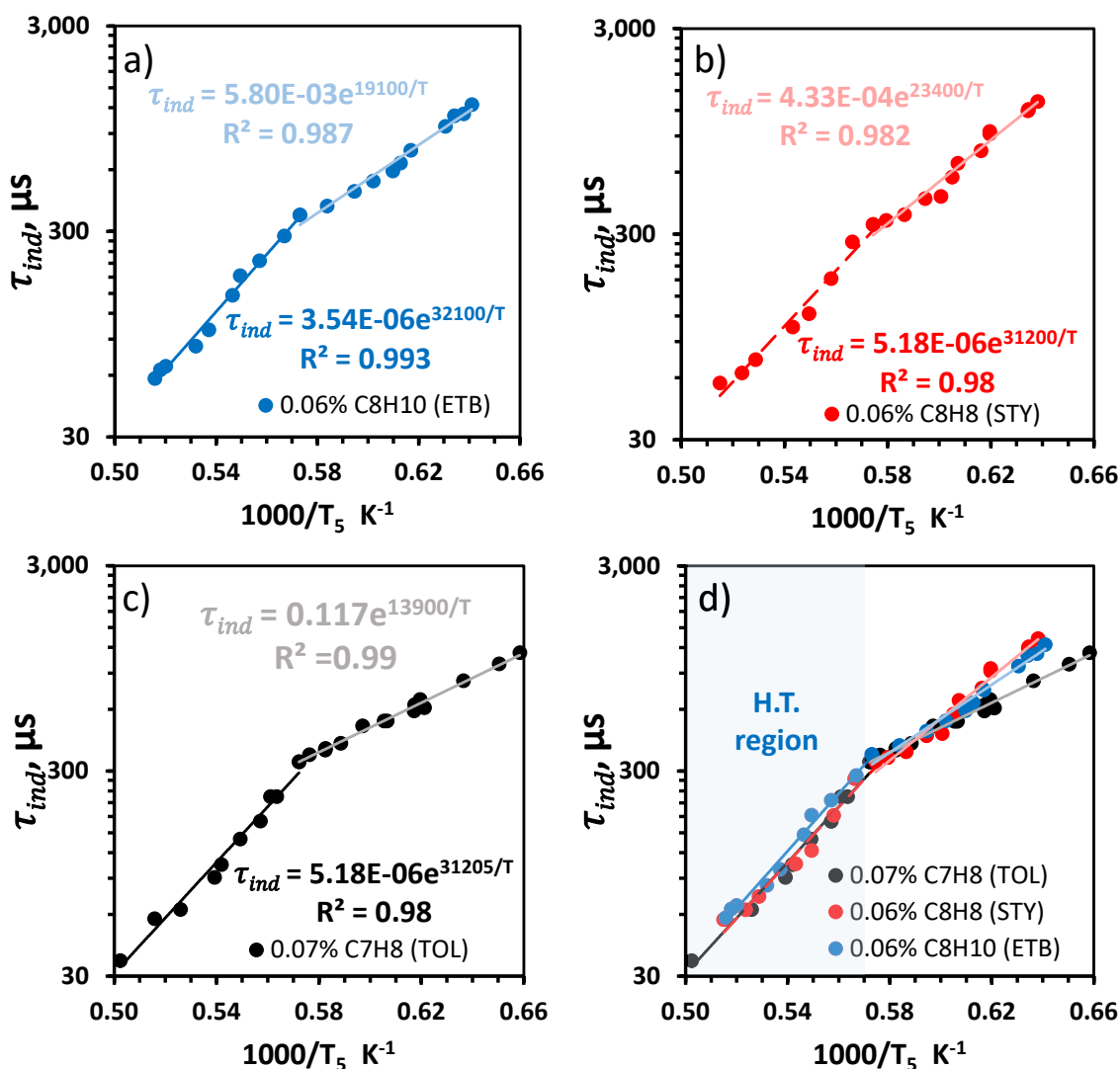
Figure 5-77. Induction delay times vs 1000/\text{temperature} ( 1000\text{-K}^{-1} ) for a) 0.0613% ethylbenzene (blue), b) 0.0613% styrene (red), c) 0.07% toluene (black; [128]), diluted in argon d) comparison between the three datasets.
