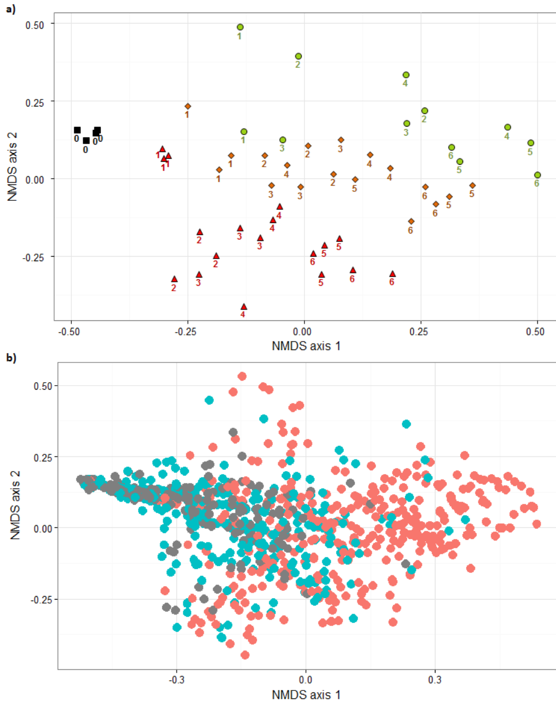
Figure 6.3-3: Ordination graph for a two-dimensional NMDS of the identified sequences based on the Bray-Curtis distance. The first plot (a) represents similarities between samples along the different cycles (number below symbols) for reactors fed with cellobiose (●), with SAC (▲), and with a mix of these two substrates (◆). The second graph (b) represents similarities between identified sequences affiliated to Firmicutes (●), Proteobacteria (●) and other taxonomic phyla (●).
