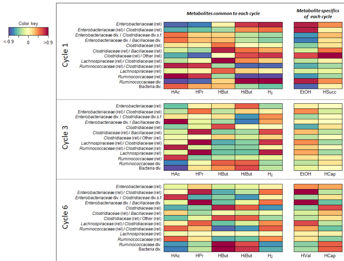
Figure 6.3-4: Regularised Canonical Correlation Analysis (rCCA) performed on calculated indicators
