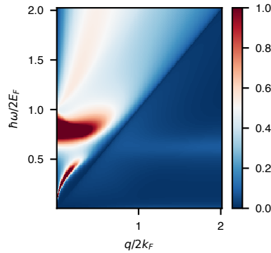
Figure 27: Loss function -\text{Im}[1/\epsilon(q, \omega)] of solvated graphene. The electronic temperature is T = 0\text{K} and Fermi energy E_F = 70\text{ meV} . We used the model of Eq. 88 for g_w(q, \omega) with d = 1.52\text{\AA} .
