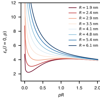
Figure 42: Static dielectric constant \epsilon_e(l = 0, p) of a CNT a T = 300 K.
