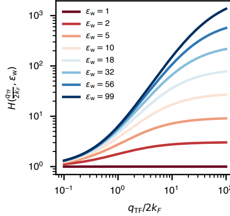
Figure 44: H(\frac{q_{\text{TF}}}{2k_F}, \varepsilon_w) computed from Eq. 380.
