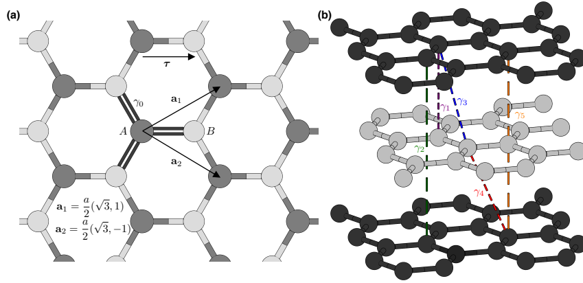
Figure 14: Tight-binding model for graphene and few-layers graphene. (a) Lattice vectors (\mathbf{a}_1, \mathbf{a}_2) of graphene with two sites (A, B) per unit cell that are linked by the vector \boldsymbol{\tau} . The chemical bonds are highlighted and defined by the vectors \boldsymbol{\tau} , \boldsymbol{\tau} - \mathbf{a}_1, \boldsymbol{\tau} - \mathbf{a}_2 . The covalent bond strength \gamma_0 = \langle \phi_{B,0} | \hat{H}_e^{(0)} | \phi_{A,0} \rangle is represented. (b) Other coupling parameters between different sites in the SWMC [70] TB model.
