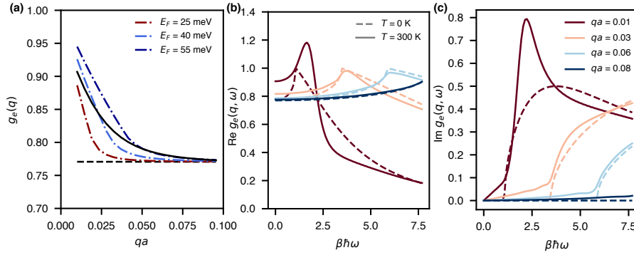
Figure 16: Surface response function (SRF) of graphene g_e(q, \omega) . (a) Static SRF g_e(q) = g_e(q, \omega = 0) of intrinsic graphene at T = 0 K (black dashed curve), at T = 300 K (black curve) and for various doping level E_F at T = 0 K (dashed dotted curve). Evolution of the (b) real and (c) imaginary part of g_e(q, \omega) with wavevector and temperature.
