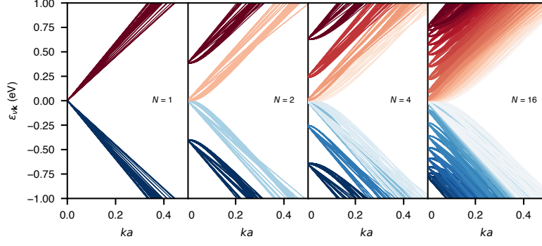
Figure 15: Evolution of the band structure near the \mathbf{K} point for FLG. The number of graphene layers N are stacked in the Bernal configuration (ABA...). For each band, we represent N_{\theta_k} = 20 angles for the same norm of k = |\mathbf{k}| .
