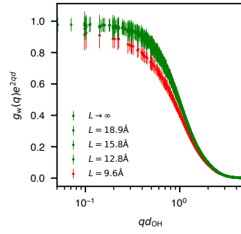
Figure 37: Static surface response function of water confined in slabs of length L . We use the Werder force field and d_{\text{Werder}} .
