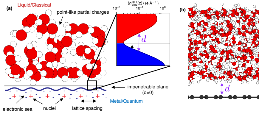
Figure 3: Schematic drawing of the metal/liquid interface. (a) From a quantum perspective, the zoom shows the electronic density near the interface between graphene and water. It is obtained with a static DFT calculation on a snapshot taken randomly at equilibrium. We fix an altitude for the impenetrable plane ( d = 0 ). (b) From a classical or practical modeling perspective, a vacuum gap d > 0 is introduced. The image is a snapshot from an interfacial MM simulation.
