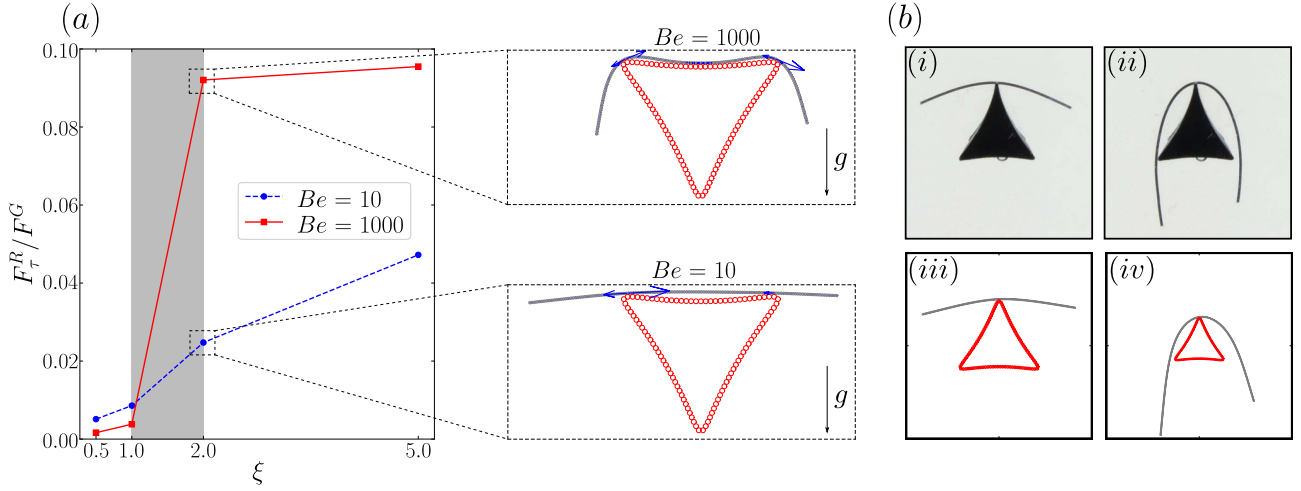
Figure 5.8: (a) Evolution of the tangential component (frictional force) of the steric force scaled by the gravitational force for two different values of Be and various values of \xi , D_x = 0.05L and \mathcal{K} = -0.6 . The close-up views show the corresponding distributions of the tangential component of the steric force along the fiber centerline, for \xi = 2 . (b) Trapping events from experimental (i – ii) and numerical (iii – iv) results obtained for \mathcal{K} = 0.6 . (i) Be = 36 and \xi = 2 . (ii) Be = 210 and \xi = 4 . (iii) Be = 10 and \xi = 2 . (iv) Be = 200 and \xi = 5 .
