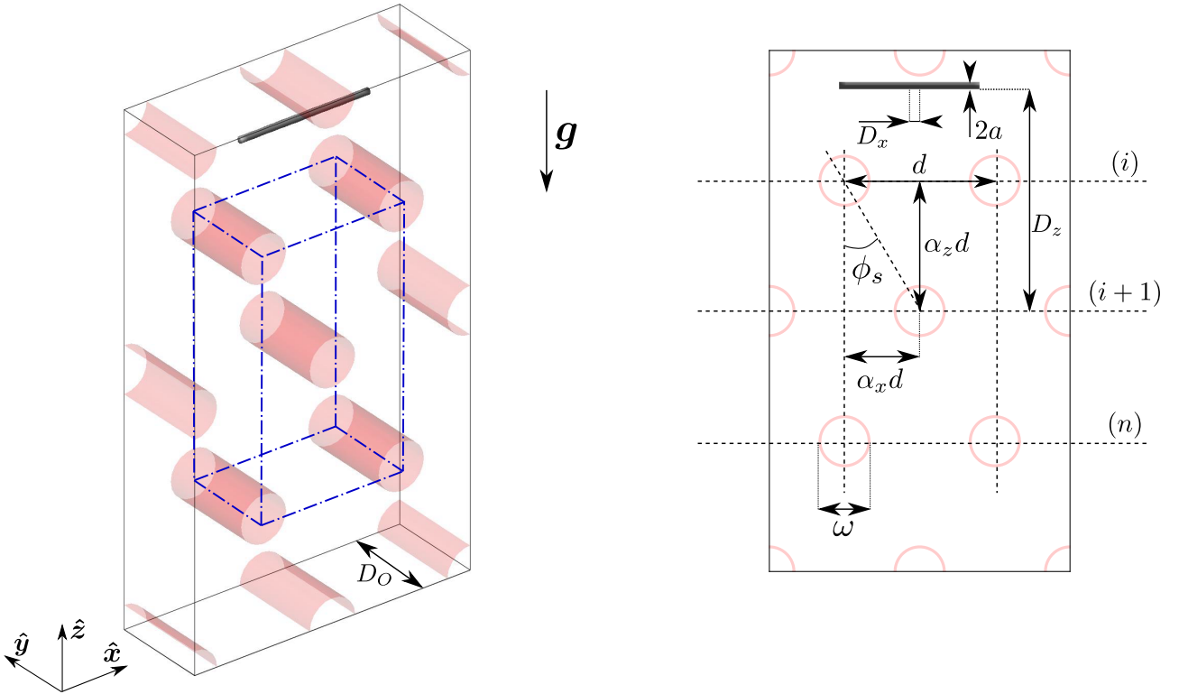
Figure 6.1: Schematic of the problem considered: A flexible fiber, initially straight, sediments under gravity in an array of rigid pillars, that is arranged in a hexagonal lattice, and immersed in a quiescent viscous fluid. Left: A 3D representation of the computational domain made of 2 \times 1 \times 2 unit cells. A unit cell (indicated in blue) contains the equivalent to two pillars of depth D_O . Right: A planar representation of the computational domain, that shows an array of pillars, whose geometry is characterized by its topological parameters \alpha_x = 1/2 and \alpha_z = \sqrt{3}/2 .
