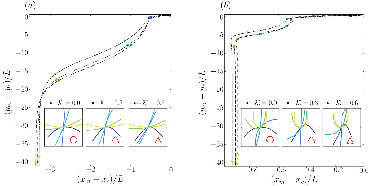
Figure 5.5: Results from numerical simulations of the trajectory of the center of mass of the fiber for \xi = 1 and three different shapes of the obstacle ( K = 0, 0.3 and 0.6 ). The snapshots show the configurations of the fiber under sedimentation in a frame moving with its midpoint, each configuration corresponds to the point having the same color on the trajectory. The initial offset of the fiber midpoint is set horizontally at D_x/L = 0.05 with respect to the center of mass of the obstacle. (a) With an intermediate value of the elasto-gravitational number Be = 100 . (b) With a large value of the elasto-gravitational number Be = 1000 . Note that x_c and y_c represent the position of the center of mass of the obstacle in xy plane. Parameter values are as in Fig. 5.4.
