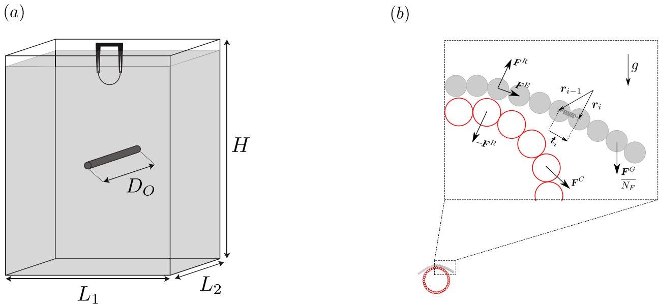
Figure 5.2: (a) Experimental setup, showing a fiber initially held with tweezers under the free-surface of the tank, with an obstacle of circular cross-section and depth D_O held at the center of the tank. (b) Numerical model, showing the fiber (gray), represented by a chain of N_F spherical beads linked elastically by Hookean springs, and an obstacle slice (red), discretized by a series of N_O beads along its contour. Both fiber and obstacle beads are subject to external and internal forces: \mathbf{F}^R is the repulsive contact barrier force between the fiber and obstacle beads, \mathbf{F}^C is the constraint force applied to obstacle beads in order to prescribe their motion, \mathbf{F}^E and \mathbf{F}^G/N_F are respectively the internal elastic and gravitational forces experienced by the fiber beads. \mathbf{t}_i = \mathbf{r}_i - \mathbf{r}_{i-1} is tangent vector to the fiber centerline at the position of bead i - 1 .
