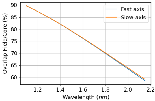
(e) Overlap of the fundamental mode and core area of the PM1550XP fiber.
