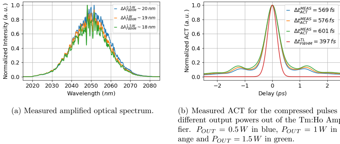
Figure 3.15: Measured optical spectrum and ACT for the compressed pulses using a CVBG pair as stretcher and compressor devices.
