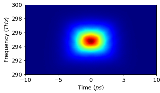
(c) Measured spectrogram. \Theta_{\lambda/2} = 0^\circ
