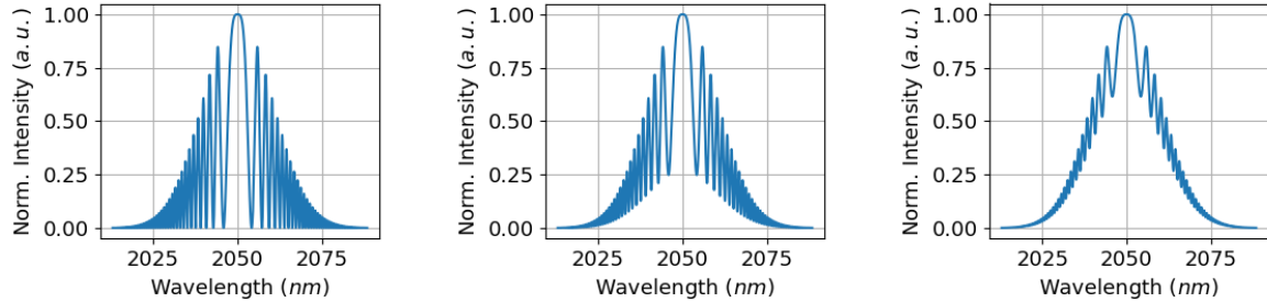
(a) Simulated spectrum of a pair of pulses with equal intensity. (b) Simulated spectrum of a pair of pulses with 10% relative intensity. (c) Simulated spectrum of a pair of pulses with 1% relative intensity.
