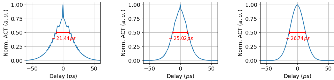
(d) Simulated ACT of a pair of pulses with equal intensity. (e) Simulated ACT of a pair of pulses with 10% relative intensity. (f) Simulated ACT of a pair of pulses with 1% relative intensity.
