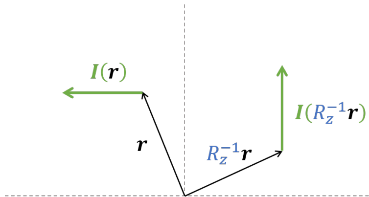
FIGURE 3.2: The current I evaluated at position r and at a -\pi/2 rotated position R_z^{-1}r .
