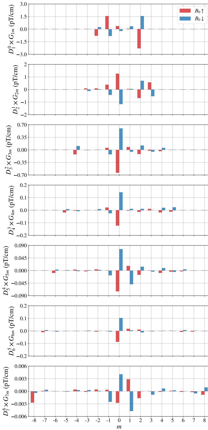
FIGURE D.1: Harmonic spectrum of the n2EDM magnetic field, for two polarities of the B_0 coil ( I = \pm 11.25 mA).
