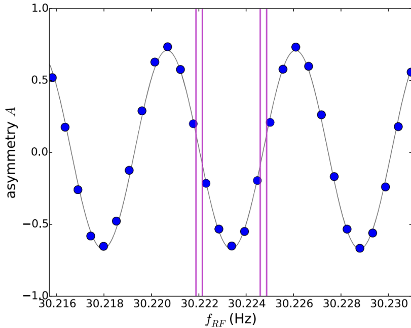
FIGURE 2.6: A set of measurements of the spin asymmetry (2.23) for different values of the transverse rotating field frequency (blue points), fitted according to equation (2.24) (black curve). The purple lines correspond to the four working points given by equation (2.26), set around the points where slope of the asymmetry, hence the sensitivity on f_n , is maximal. This result appears in the article announcing the nEDM limit (Abel et al., 2020).
