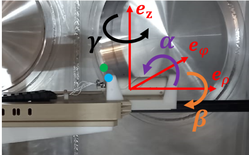
FIGURE 7.4: The purple, orange, and black arrows correspond respectively to the roll, pitch, and yaw angles of the fluxgate. The blue and green dots represent the markers 1 and 2 used for laser-tracking.
