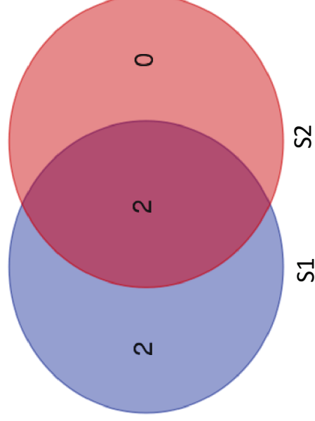
LPED: 4 QTL
