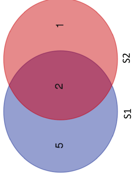
LPAN: 8 QTL
