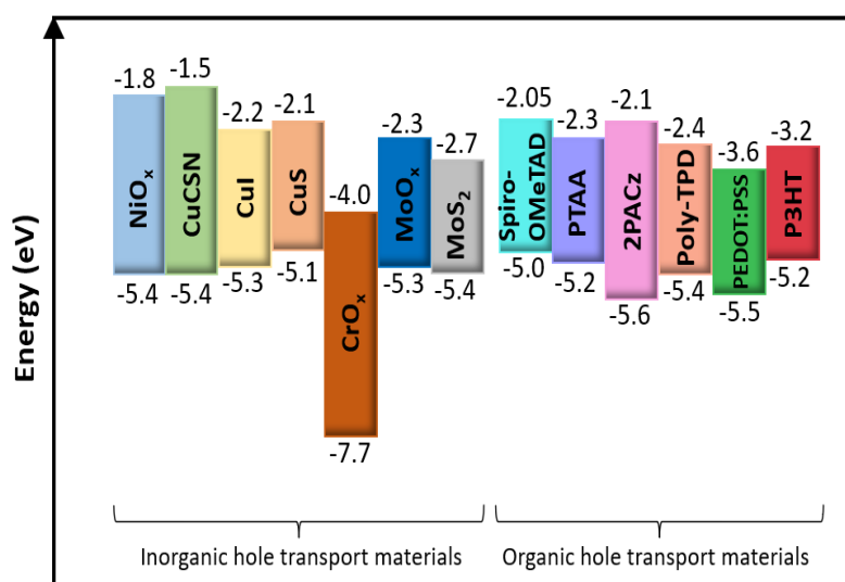
Figure I.15: VBM and CBM levels of certain hole transport materials for perovskite optoelectronics
