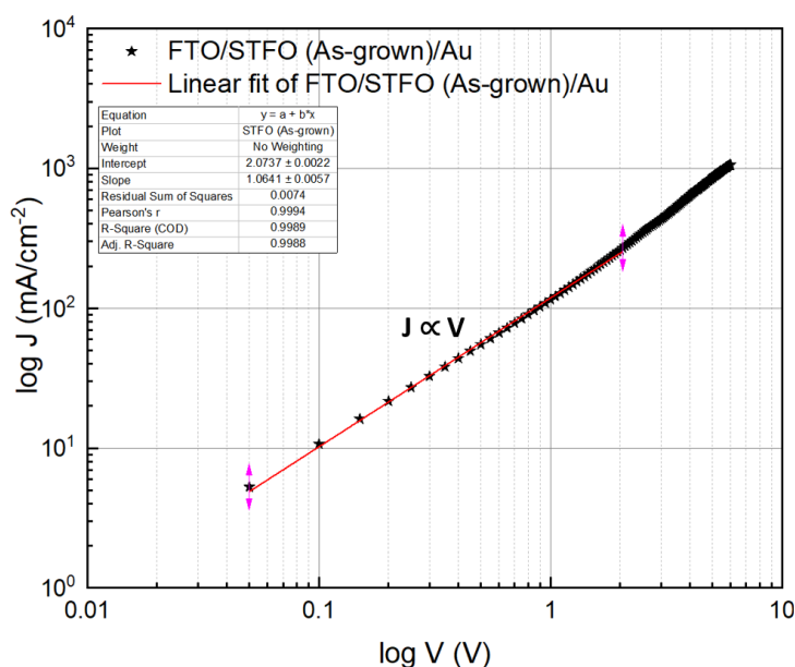
Figure III.15: Log-log scale J-V characteristics of STFO (as-grown)
